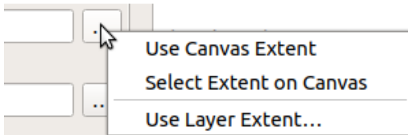
Figure 21.11: Extent selector
