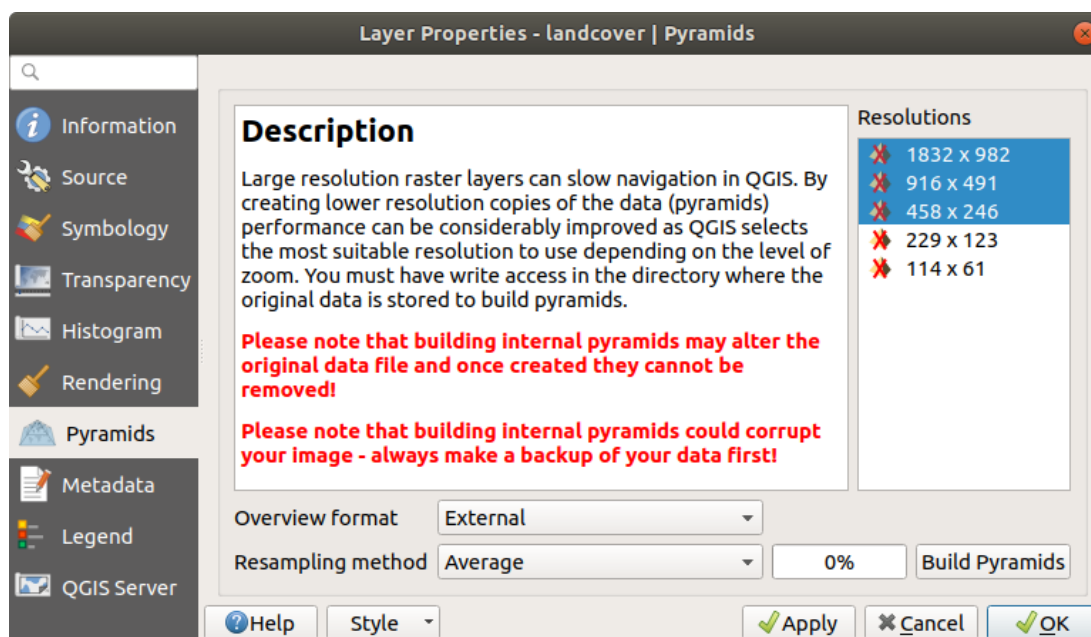
Figure 14.12: Raster Pyramids
