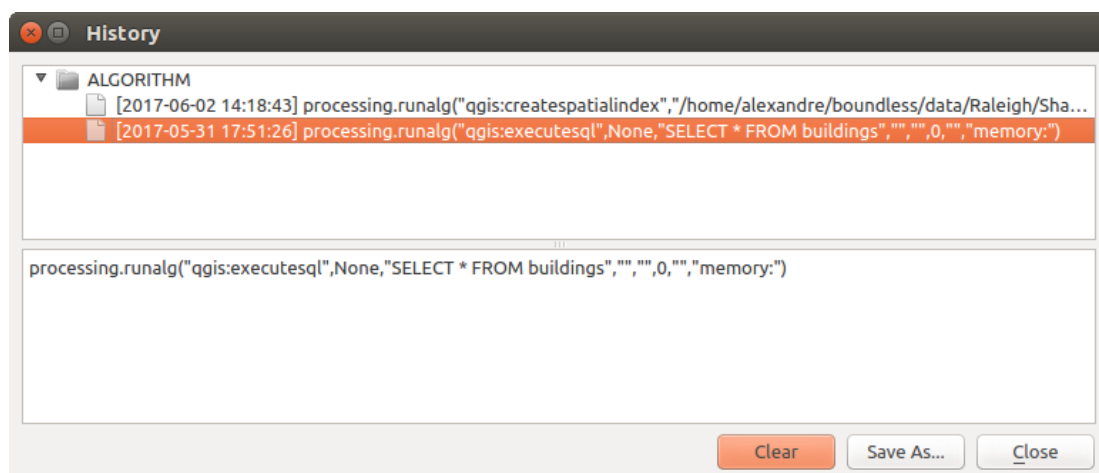
Figure 21.17: History
