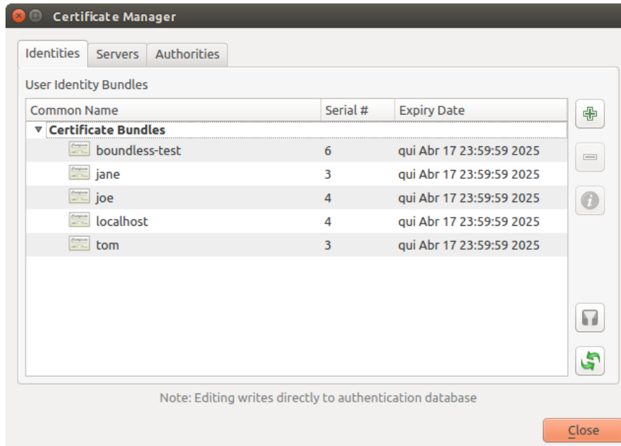
Fig. 17.29: Identities editor
