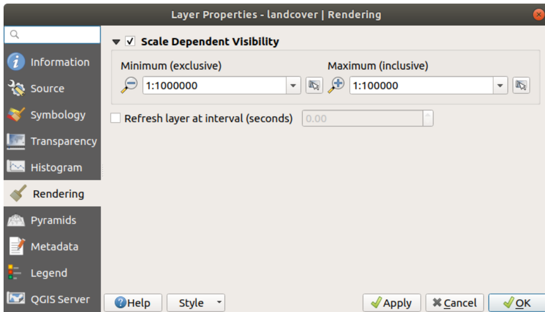
Fig. 13.11: Raster Rendering
