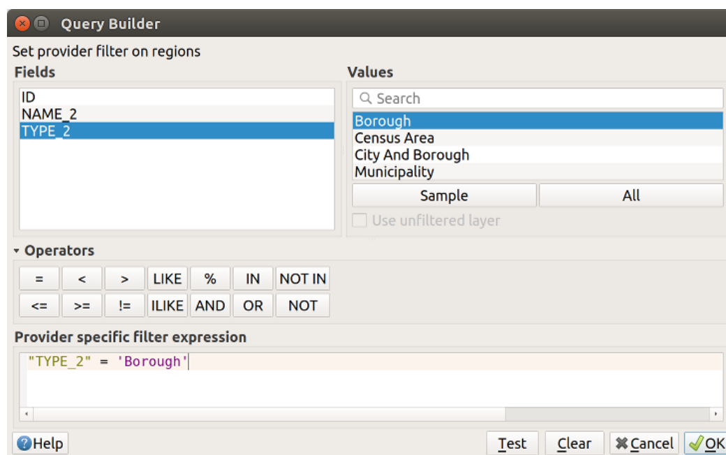
Fig. 12.9: Query Builder
