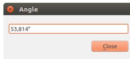
Fig. 10.16: Measure Angle
