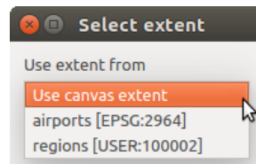
Fig. 19.12: Extent List
