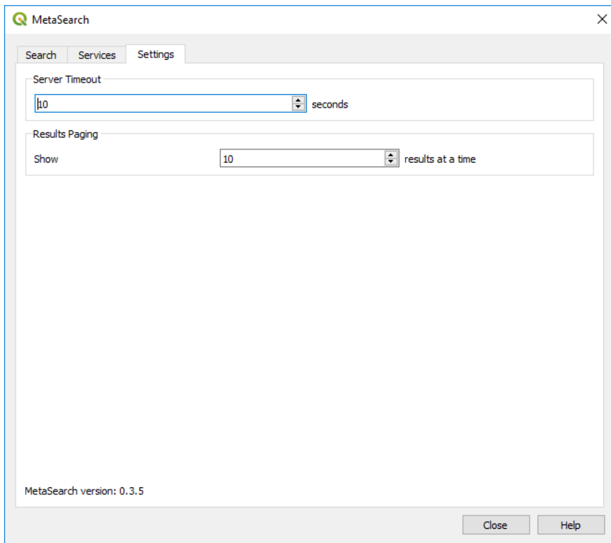
Fig. 20.28: MetaSearch settings
