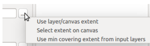
Fig. 19.11: Extent selector
