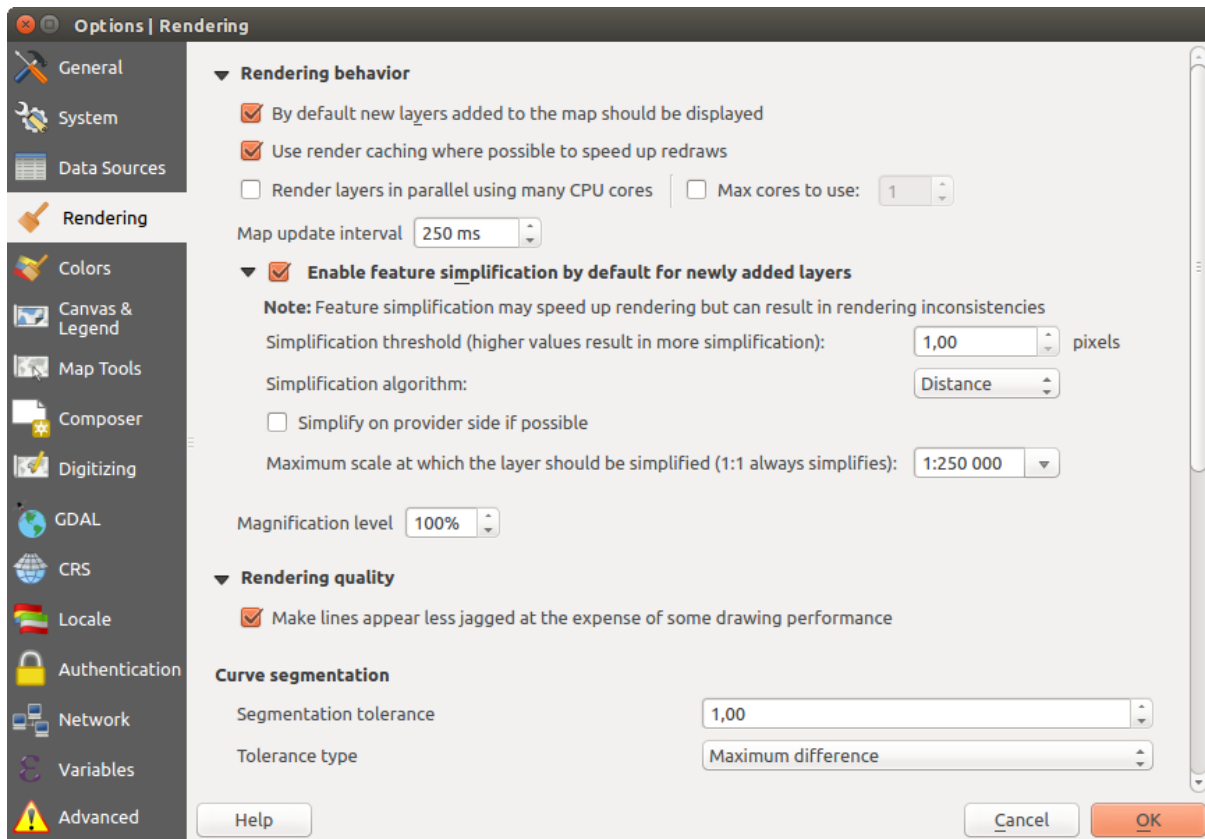
Fig. 8.4: Rendering tab of Project Properties dialog
