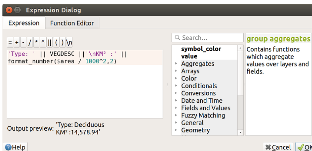
Fig. 12.39: Using expressions for labeling
