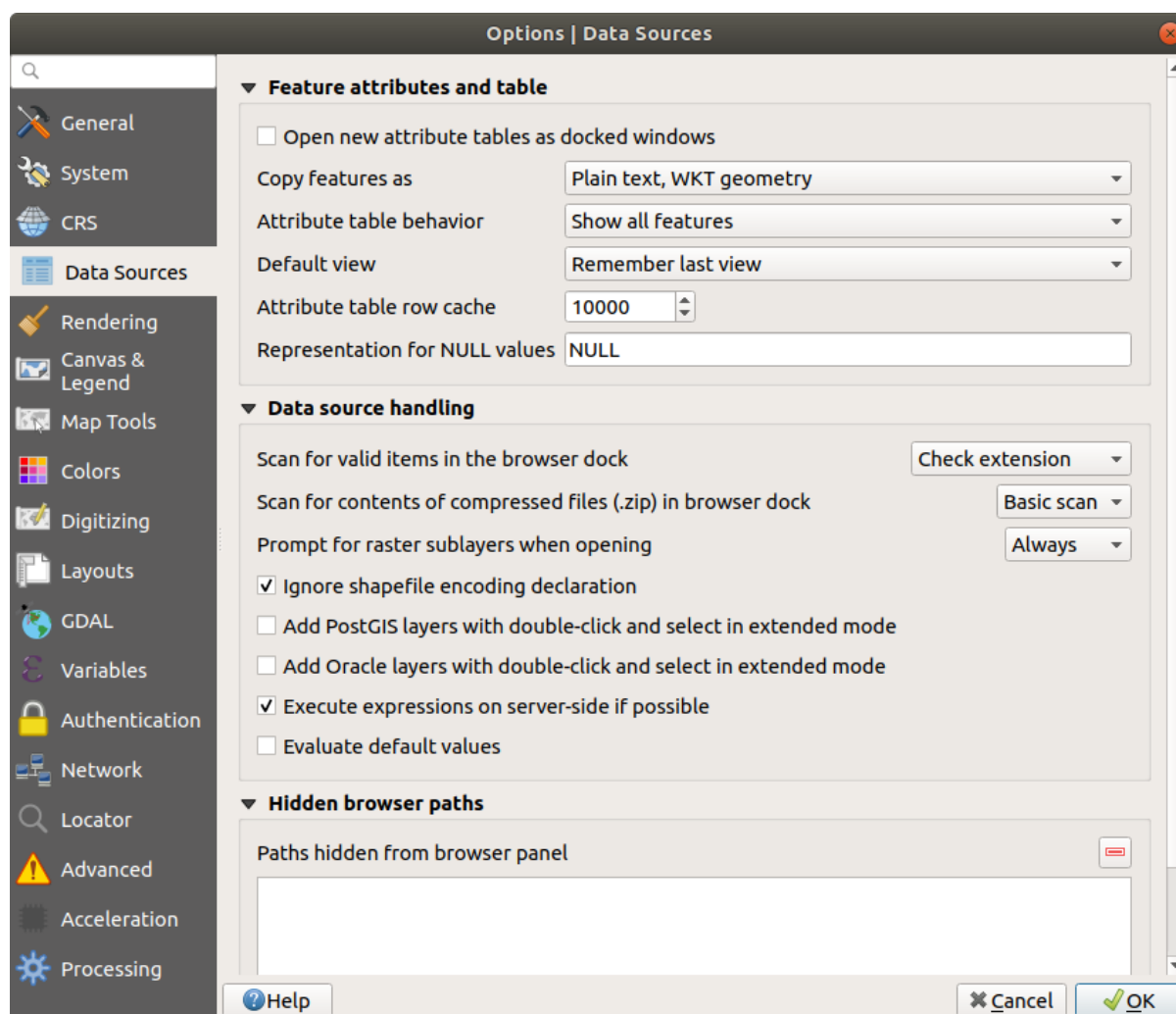
Fig. 8.3: Data Sources Settings in QGIS
