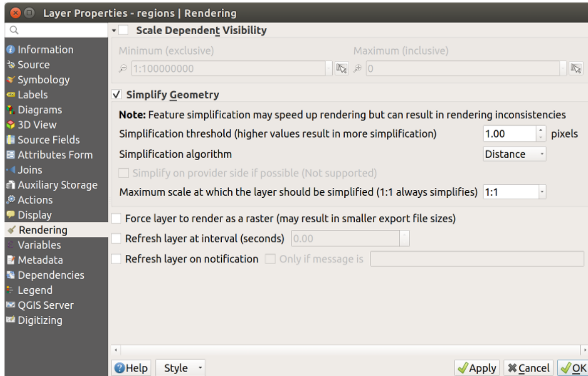
Fig. 12.69: Layer Geometry Simplification dialog
