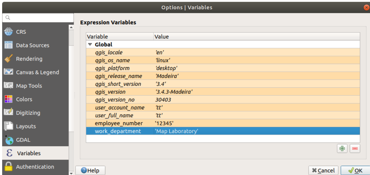
Fig. 8.11: Variables Settings in QGIS
