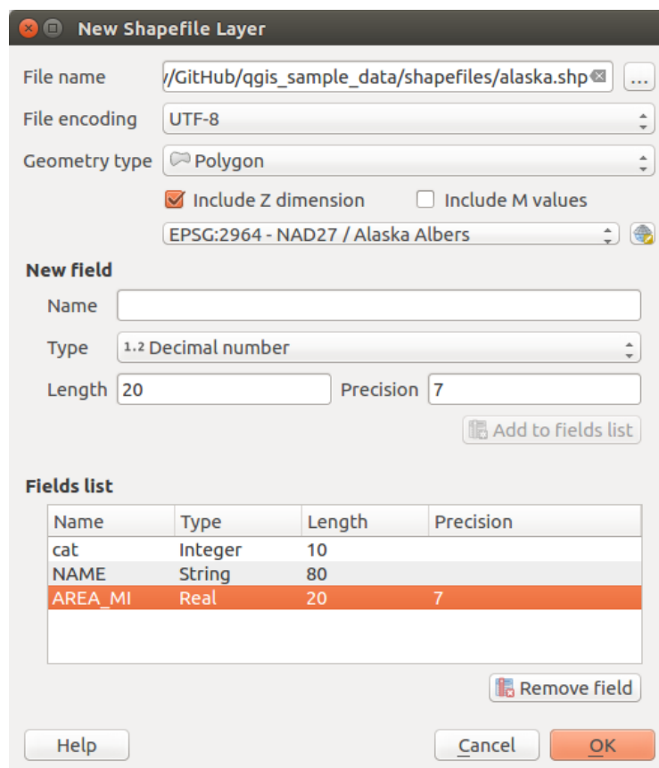
Fig. 11.12: Creating a new Shapefile layer dialog
