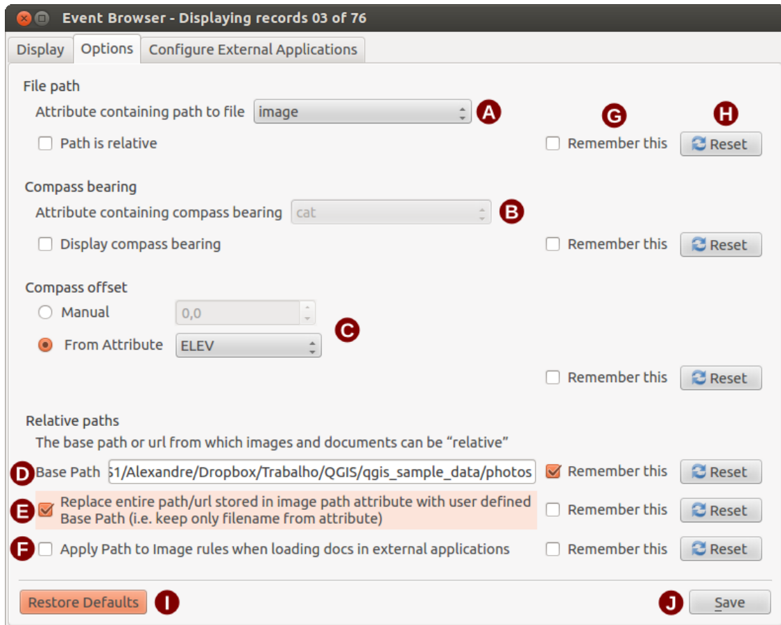
Fig. 20.14: The eVis Options window
