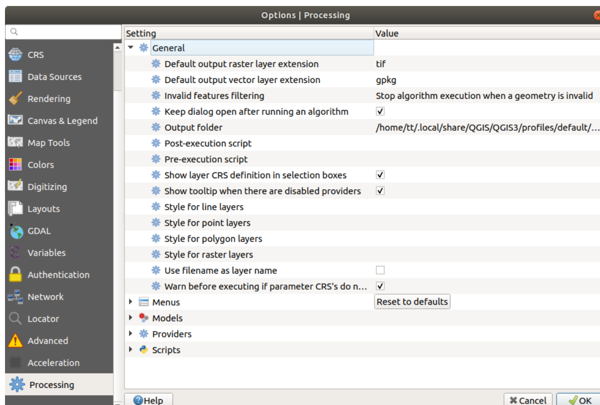
Fig. 8.16: Processing Settings tab in QGIS
