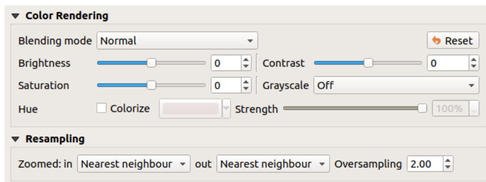
Fig. 13.8: Raster Symbology - Color rendering and Resampling settings
