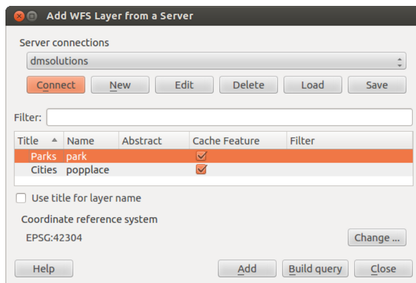
Fig. 15.4: Adding a WFS layer
