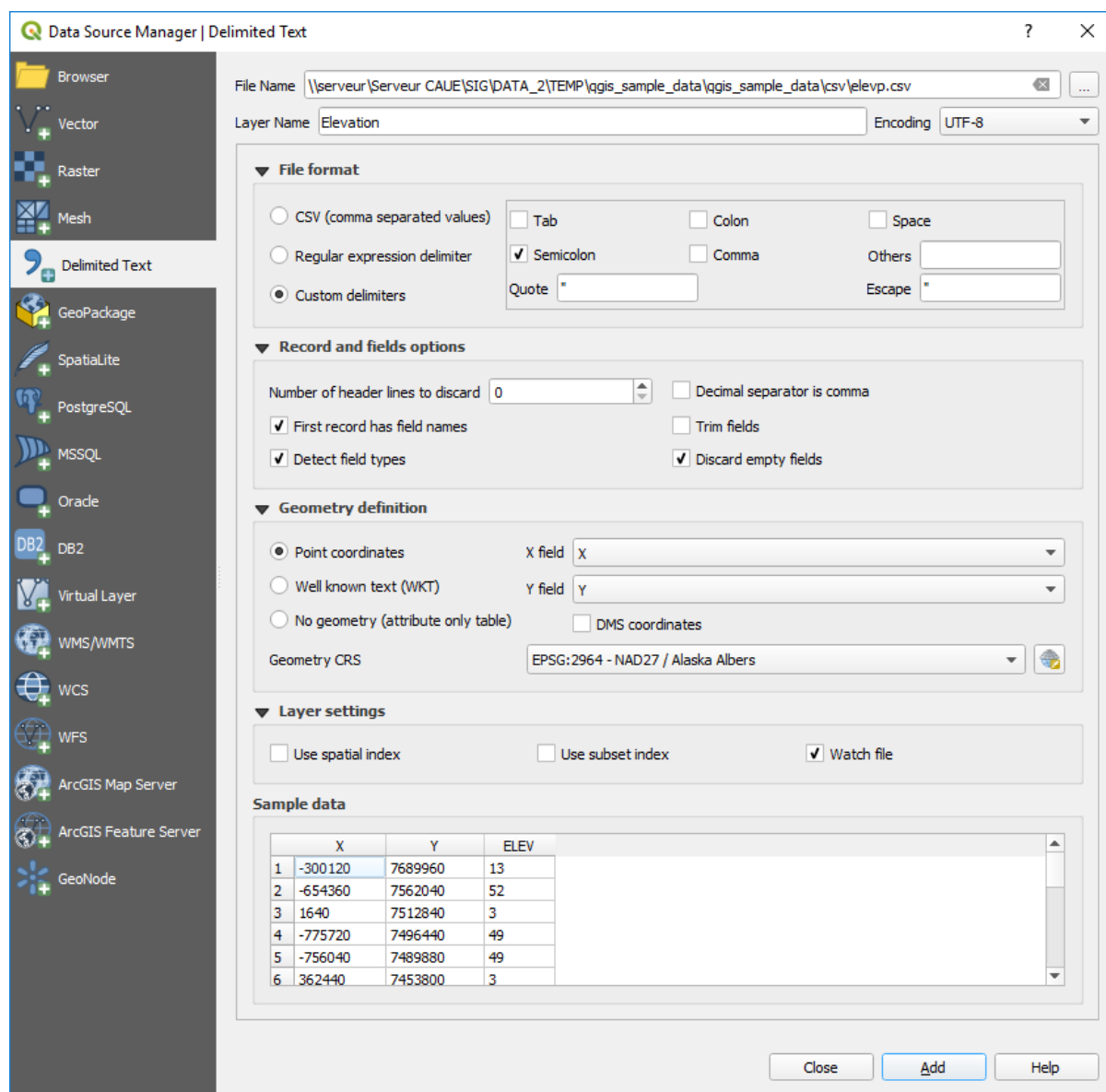
Fig. 11.7: Delimited Text Dialog
