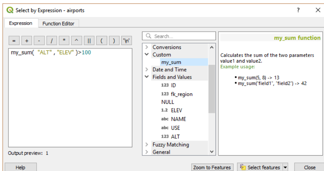
Fig. 12.75: Custom Function added to the Expression tab
