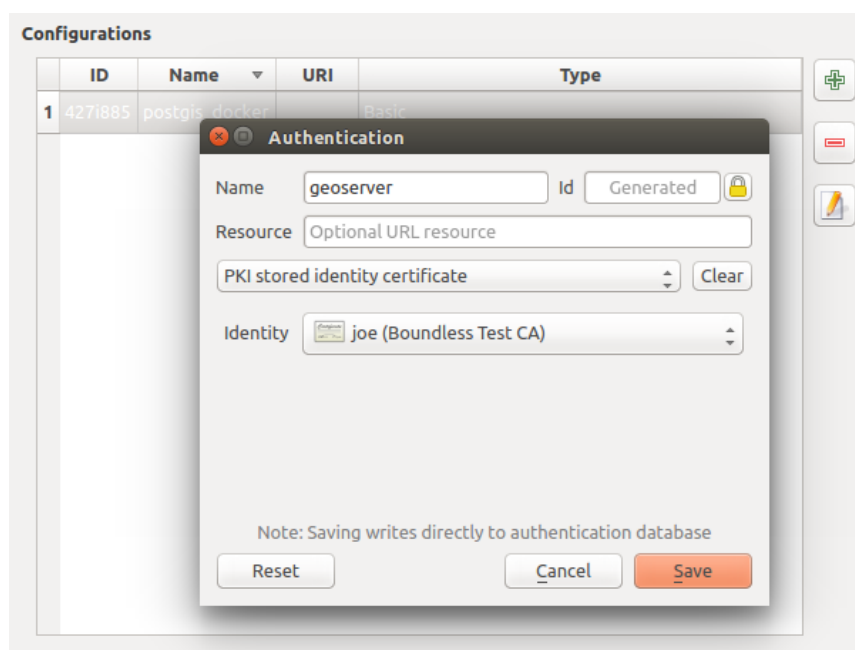
Fig. 17.6: Adding config from within Configuration editor
