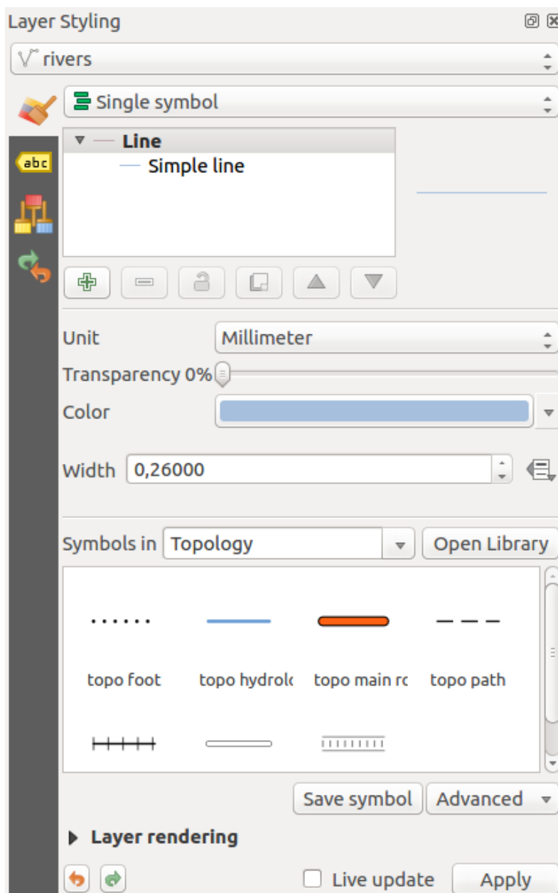
Fig. 10.2: Defining a layer’s symbology from the layer styling panel
