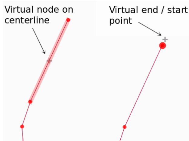
Fig. 12.91: Virtual nodes for adding vertices
