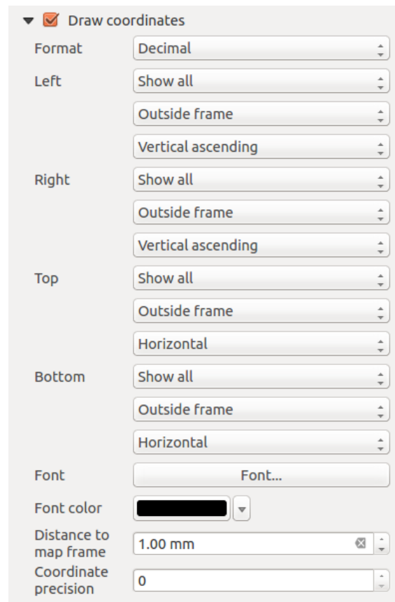
Fig. 14.19: Grid Draw Coordinates dialog
