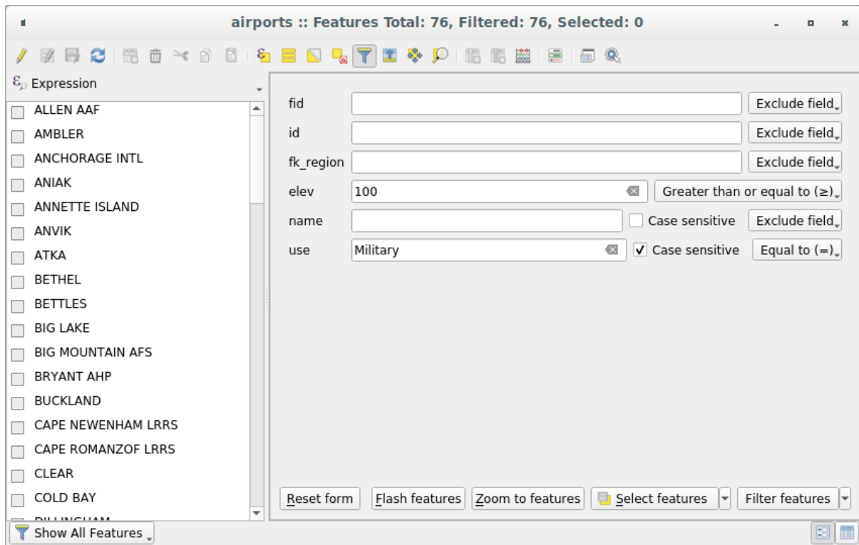
Fig. 12.79: Attribute table filtered by the filter form
