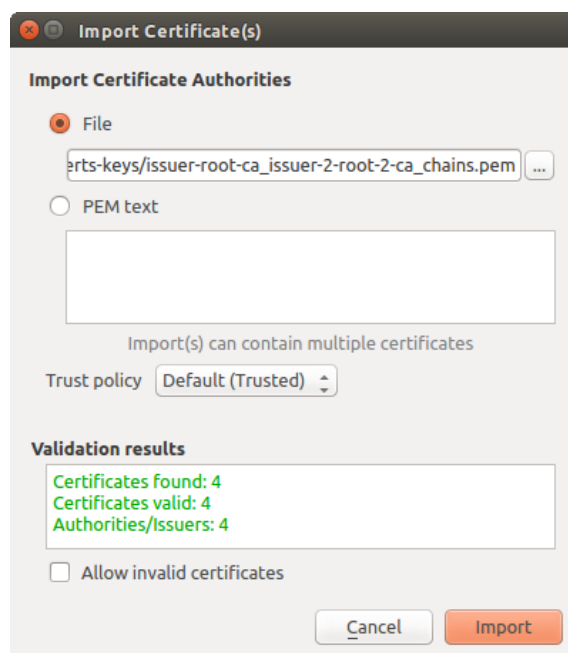
Fig. 17.28: Import certificates dialog
