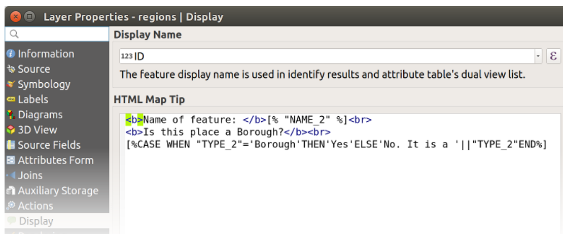
Fig. 12.67: HTML code for map tip
