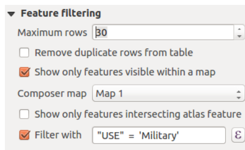
Fig. 14.37: Attribute table Feature filtering Group
