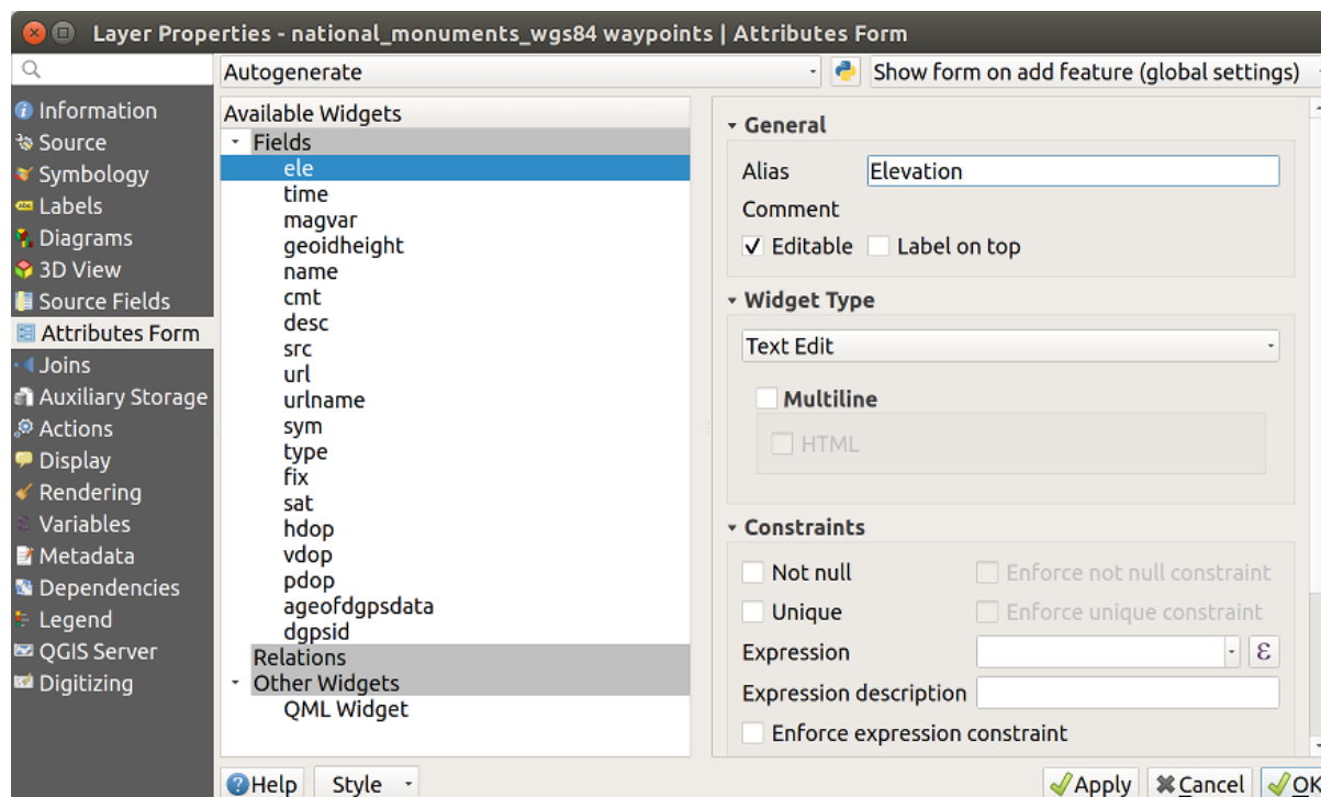
Fig. 12.52: Dialog to select an edit widget for an attribute column
