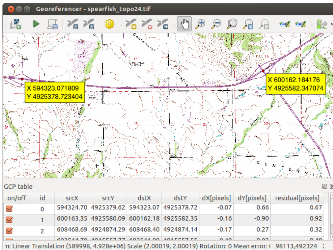
Fig. 20.21: Georeferencer Plugin Dialog
