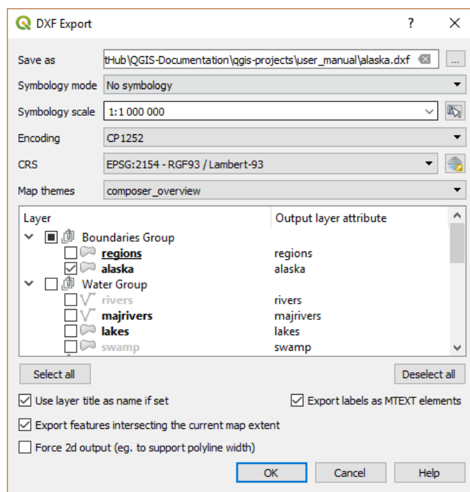
Fig. 11.17: Exporting a project to DXF dialog
