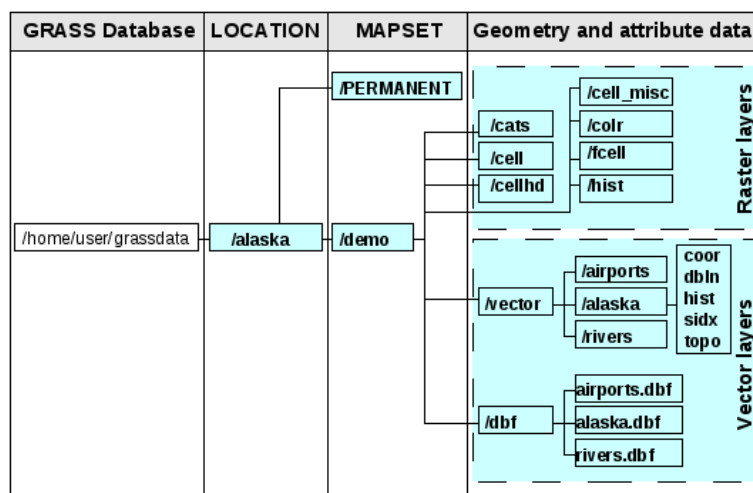
Fig. 18.1: GRASS data in the alaska LOCATION
