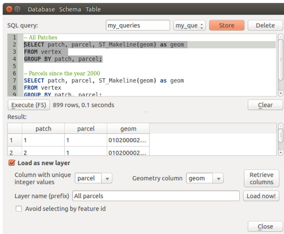
Fig. 20.12: Executing SQL queries in the DB Manager SQL window
