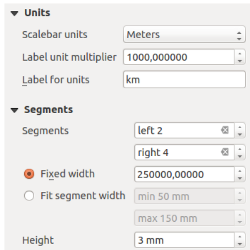
Fig. 14.29: Scale Bar Units and Segments groups
