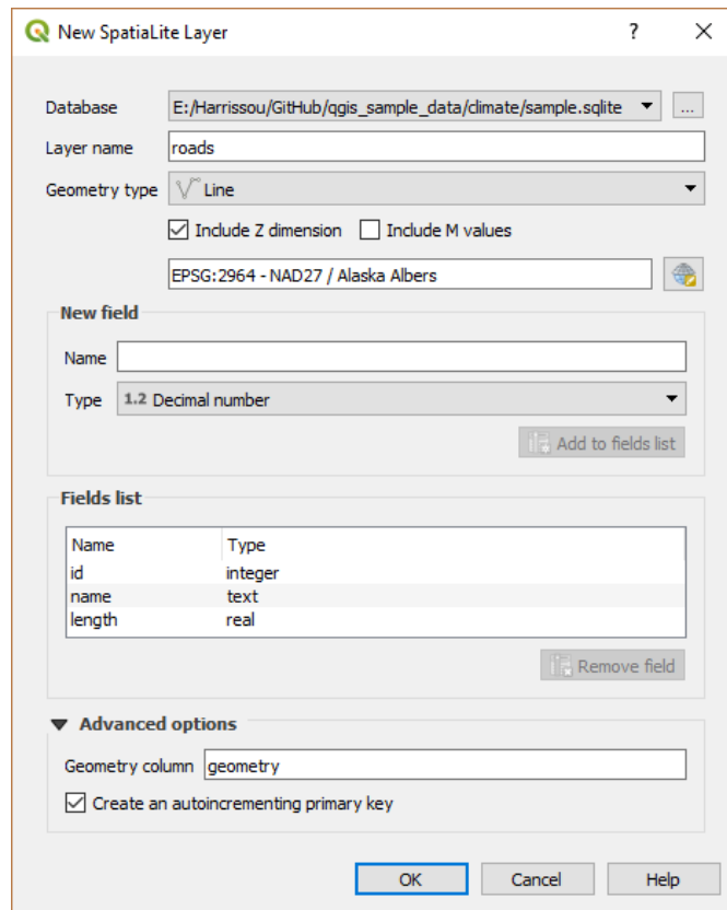
Fig. 11.13: Creating a New SpatialLite layer dialog
