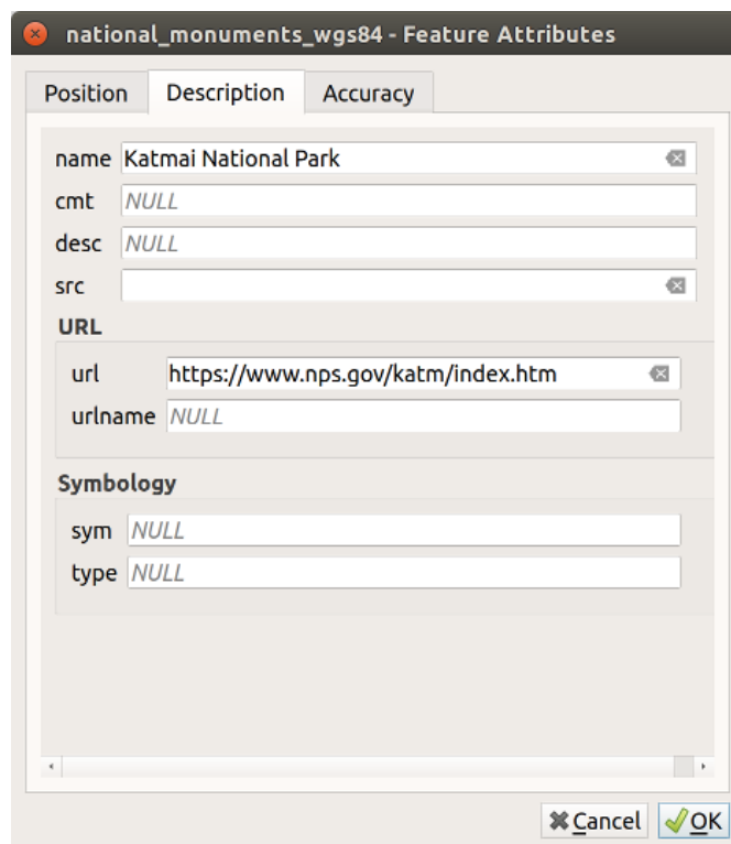
Fig. 12.50: Resulting built-in form with tabs and named groups
