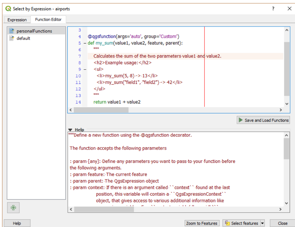
Fig. 12.74: The Function Editor tab
