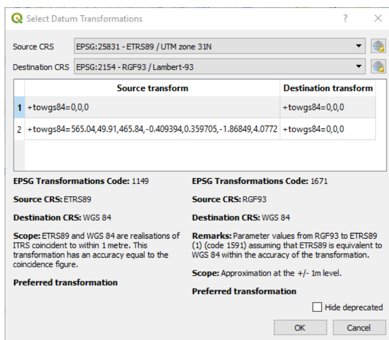
Fig. 9.4: Selecting a preferred default datum transformation
