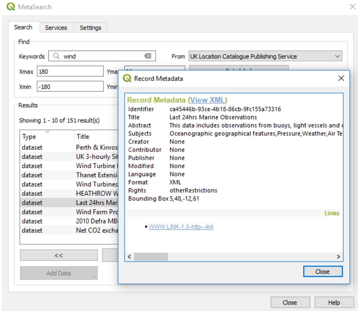
Fig. 20.27: Metadata record display
