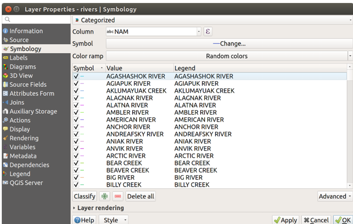
Fig. 12.11: Categorized Symbolizing options
