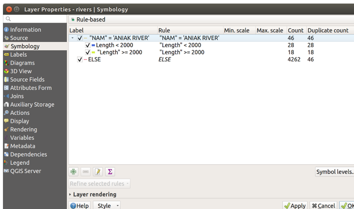
Fig. 12.15: Rule-based Symbolizing options
