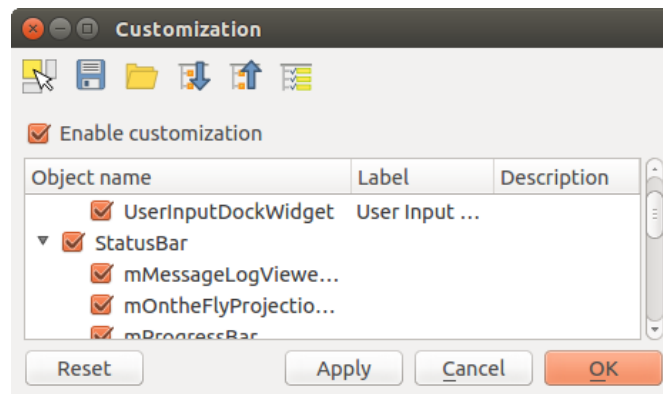
Fig. 8.20: The Customization dialog
