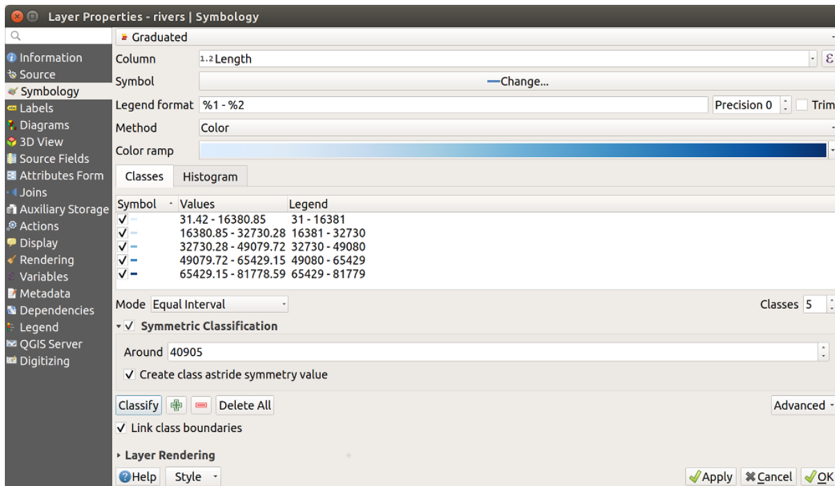
Fig. 12.12: Graduated Symbolizing options
