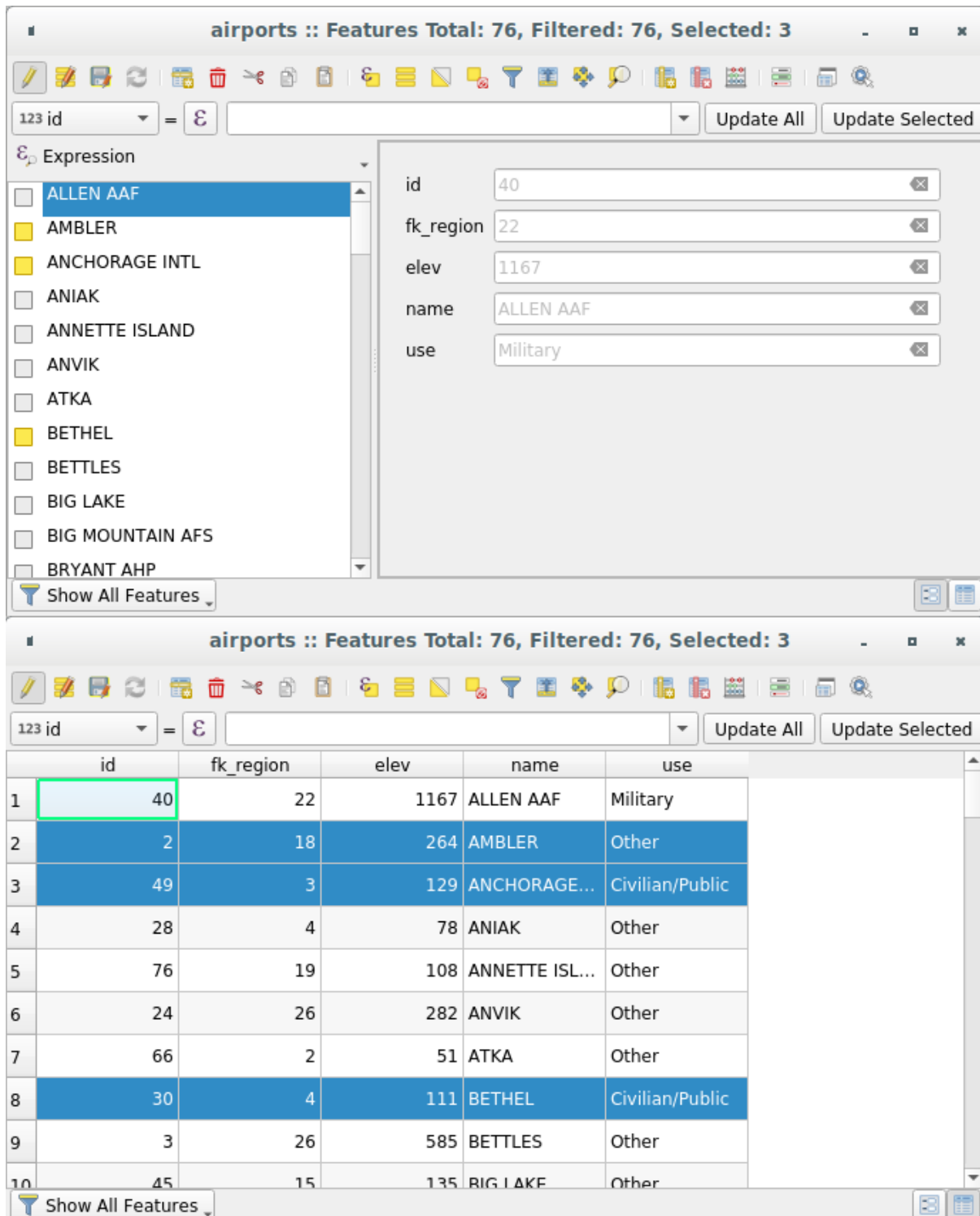
Fig. 12.77: Attribute table in form view (top) vs table view (bottom)
