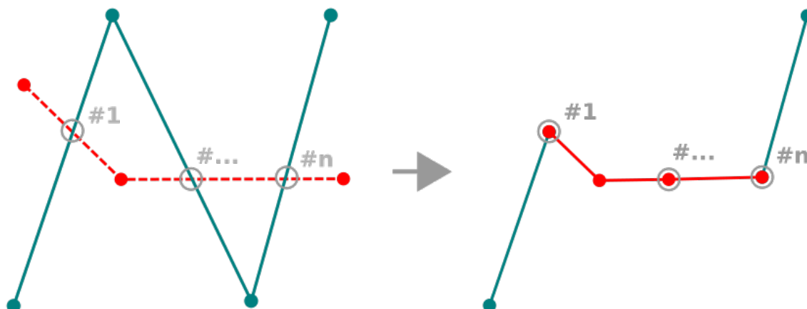
Fig. 12.95: Reshape line
