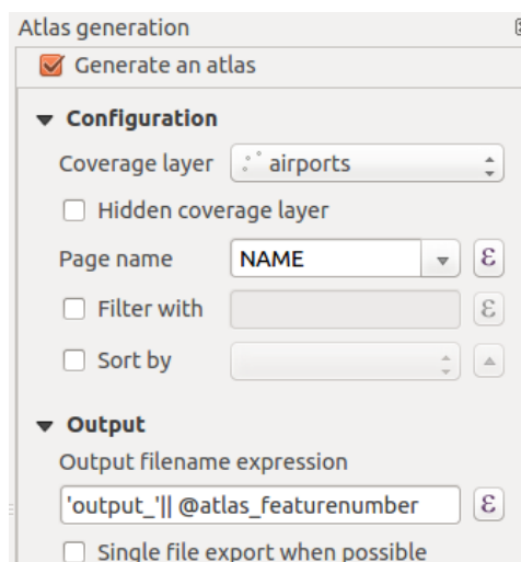
Fig. 14.56: Atlas Panel
