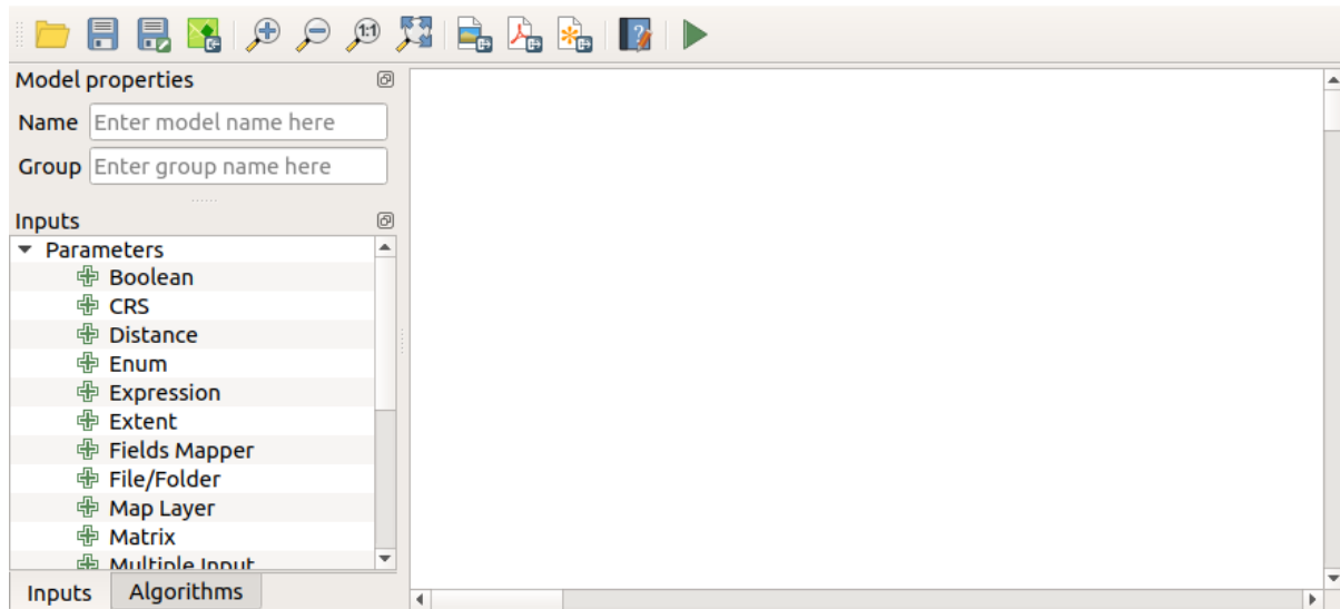
Fig. 19.17: Modeler
