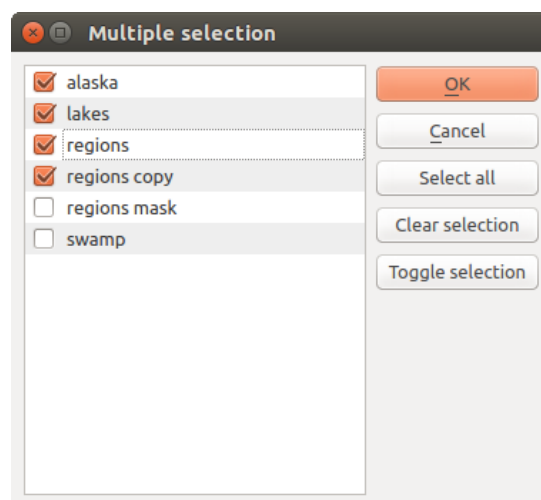
Fig. 19.14: Multiple Selection
