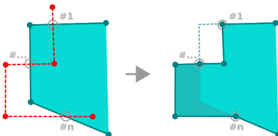
Fig. 12.96: Reshape polygon
