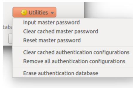
Fig. 17.15: Utilities menu
