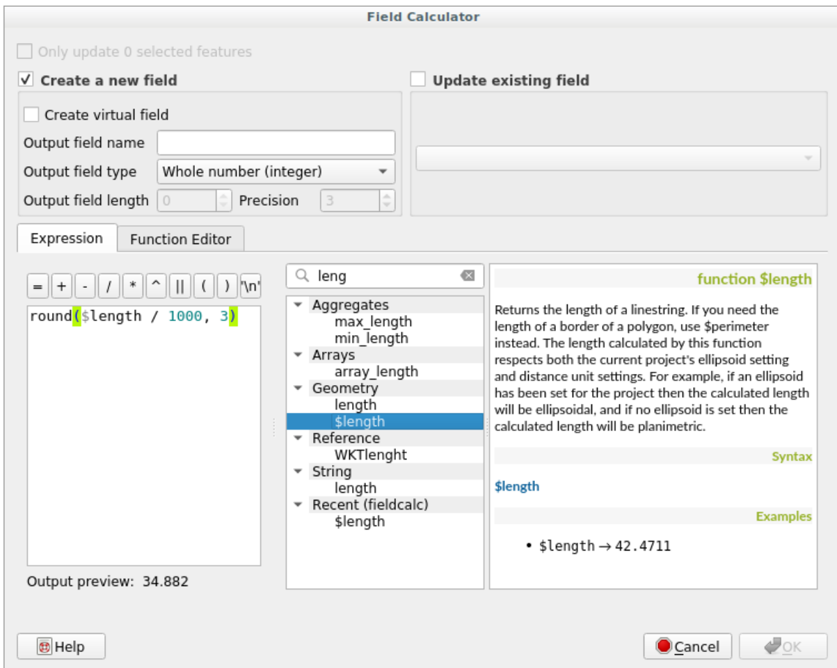
Fig. 12.81: Field Calculator
