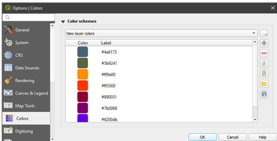
Fig. 8.7: Colors Settings
