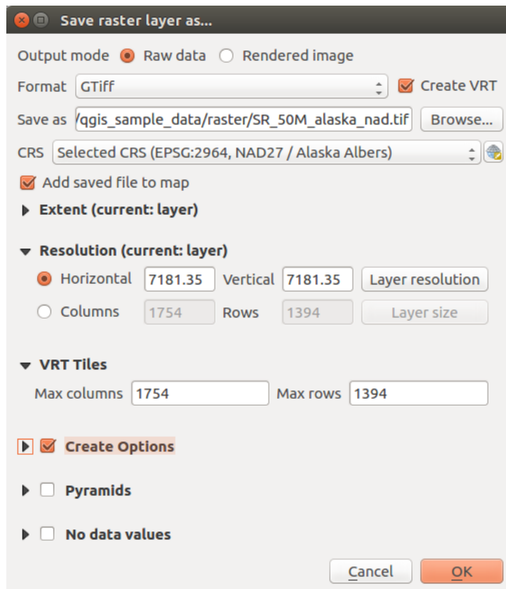
Fig. 11.15: Saving as a new raster layer
