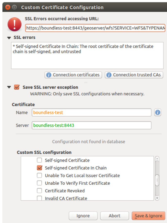
Fig. 17.37: Adding configuration during SSL error
