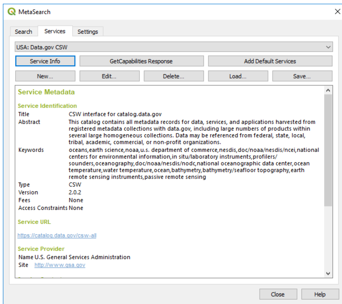
Fig. 20.25: Managing Catalog Services
