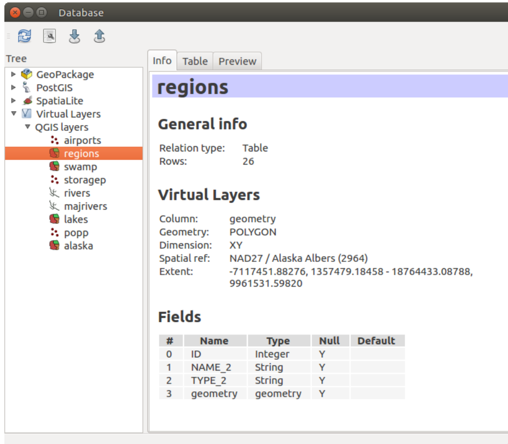
Fig. 11.3: DB Manager dialog
