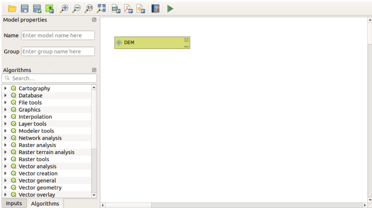
Fig. 19.20: Model Inputs
