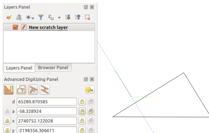
Fig. 12.102: Perpendicular digitizing
