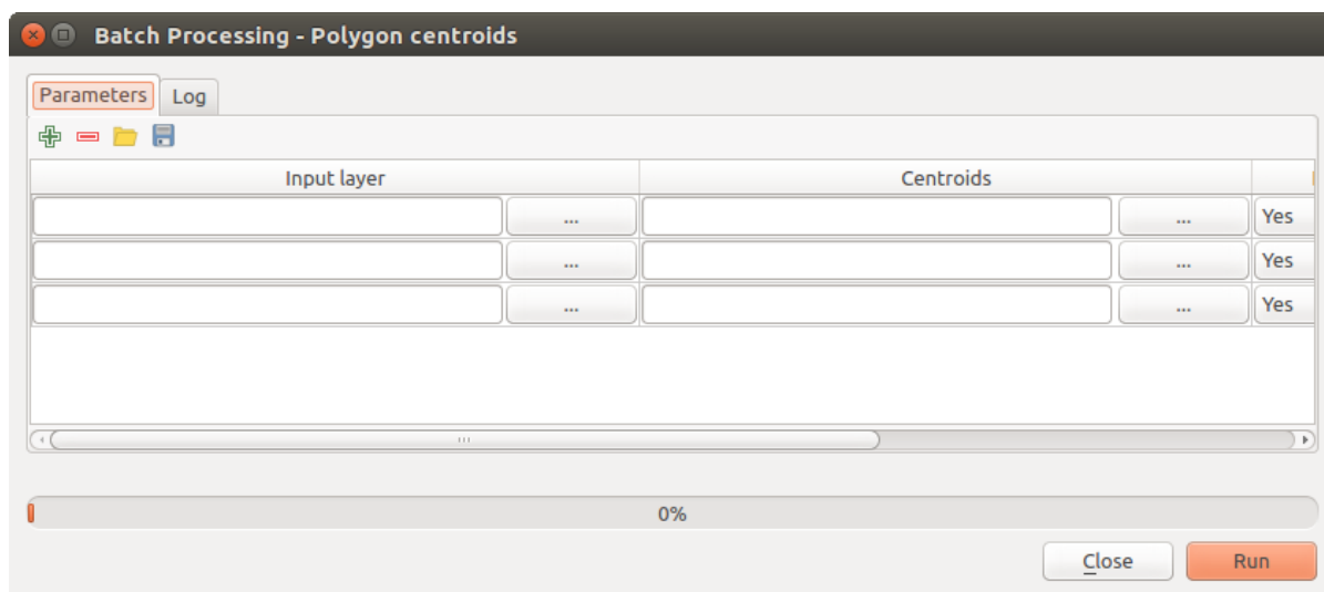
Fig. 19.28: Batch Processing
