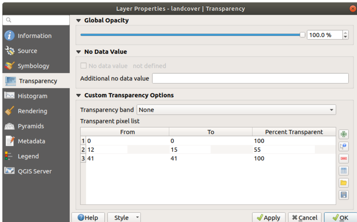
Fig. 13.9: Raster Transparency
