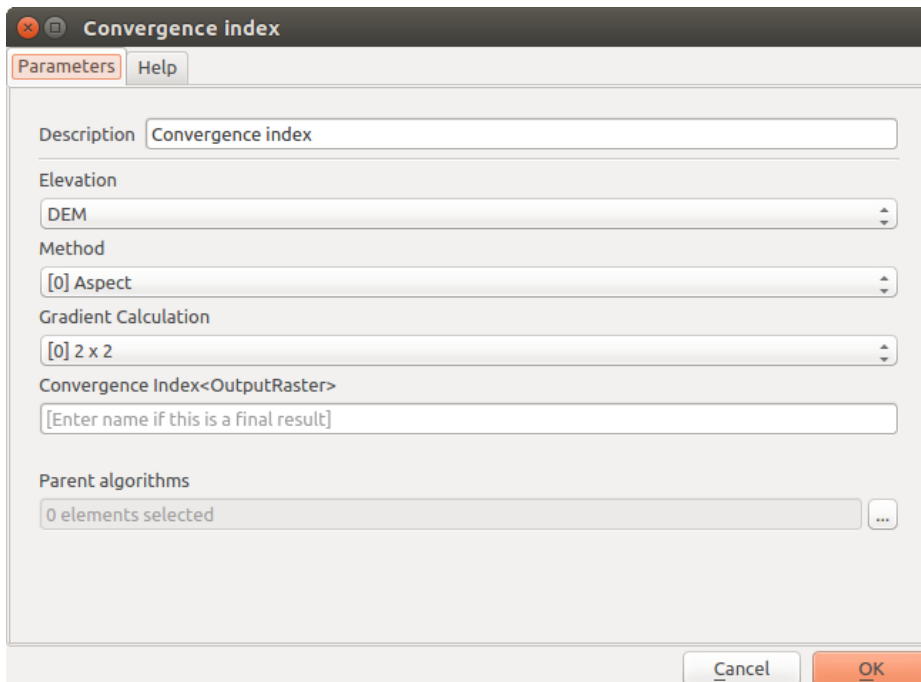
Fig. 19.21: Model Algorithm parameters
