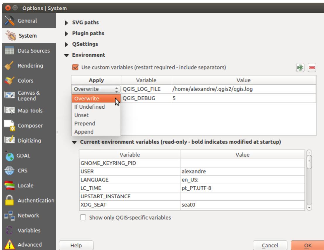
Fig. 8.1: System environment variables in QGIS
