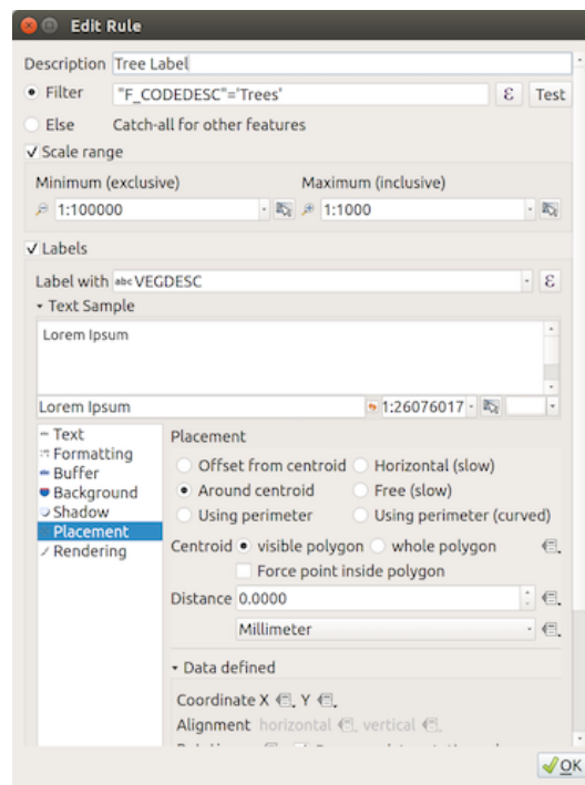
Fig. 12.37: Rule settings
