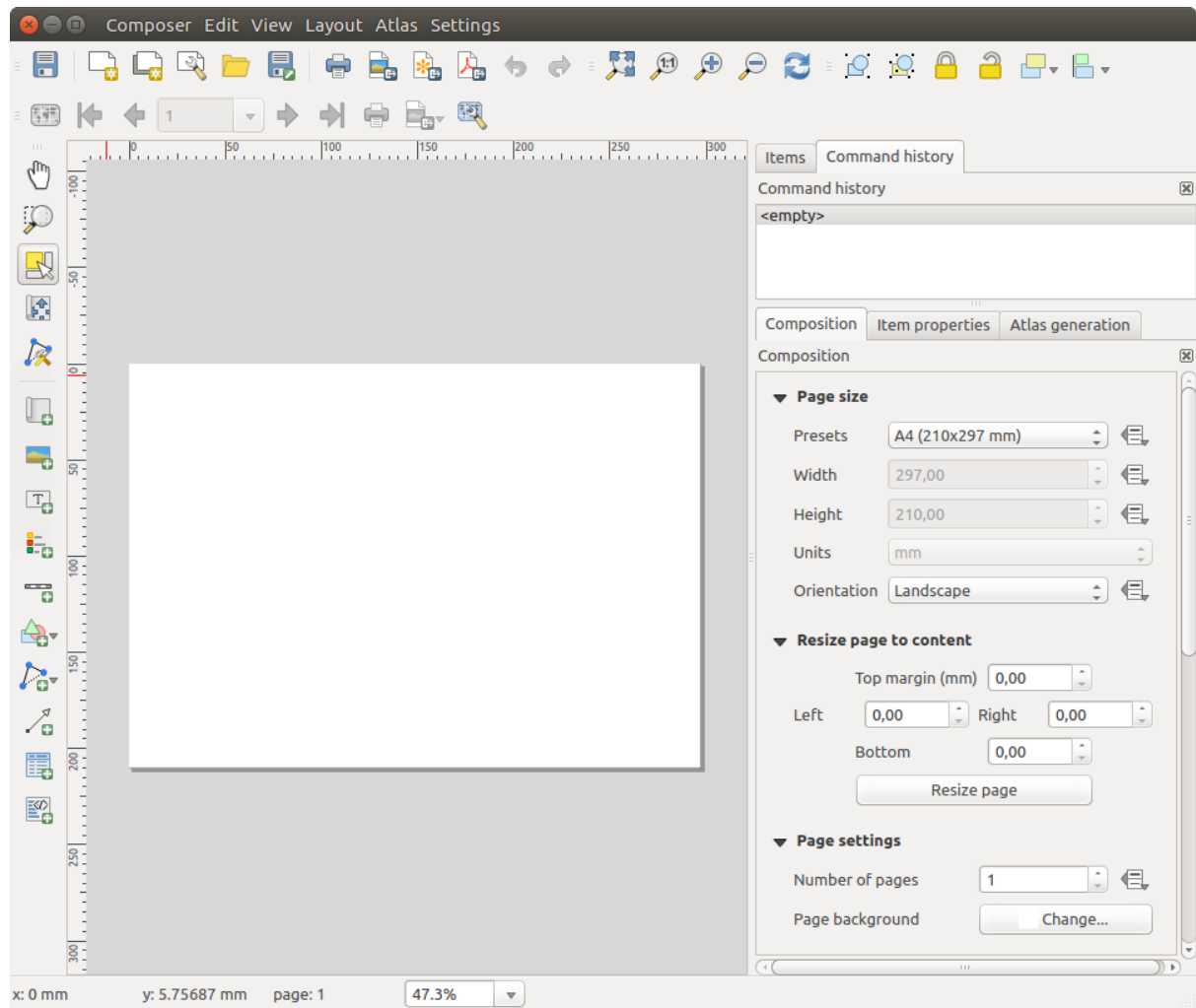
Fig. 14.2: Print Layout
