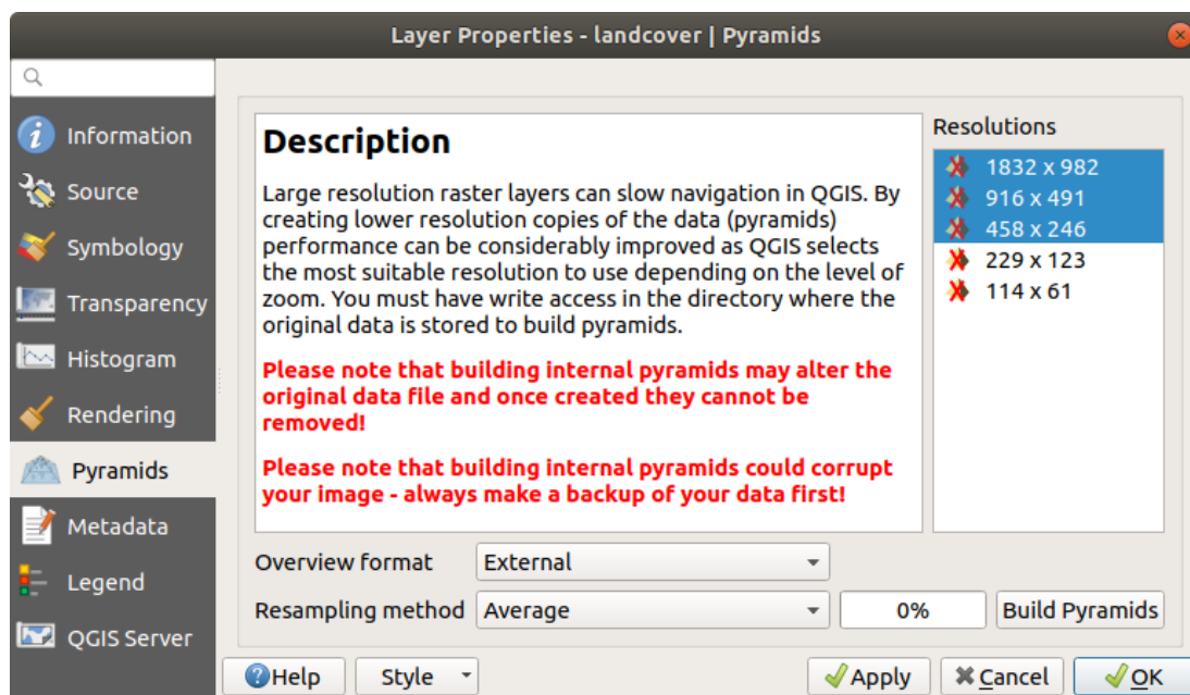
Fig. 13.12: Raster Pyramids
