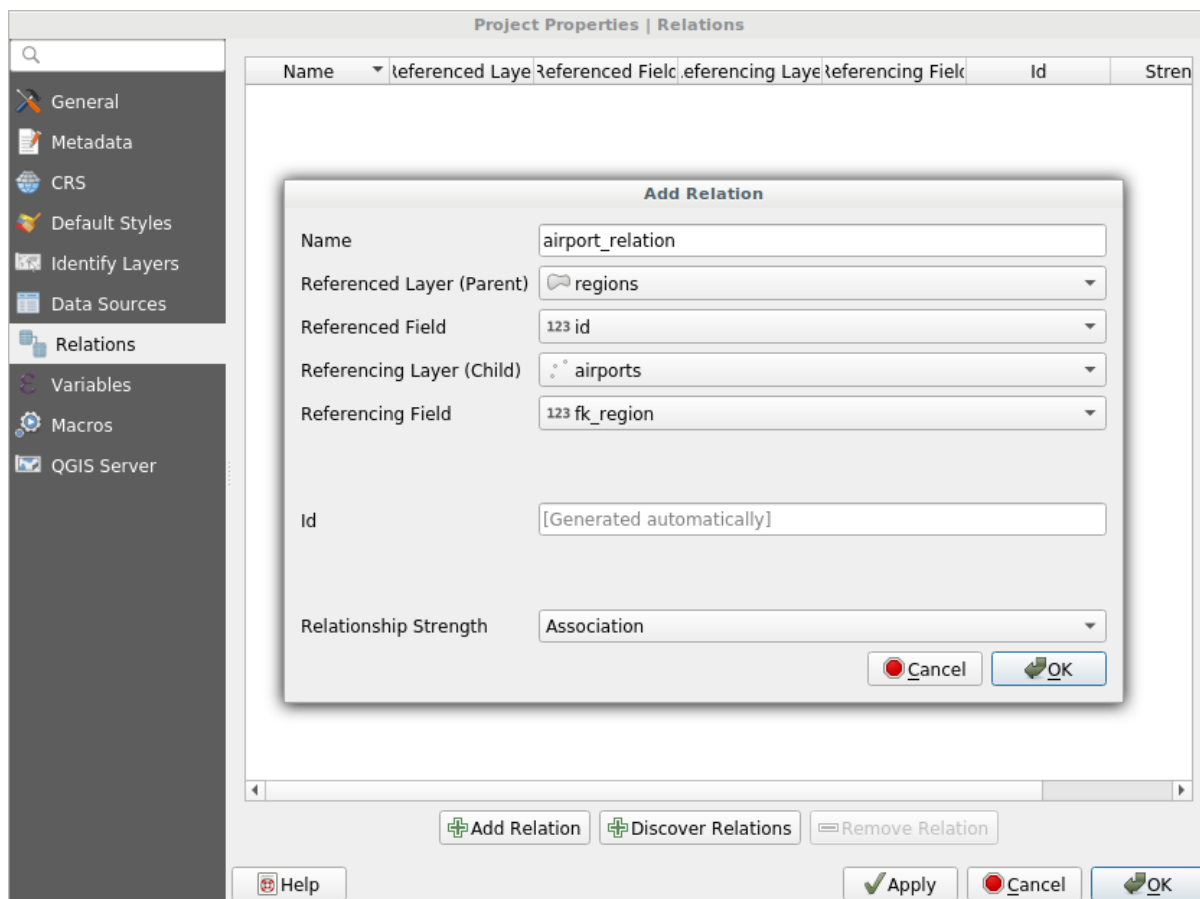
Fig. 12.85: Relation Manager
