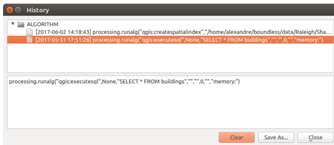
Fig. 19.16: History
