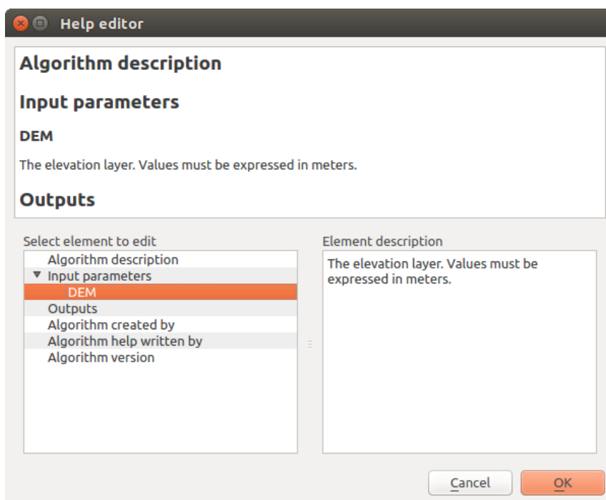
Fig. 19.25: Help Edition
