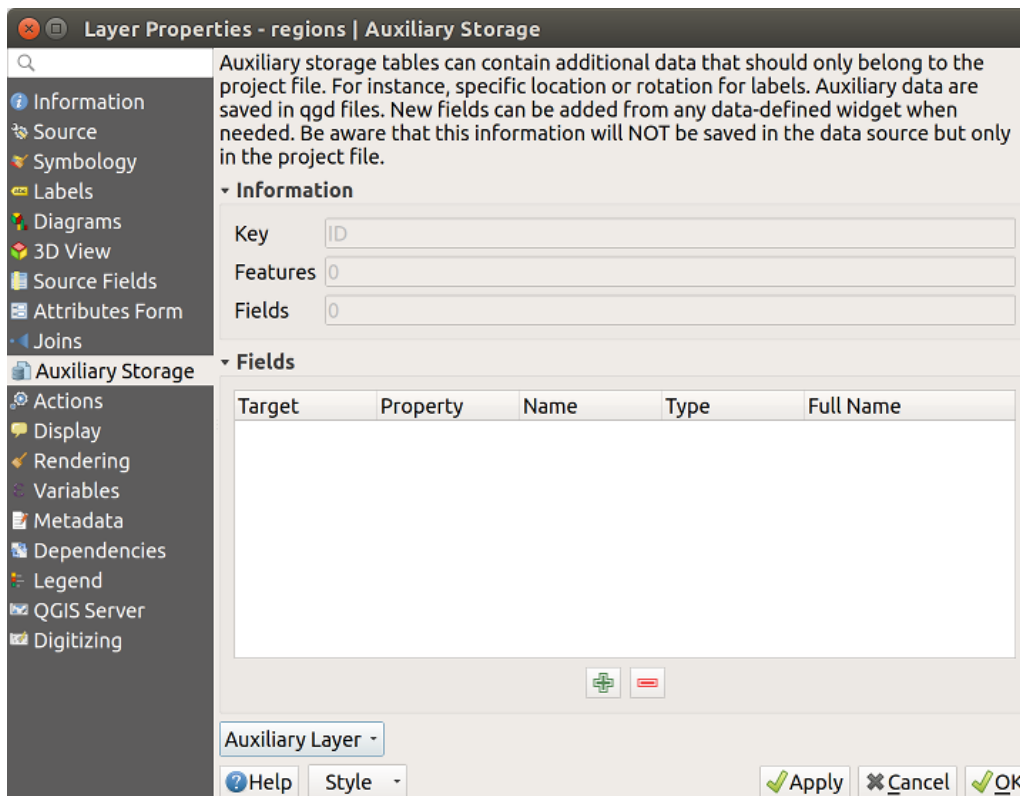
Fig. 12.56: Auxiliary Layer key
