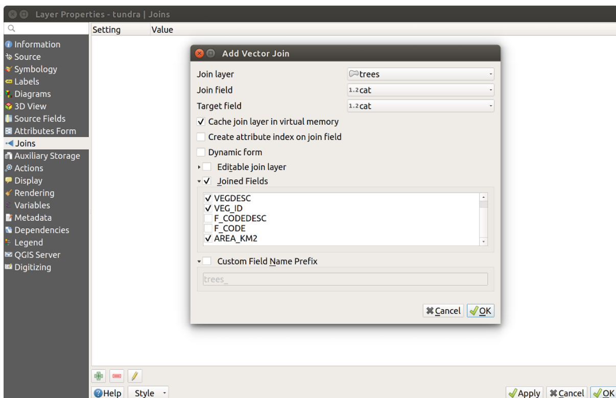
Fig. 12.53: Join an attribute table to an existing vector layer
