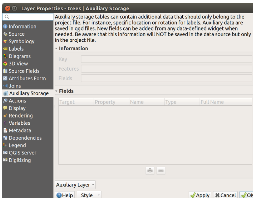
Fig. 12.54: Auxiliary Storage tab
