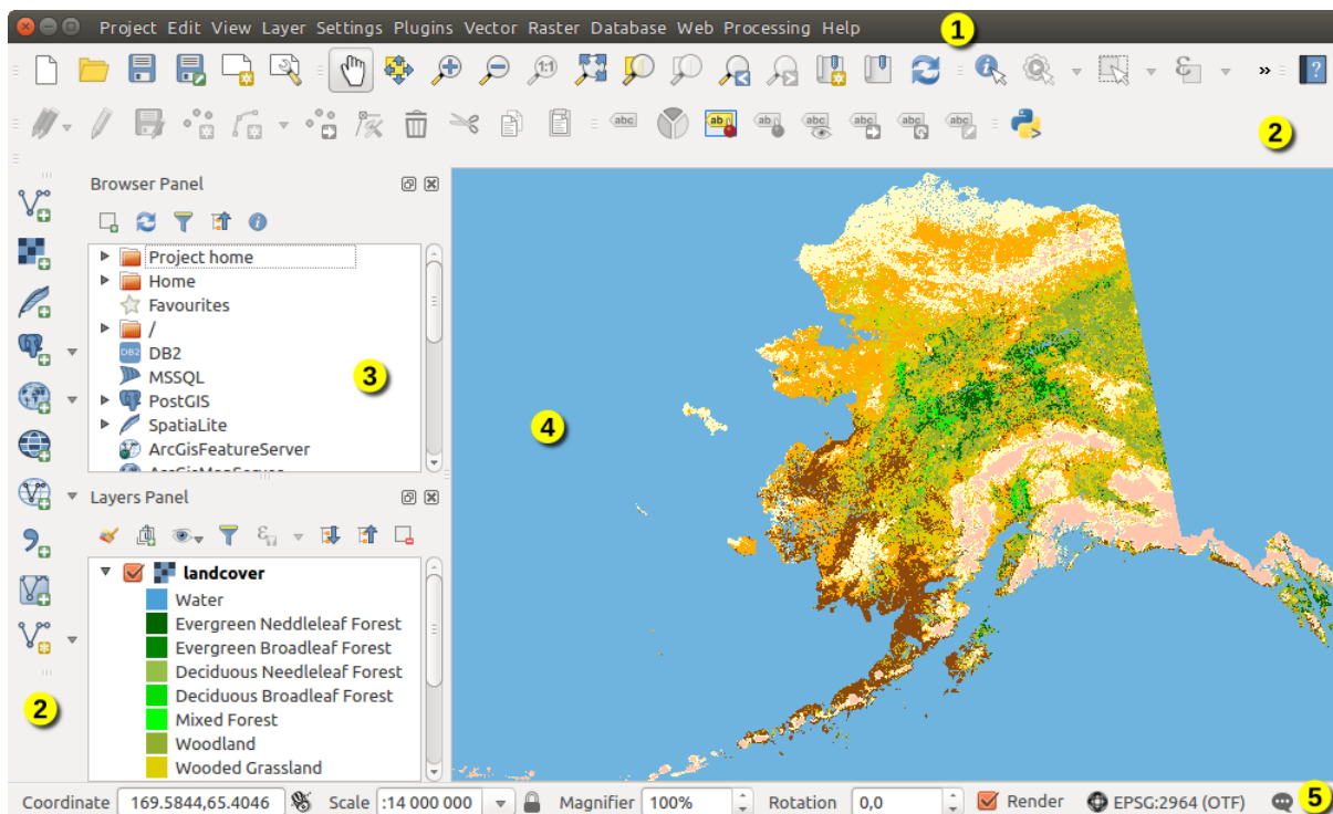
Fig. 7.1: QGIS GUI with Alaska sample data
