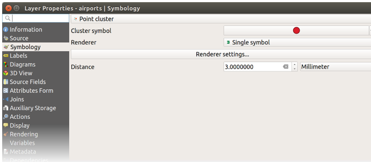
Fig. 12.17: Point Cluster dialog
