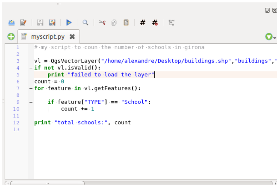
Fig. 20.2: The Python Console editor
