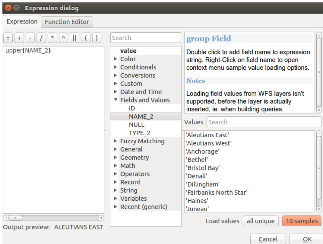
Fig. 12.73: The Expression tab
