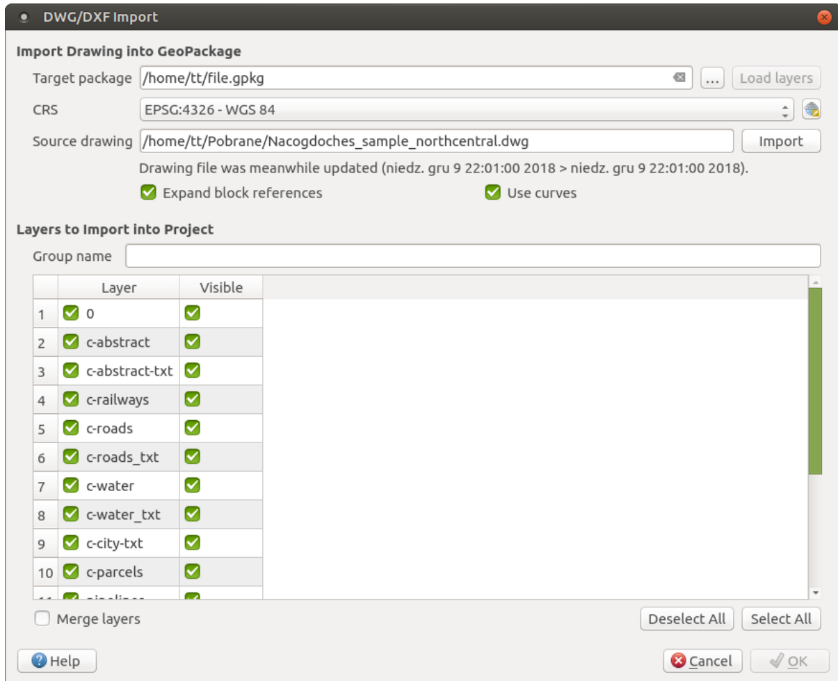
Fig. 11.8: Import dialog for DWG/DXF files
