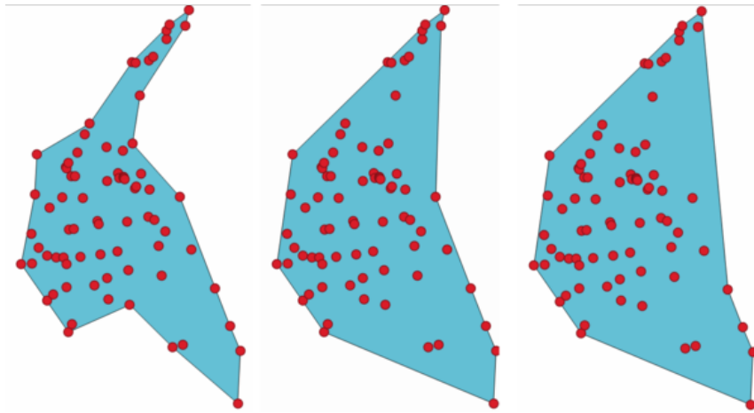
Şekil 24.49: Concave hulls with different thresholds (0.3, 0.6, 0.9)
