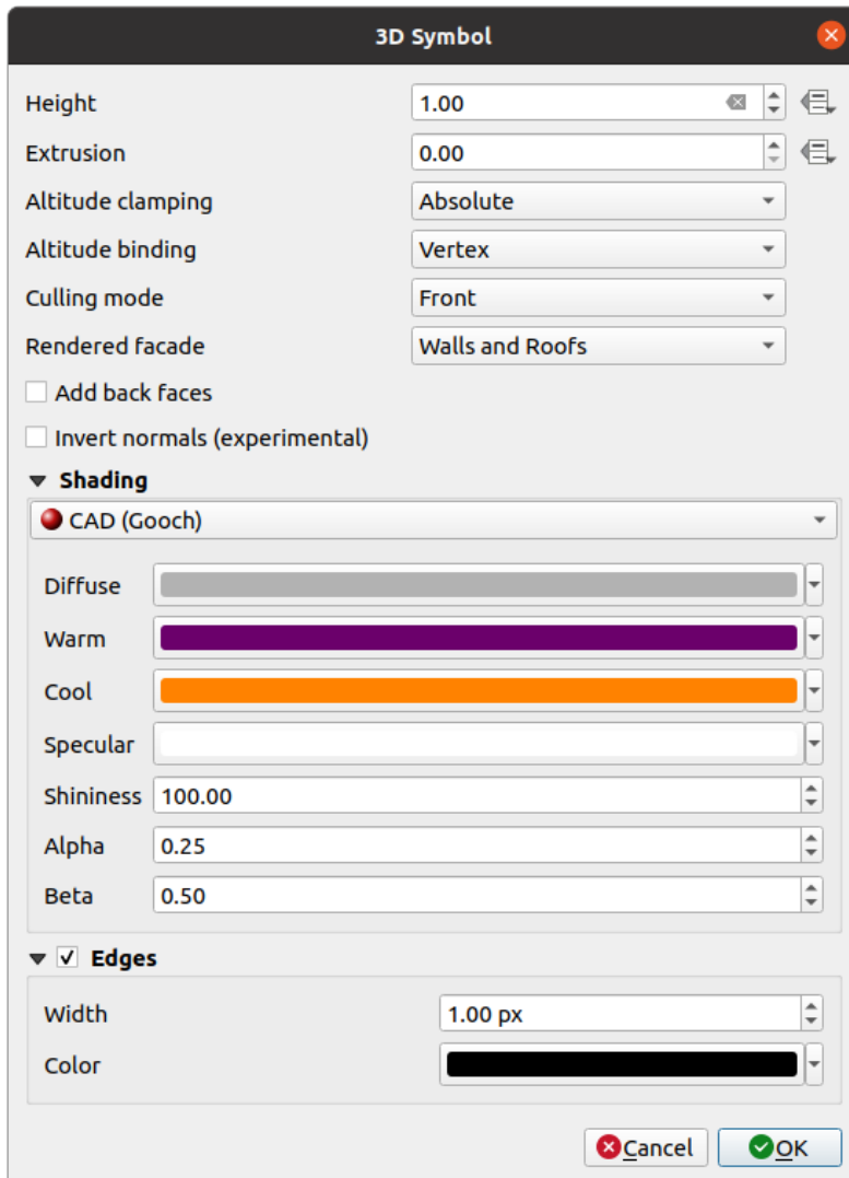
Şekil 12.26: Properties of a 3D polygon symbol
