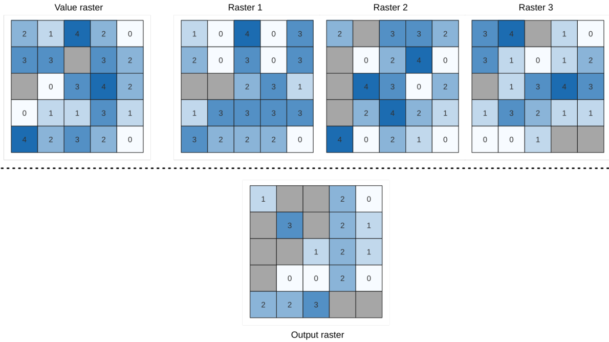
Şekil 24.12: For each cell in the output raster, the value represents the number of times that the corresponding cells in the list of rasters are less than the value raster. NoData cells (grey) are taken into account.
