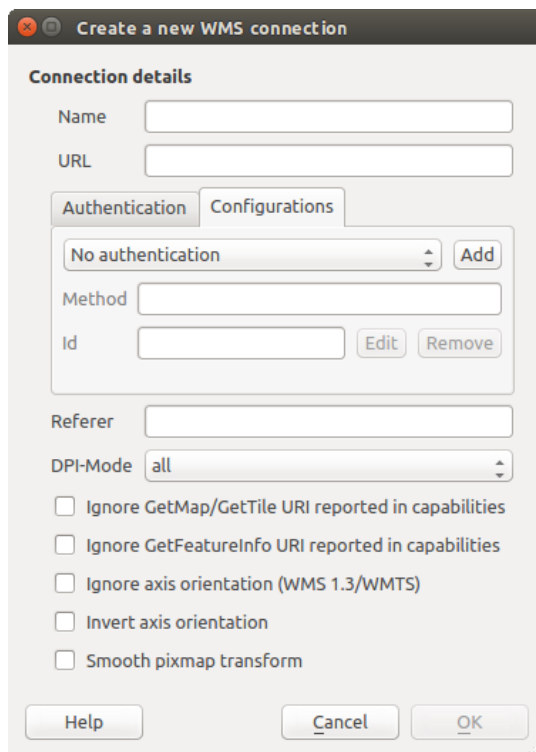
Şekil 21.7: WMS connection dialog showing Add , Edit , and Remove authentication configuration buttons
