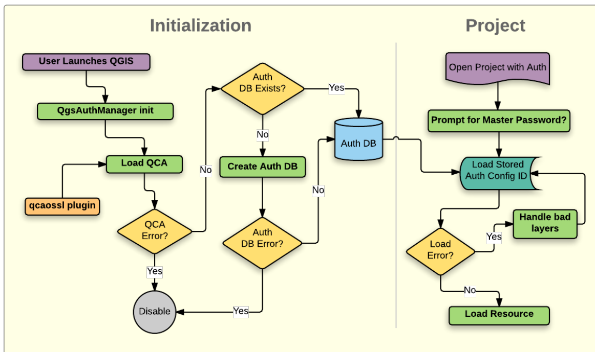
Şekil 21.1: Anatomy of authentication system
