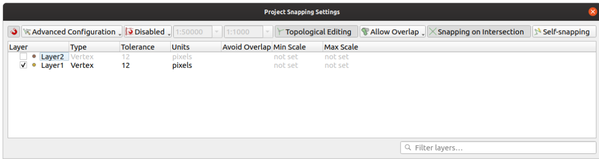
Şekil 14.84: Snapping options (Advanced Configuration mode)
