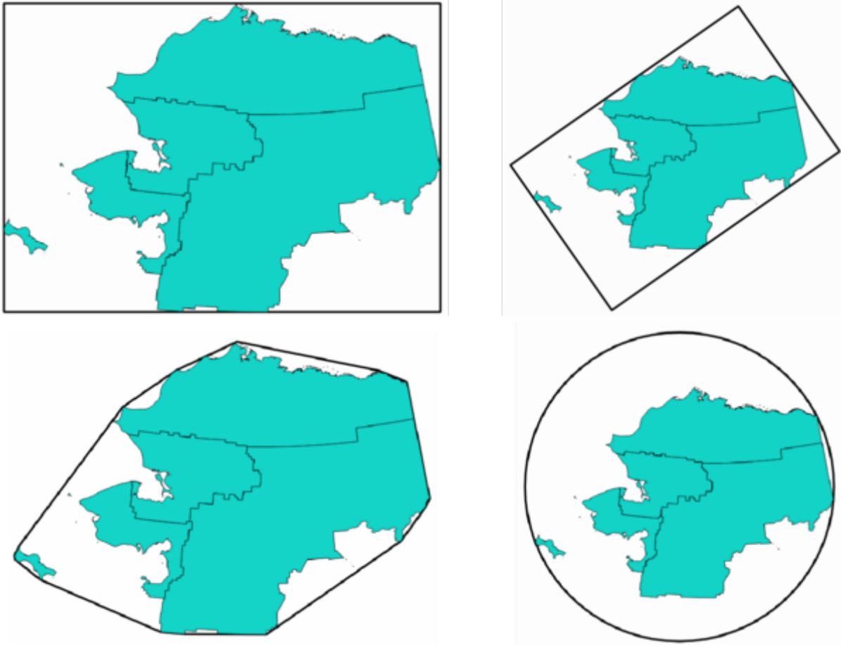
Şekil 24.66: Clockwise from top left: envelope, oriented rectangle, circle, convex hull
