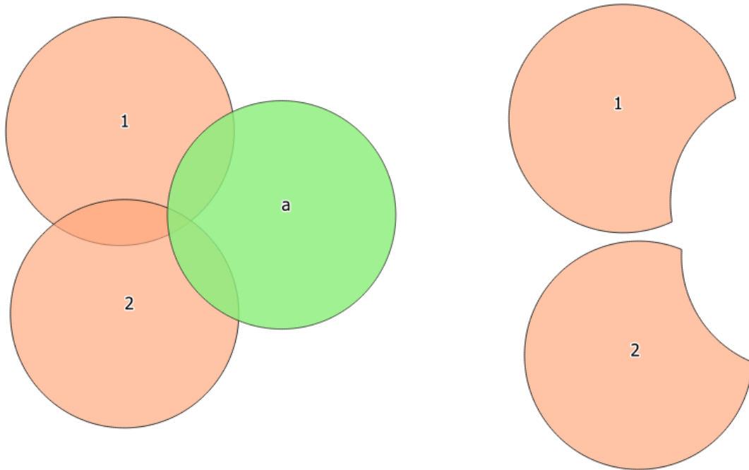
Şekil 24.93: Difference operation between a two-features input layer and a single feature overlay layer (left) - resulting features are moved for clarity (right)
