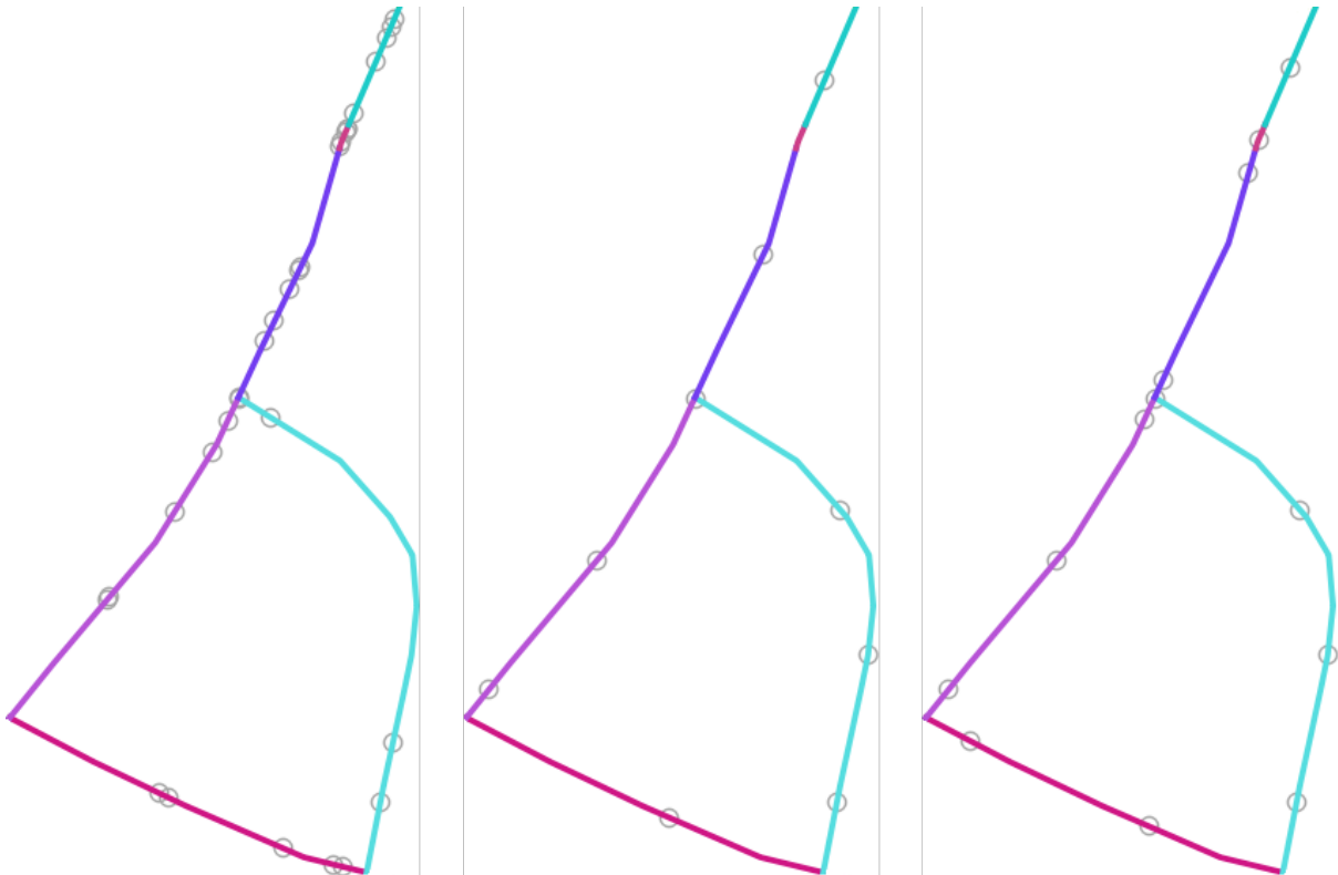
Şekil 24.37: Five points per line feature, left : min. distances = 0, middle : min.distances != 0, right : min. distance != 0, global min. distance = 0
