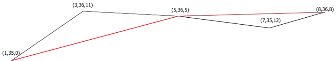
Şekil 24.61: The red line represents the black line with only vertices whose M value is \leq 10 .
