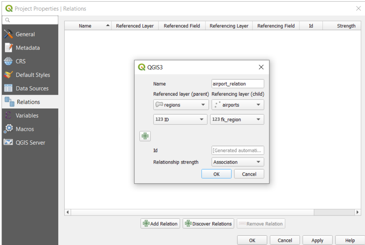
Şekil 14.77: Adding a relation between regions and airports layers
