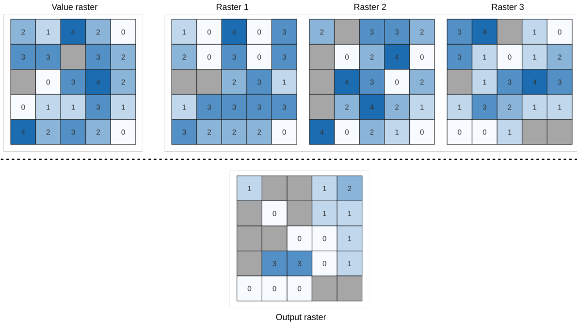
Şekil 24.11: For each cell in the output raster, the value represents the number of times that the corresponding cells in the list of rasters are greater than the value raster. NoData cells (grey) are taken into account.
