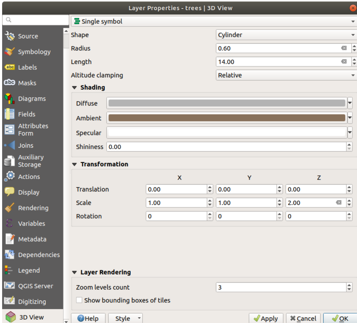
Şekil 14.40: 3D properties of a point layer
