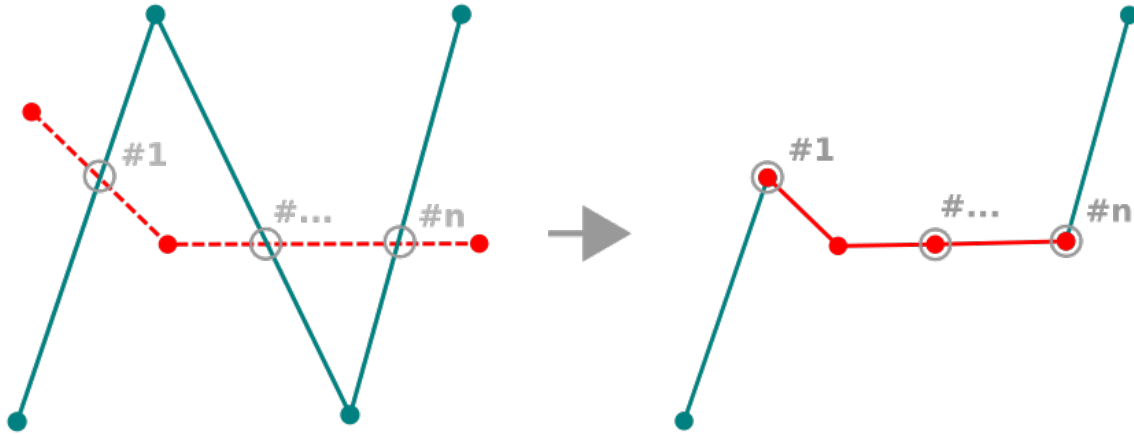
Şekil 14.91: Reshape line
