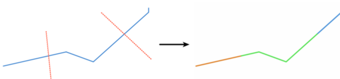
Şekil 24.96: Split lines
