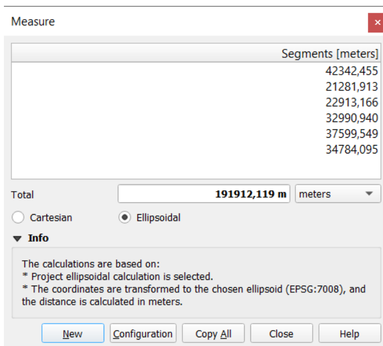
Şekil 11.17: Measure Distance
