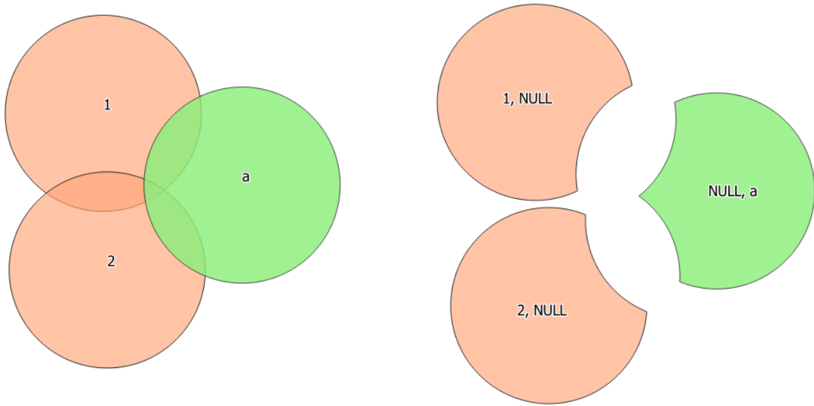
Şekil 24.97: Symmetrical difference operation between a two-features input layer and a single feature overlay layer (left) - resulting features are moved for clarity (right)
