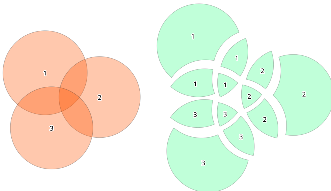
Şekil 24.98: Union operation with a single input layer of three overlapping features (left) - resulting features are moved for clarity (right)
