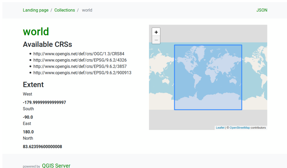
Рис. 3.4: Server WFS3 collection detail page
