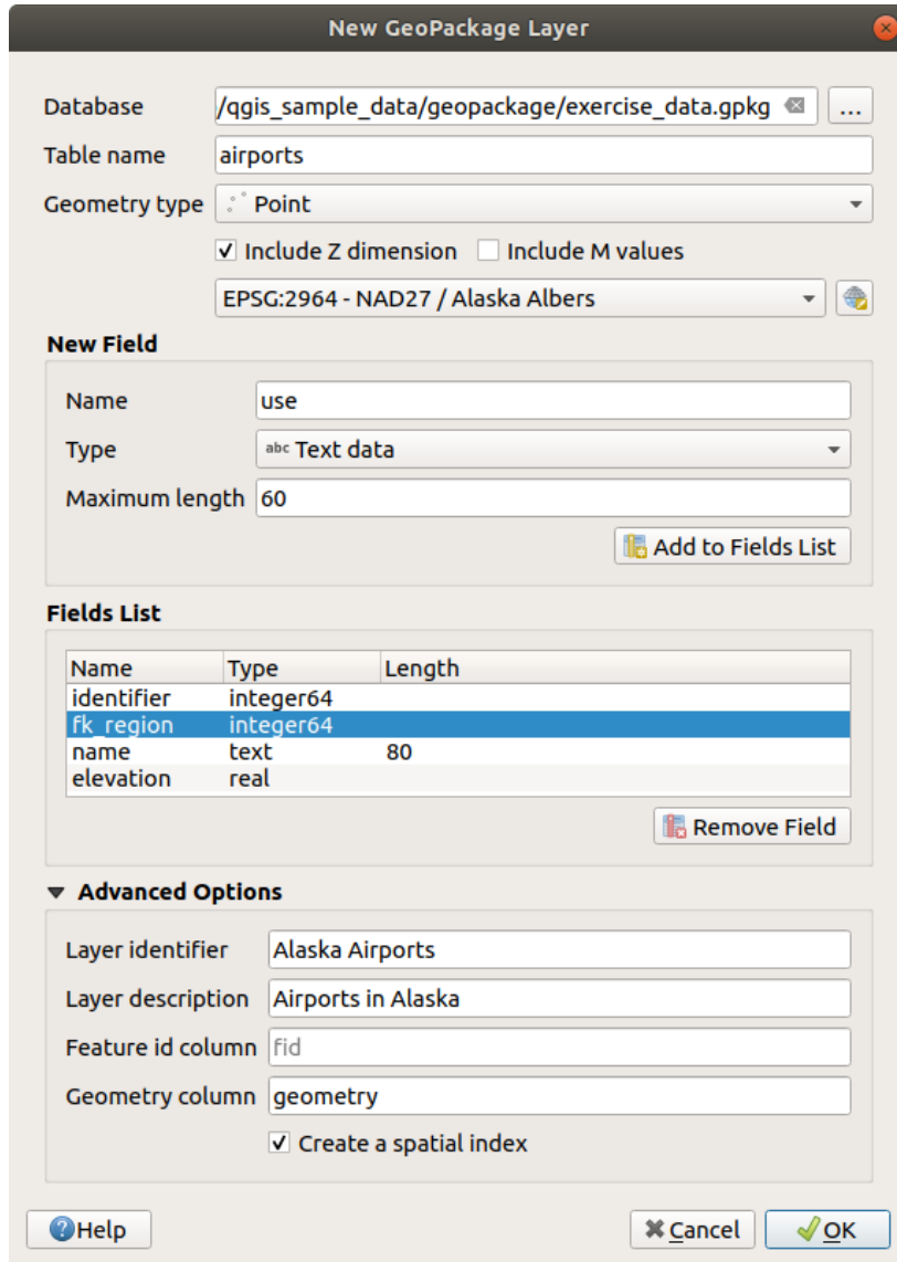
Рис. 13.15: Creating a New GeoPackage layer dialog
