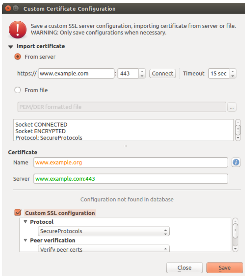
Рис. 21.36: Manually adding configuration
