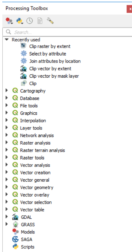
Рис. 23.6: Processing Toolbox
