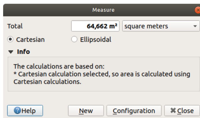
Рис. 11.18: Measure Area
