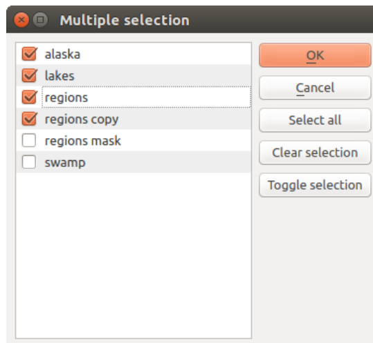
Рис. 23.12: Multiple Selection
