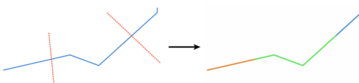
Рис. 24.96: Split lines
