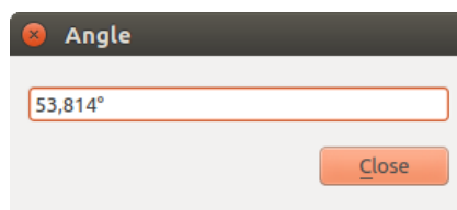
Рис. 11.19: Measure Angle
