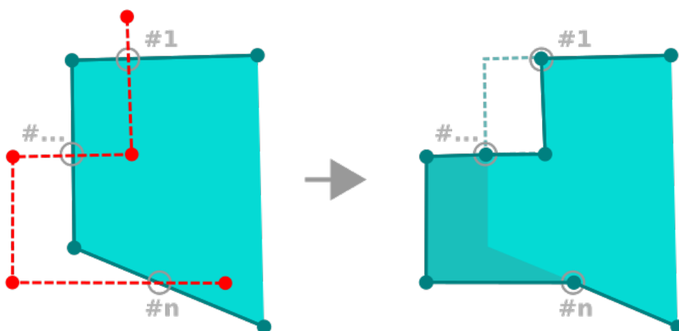
Рис. 14.92: Reshape polygon
