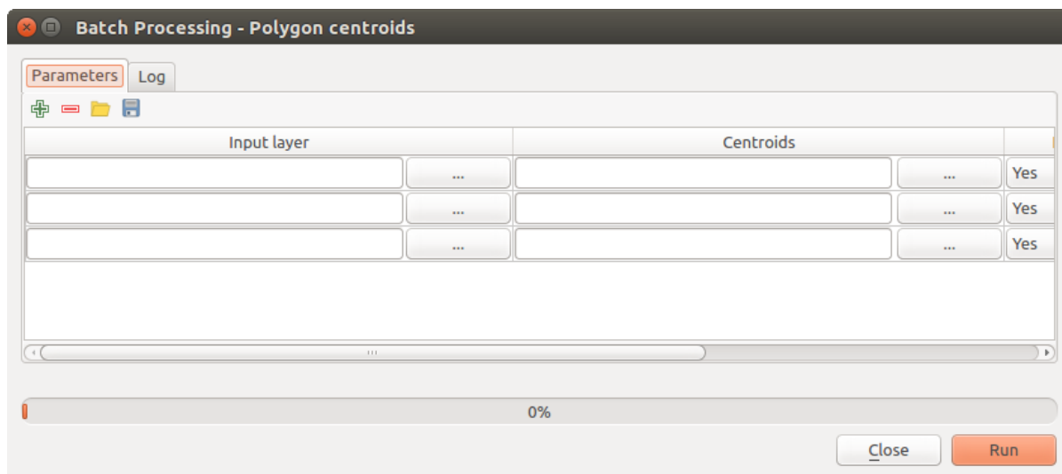
Рис. 23.31: Batch Processing
