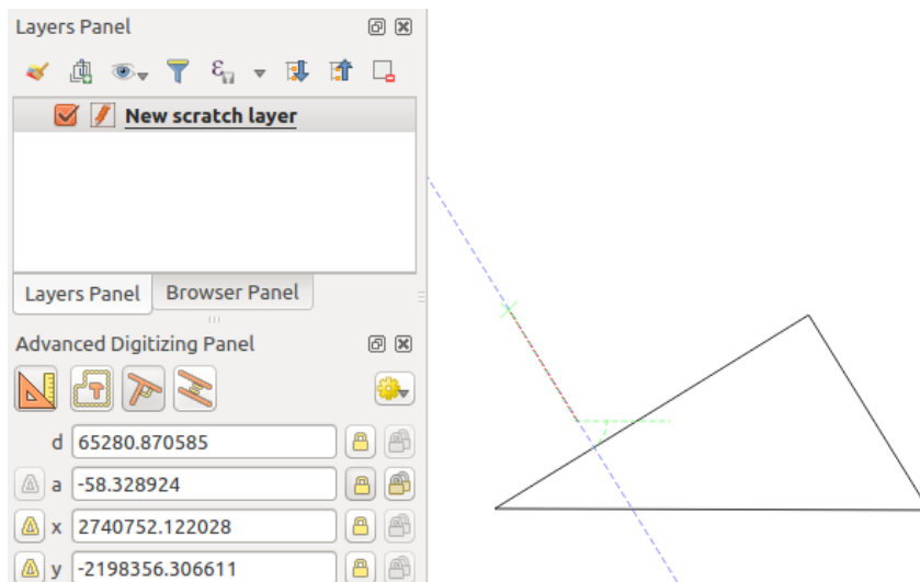
Рис. 14.99: Perpendicular digitizing
