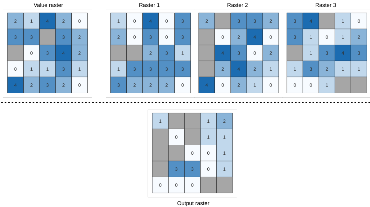
Рис. 24.11: For each cell in the output raster, the value represents the number of times that the corresponding cells in the list of rasters are greater than the value raster. NoData cells (grey) are taken into account.
