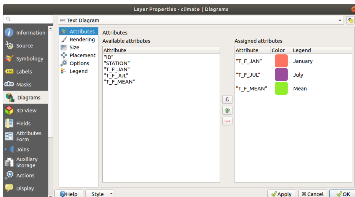
Рис. 14.35: Diagram properties - Attributes tab
