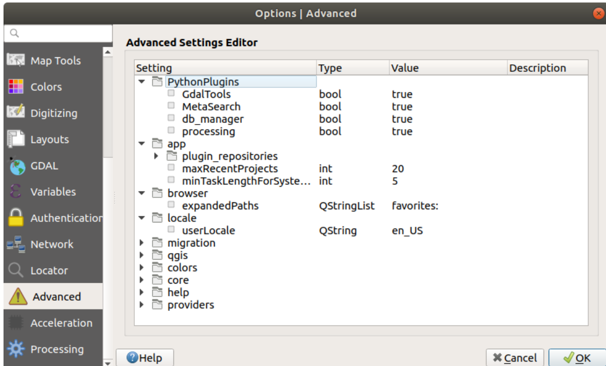
Рис. 9.18: Advanced Settings tab in QGIS
