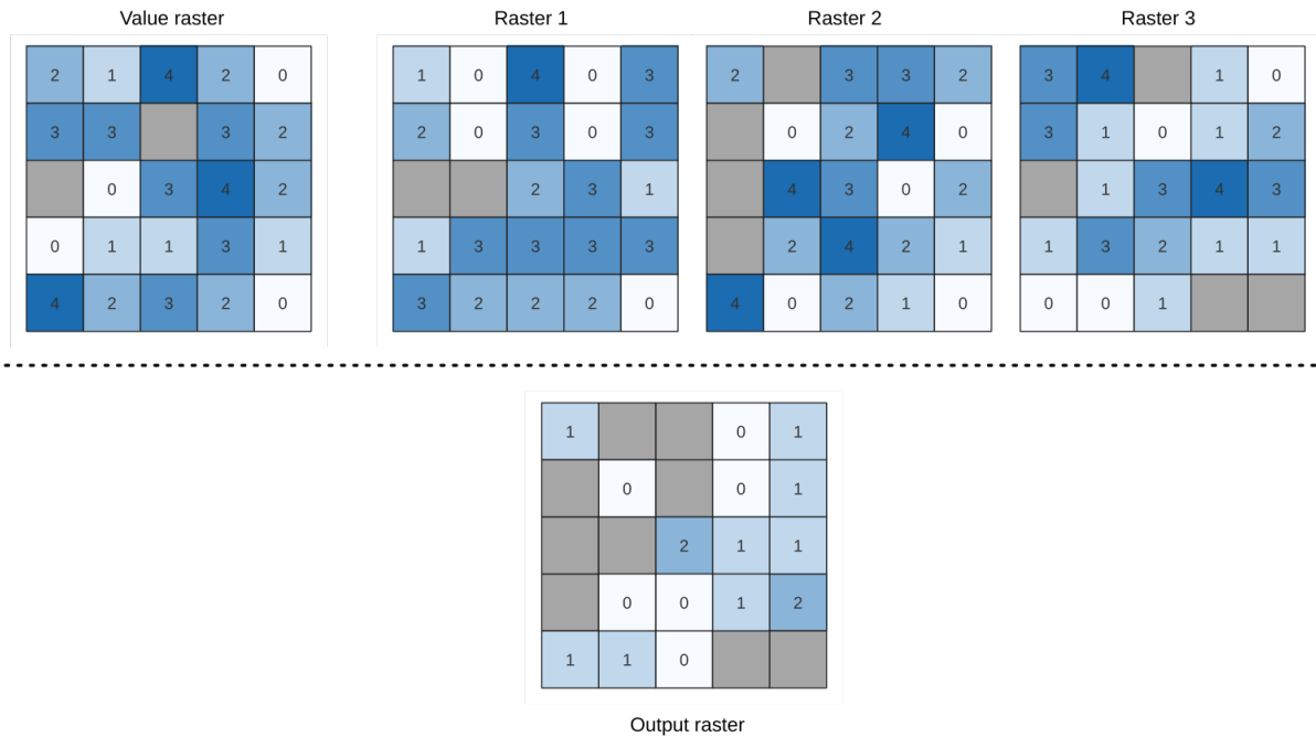
Рис. 24.9: For each cell in the output raster, the value represents the number of times that the corresponding cells in the list of rasters are the same as the value raster. NoData cells (grey) are taken into account.
