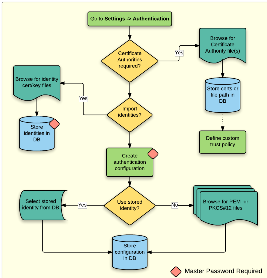
Рис. 21.22: PKI configuration workflow
