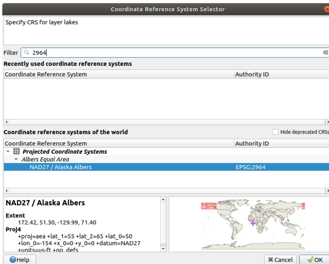
Рис. 5.2: Select the Coordinate Reference System of data
