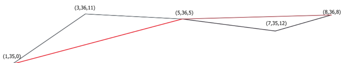
Рис. 24.62: The red line represents the black line with only vertices whose Z value is \leq 10 .
