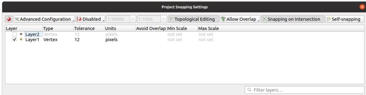
Рис. 14.84: Snapping options (Advanced Configuration mode)
