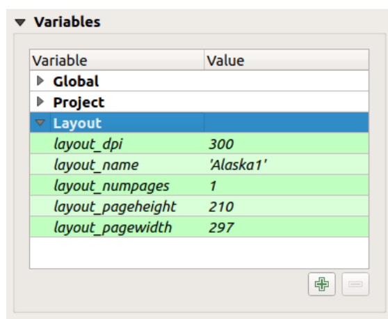
Рис. 18.4: Variables Editor in the Print Layout
