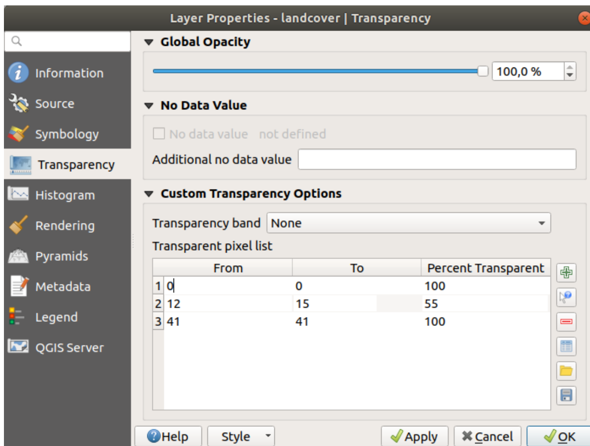
Рис. 15.10: Raster Transparency
