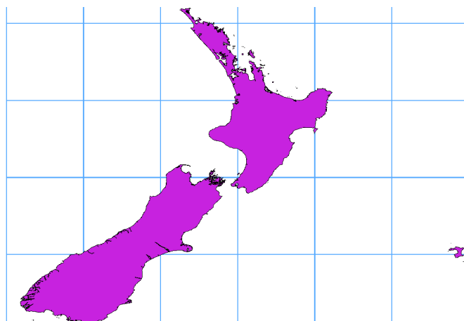
Рис. 13.24: Crossing 180^\circ longitude applying the ST_Shift_Longitude function
