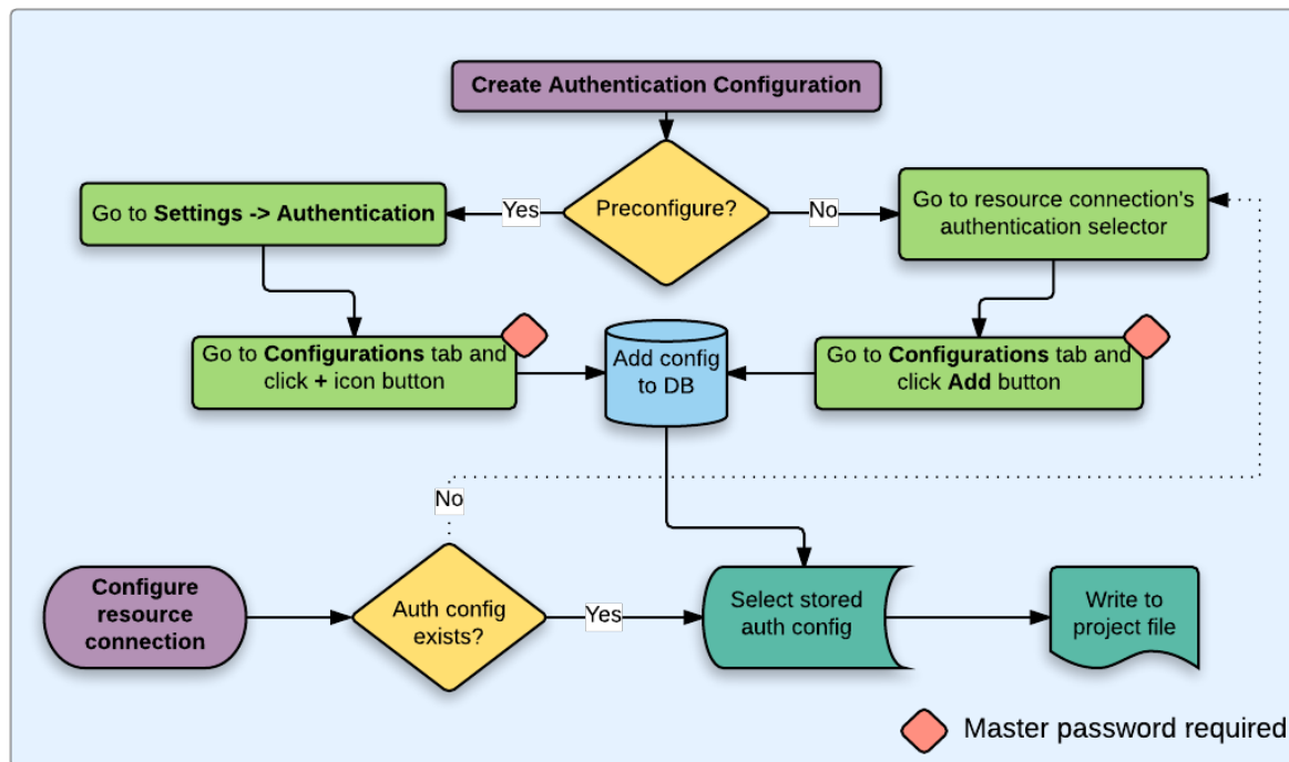
Рис. 21.19: Generic user workflow
