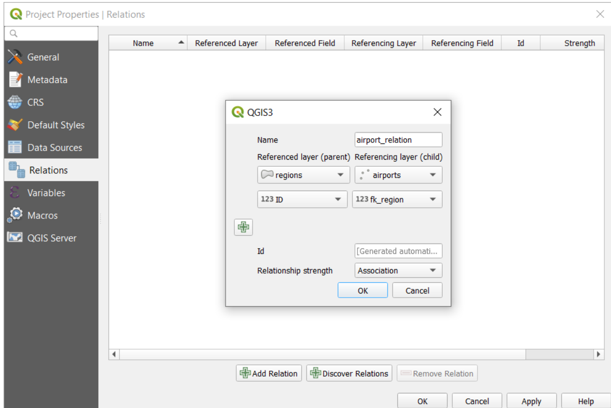
Рис. 14.77: Adding a relation between regions and airports layers
