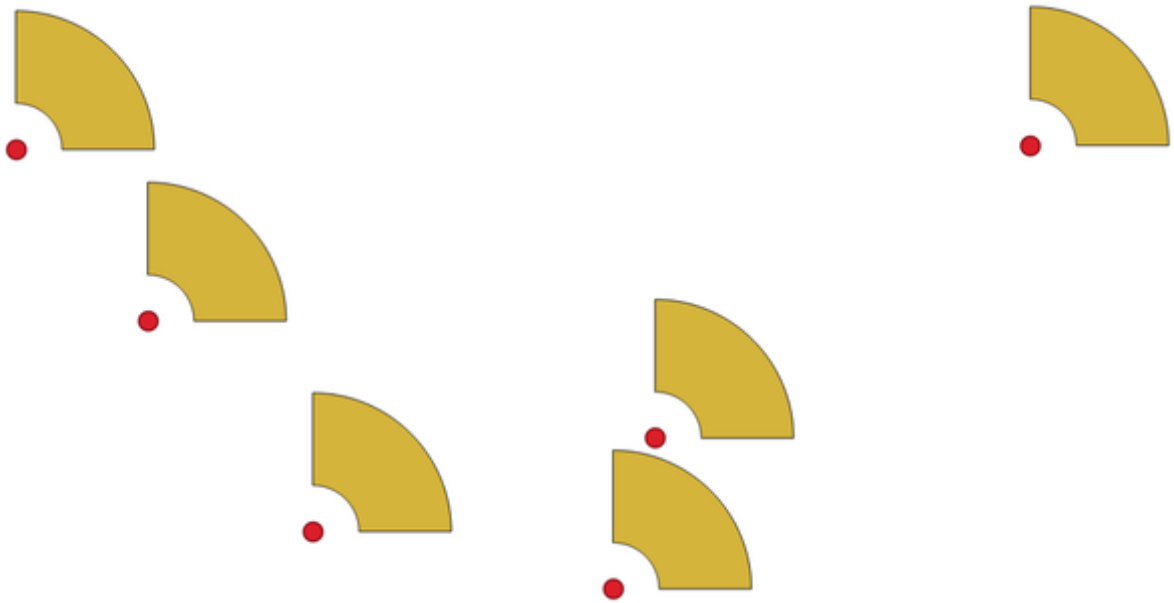
Рис. 24.51: Wedge buffers
