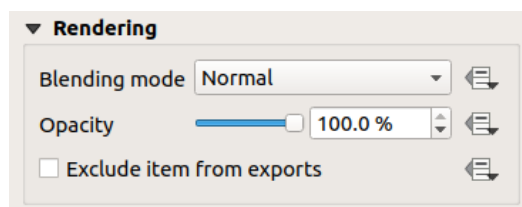
Рис. 18.13: Rendering mode
