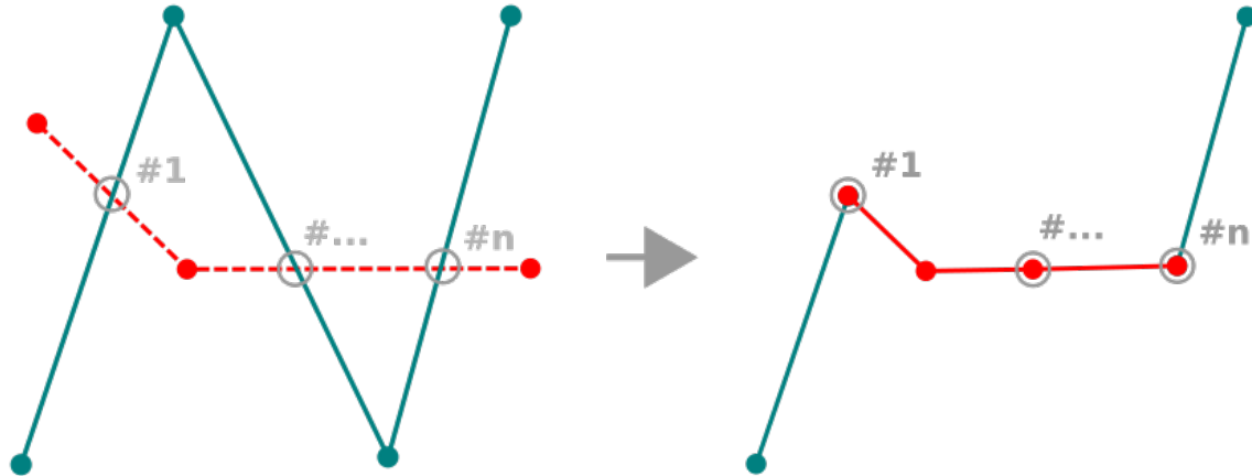
Рис. 14.91: Reshape line
