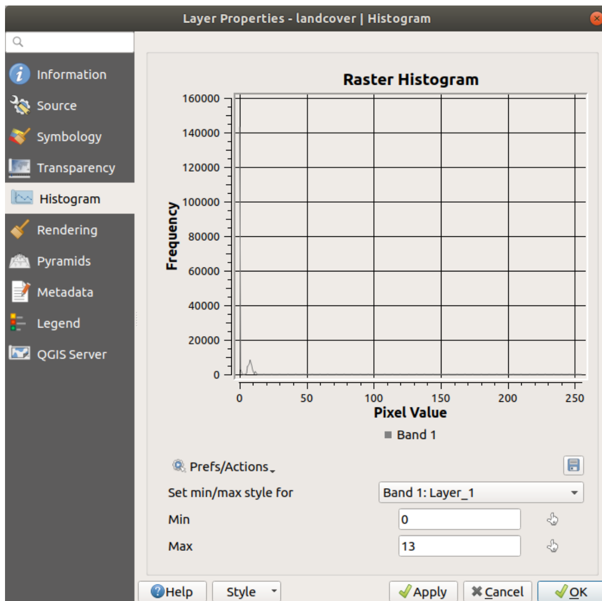
Рис. 15.11: Raster Histogram
