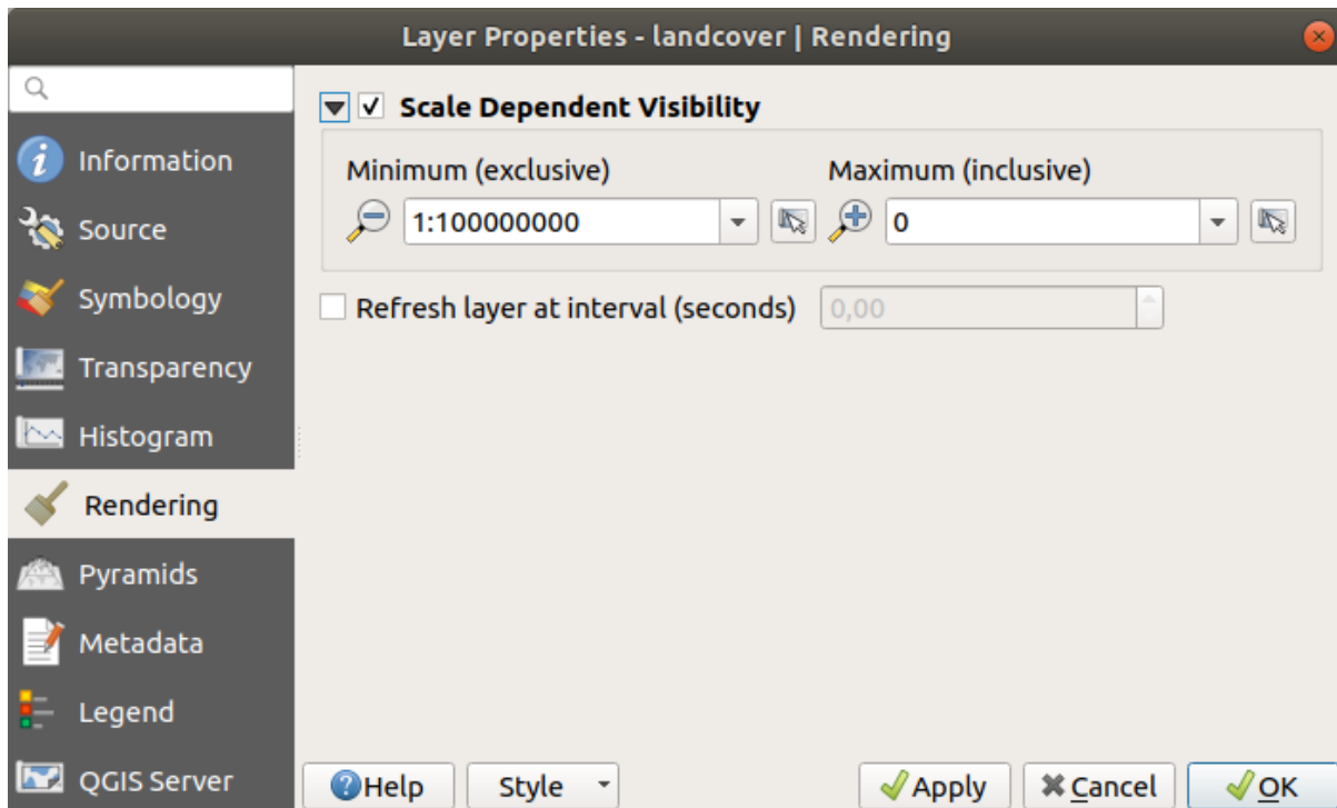
Рис. 15.12: Raster Rendering
