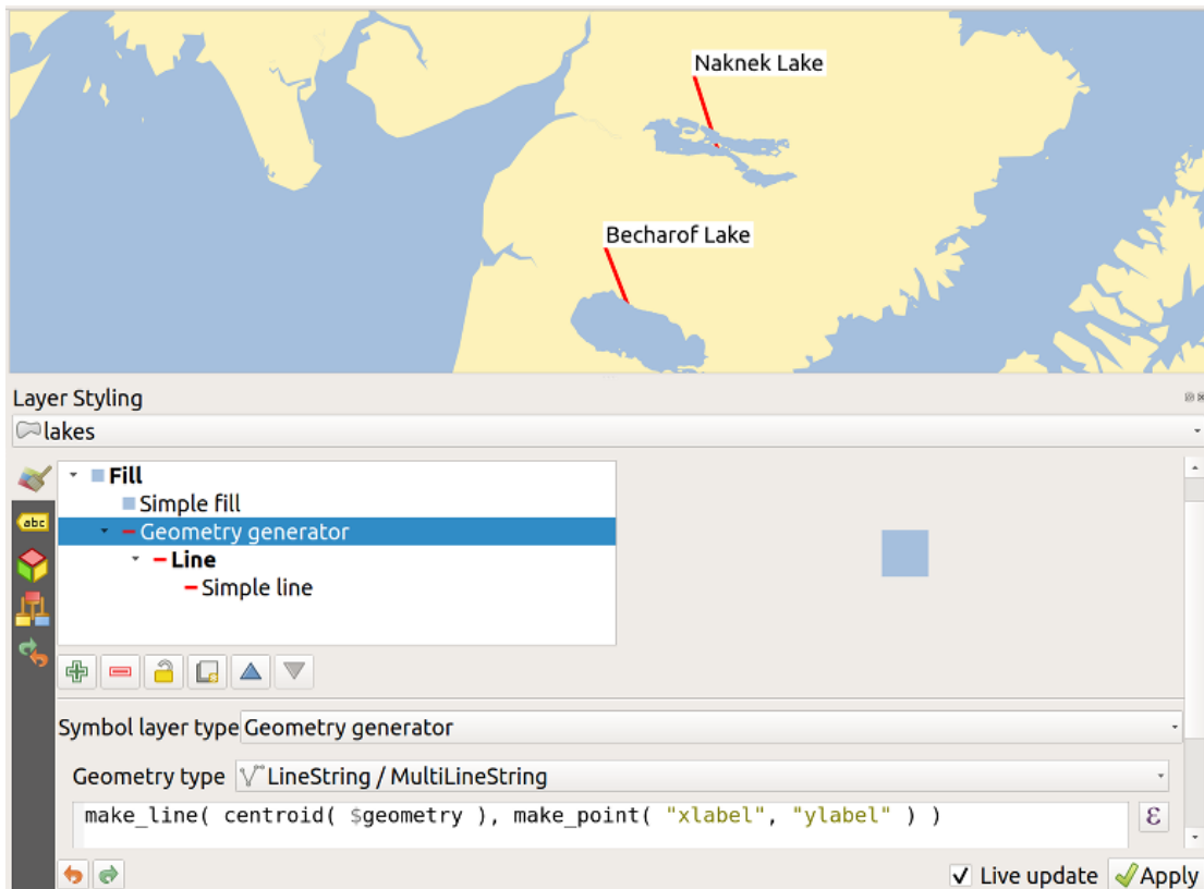
Рис. 14.34: Moved labels
