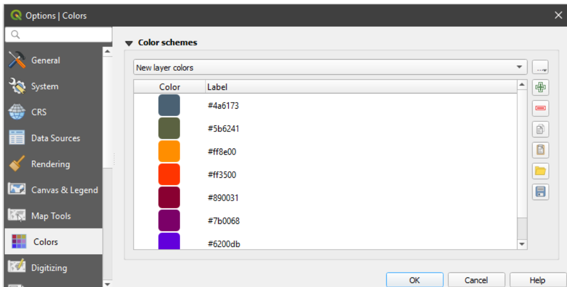
Fig. 9.8: Colors Settings
