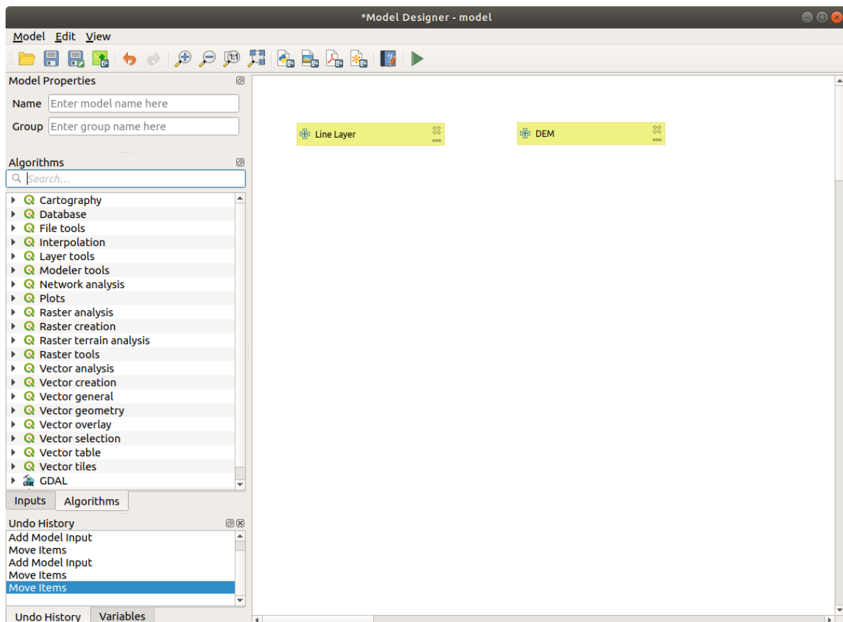
Fig. 23.19: Model Inputs
