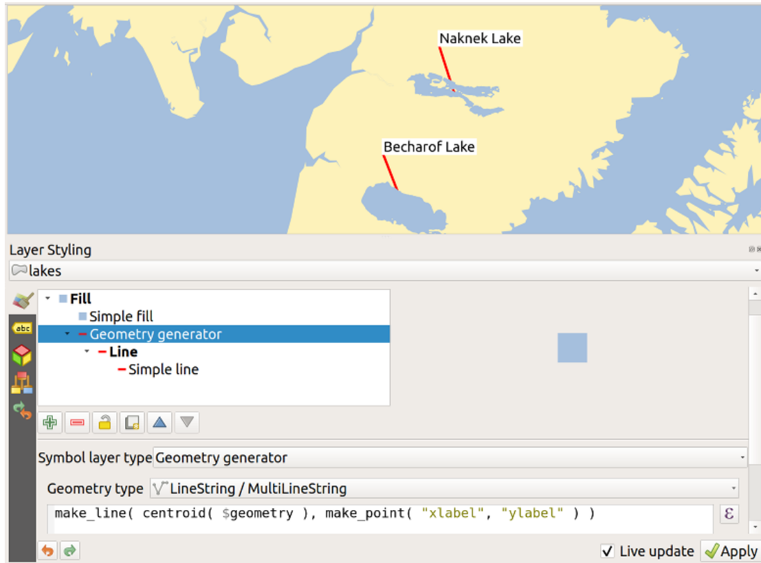
Fig. 14.34: Moved labels
