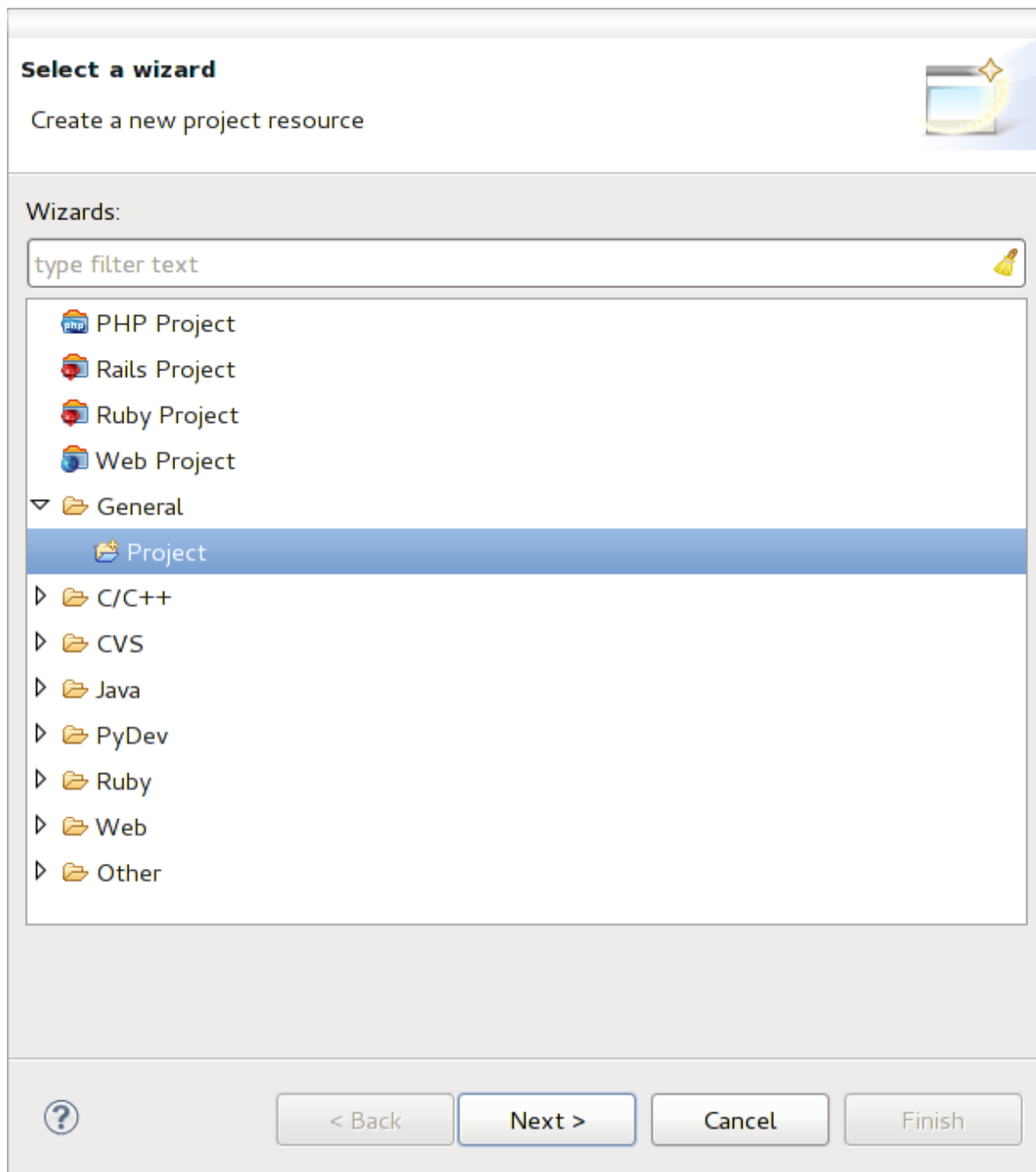
Gambar. 16.1: Eclipse project
