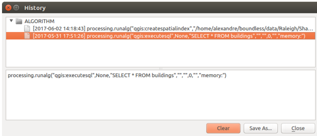
Gambar. 23.3: Processing History
