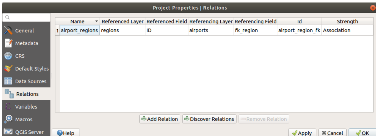
Gambar. 9.26: Relations tab
