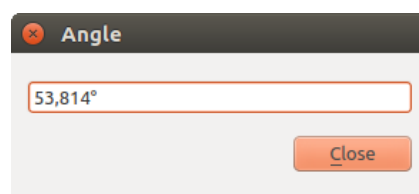
Gambar. 11.19: Measure Angle
