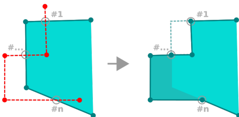
Gambar. 14.92: Reshape polygon
