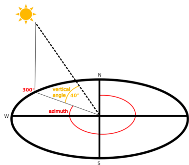
Gambar. 24.18: Azimuth and vertical angle
