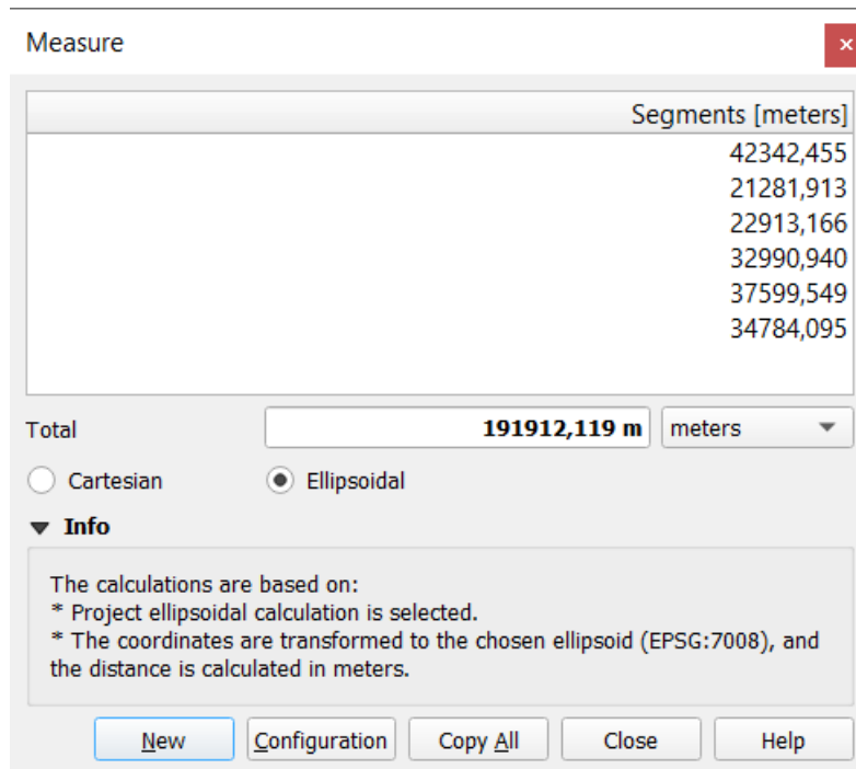
Gambar. 11.17: Measure Distance
