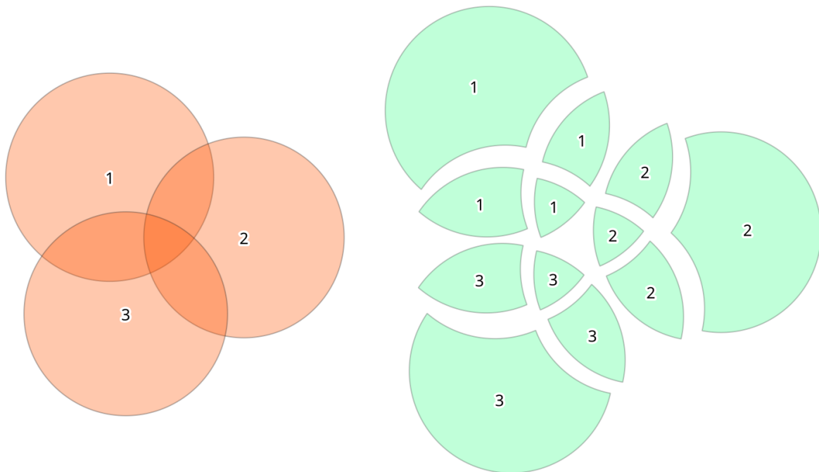
Gambar. 24.98: Union operation with a single input layer of three overlapping features (left) - resulting features are moved for clarity (right)
