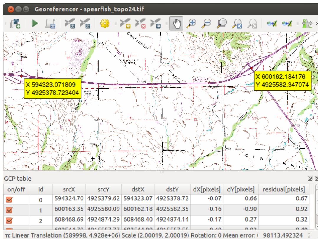
Gambar. 15.20: Georeferencer Dialog
