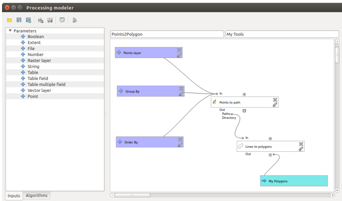
Gambar. 23.2: Processing Modeler
