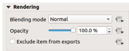
Gambar. 18.13: Rendering mode
