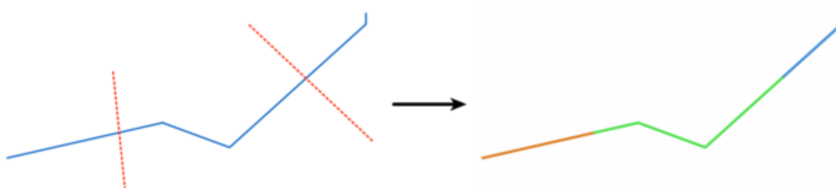
Gambar. 24.96: Split lines
