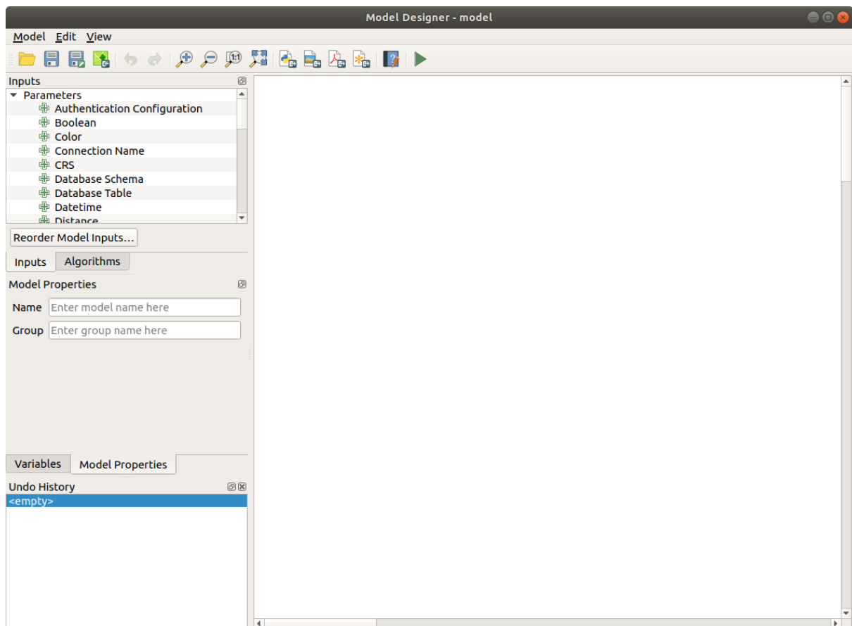
Gambar. 23.16: Modeler
