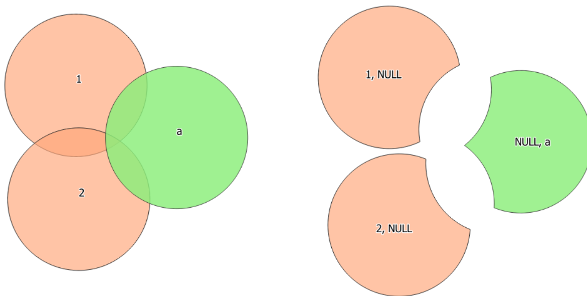
Gambar. 24.97: Symmetrical difference operation between a two-features input layer and a single feature overlay layer (left) - resulting features are moved for clarity (right)
