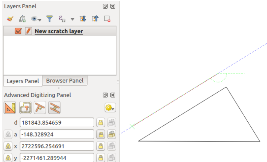
Gambar. 14.100: Parallel digitizing
