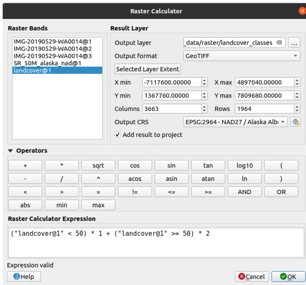
Gambar. 15.17: Raster Calculator
