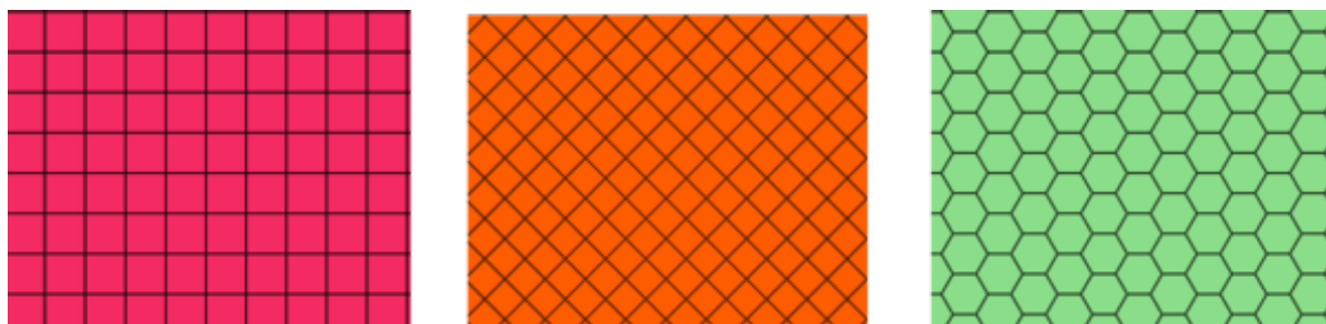
Gambar. 24.32: Different grid cell shapes
