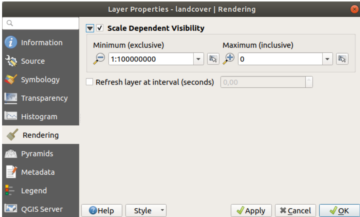
Gambar. 15.12: Raster Rendering
