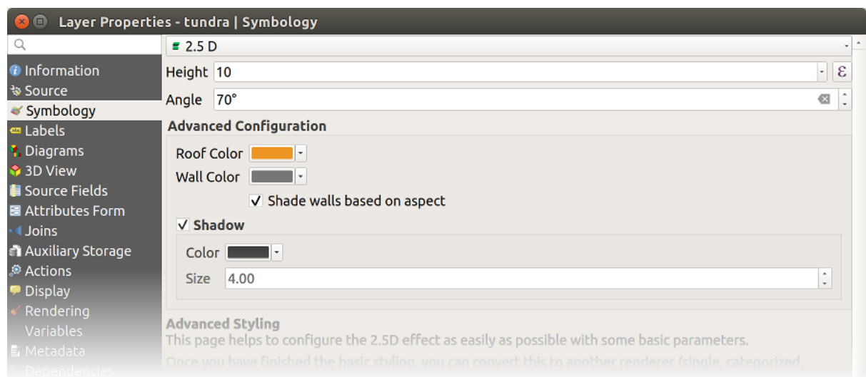
Gambar. 14.13: 2.5D dialog
