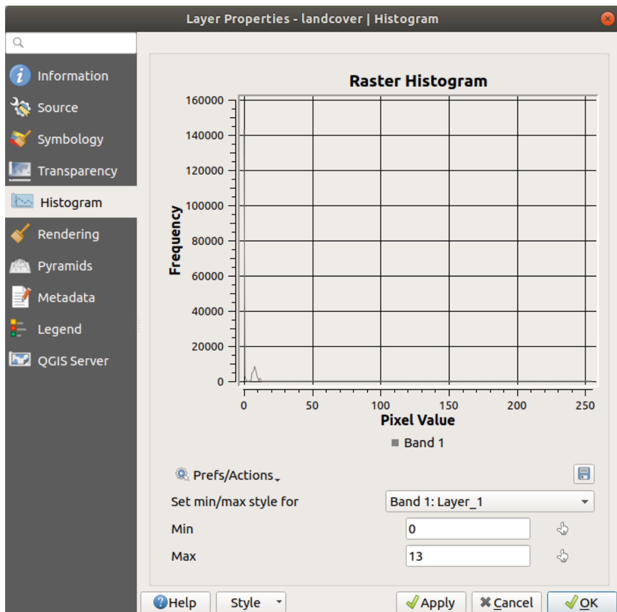
Gambar. 15.11: Raster Histogram
