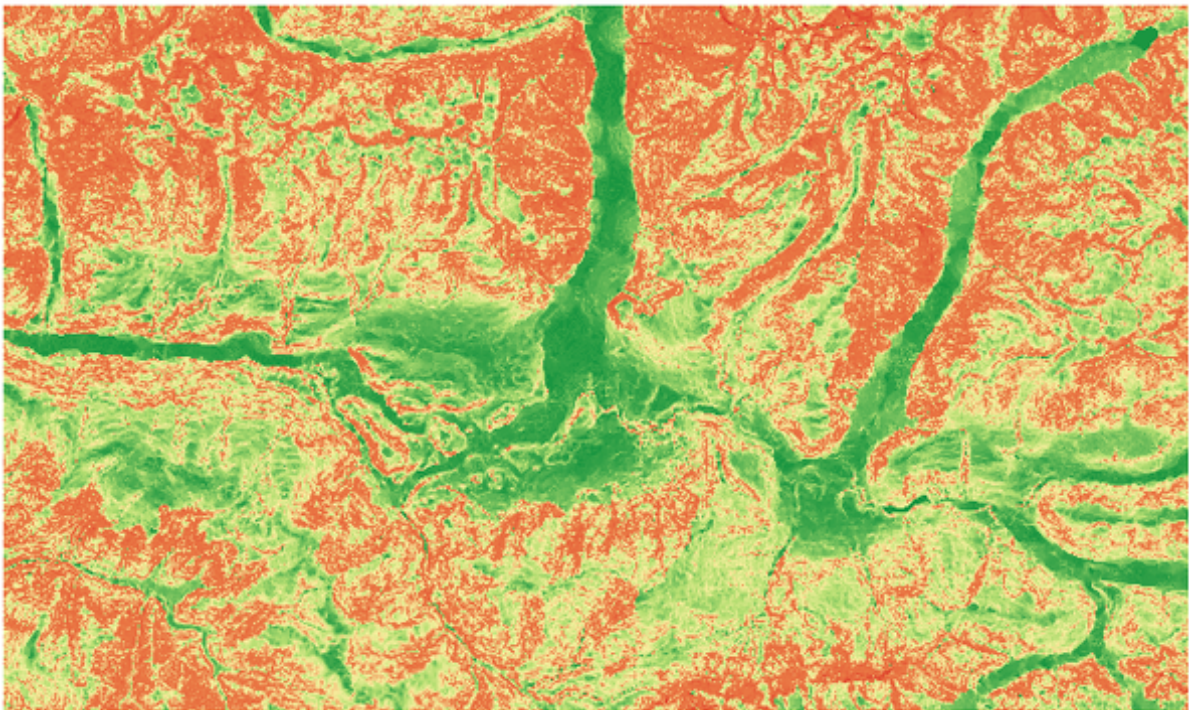
Gambar. 24.23: Ruggedness layer from low (red) to high values (green)
