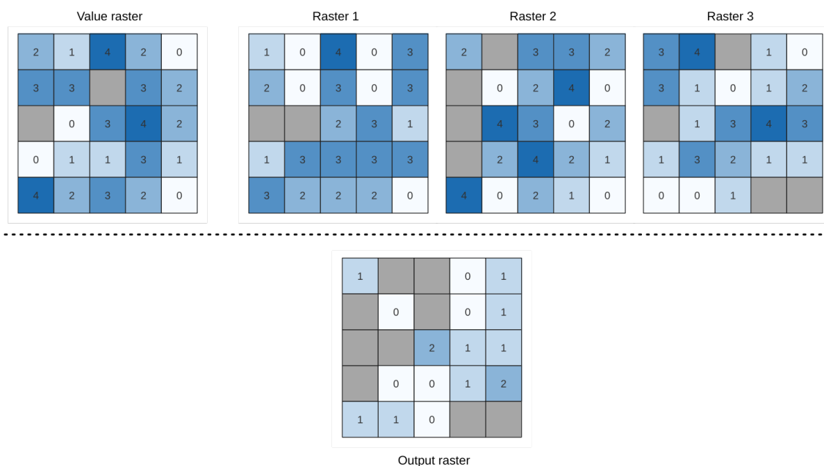
Gambar. 24.9: For each cell in the output raster, the value represents the number of times that the corresponding cells in the list of rasters are the same as the value raster. NoData cells (grey) are taken into account.
