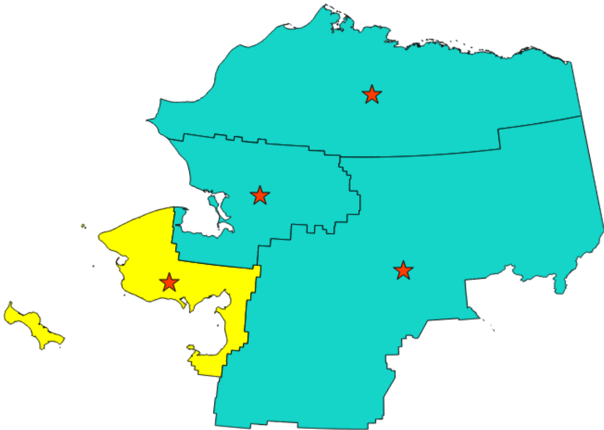
Gambar. 24.47: The red stars represent the centroids of the features of the input layer.
