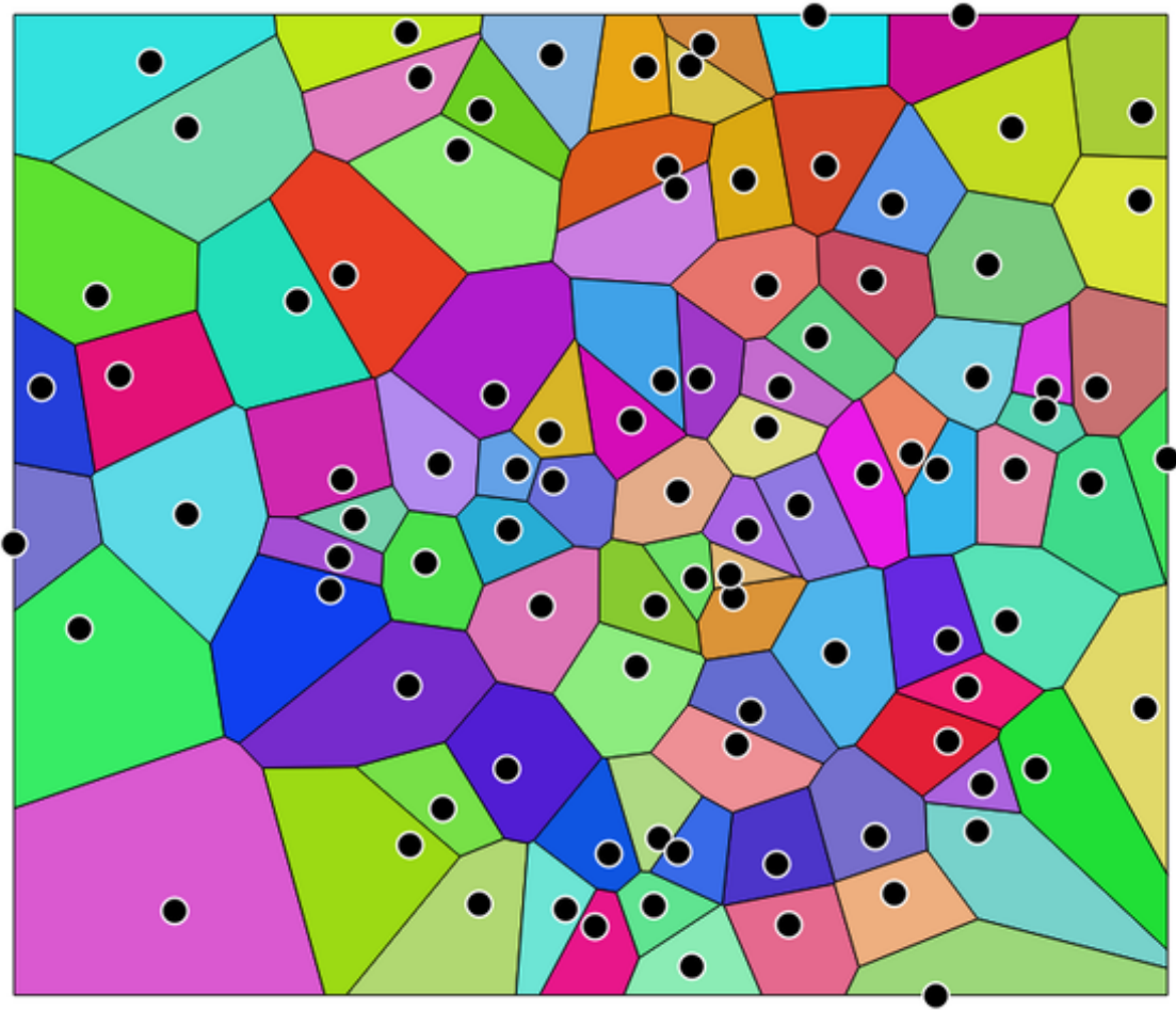
Gambar. 24.91: Voronoi polygons
