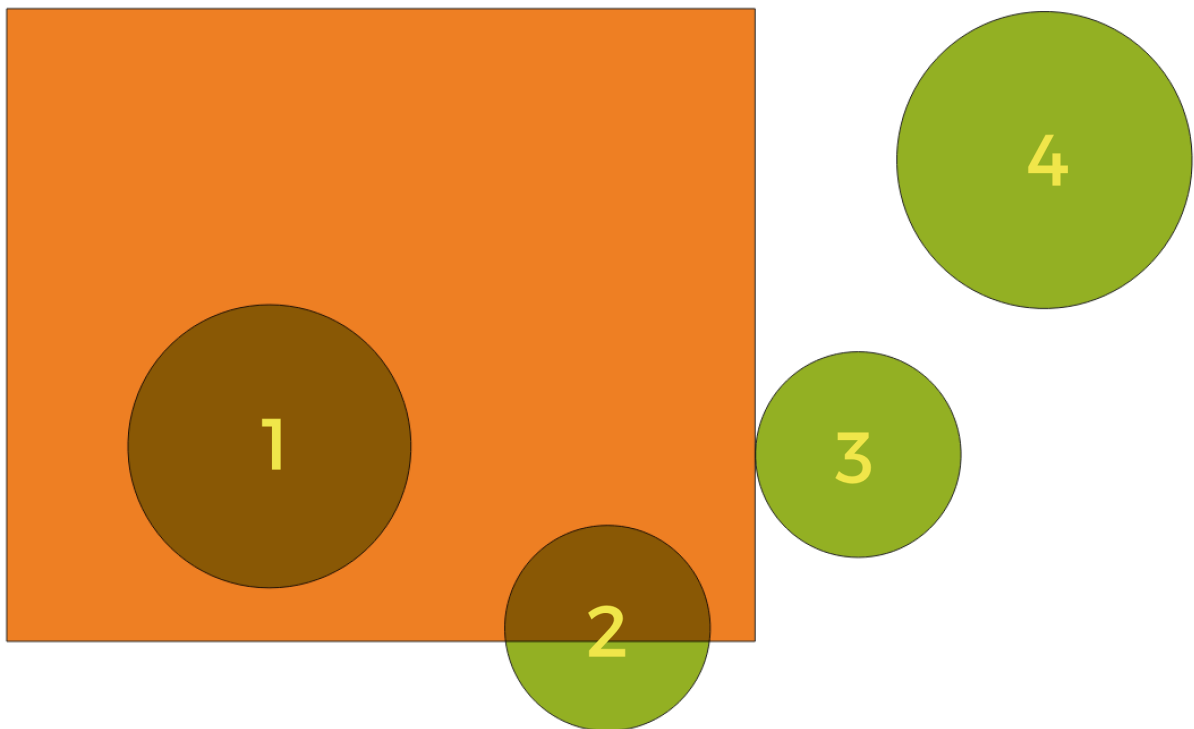
Gambar. 24.101: In this example, the dataset from which we want to select (the source vector layer ) consists of the green circles, the orange rectangle is the dataset that it is being compared to (the intersection vector layer ).
