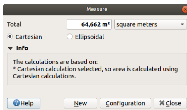
Gambar. 11.18: Measure Area
