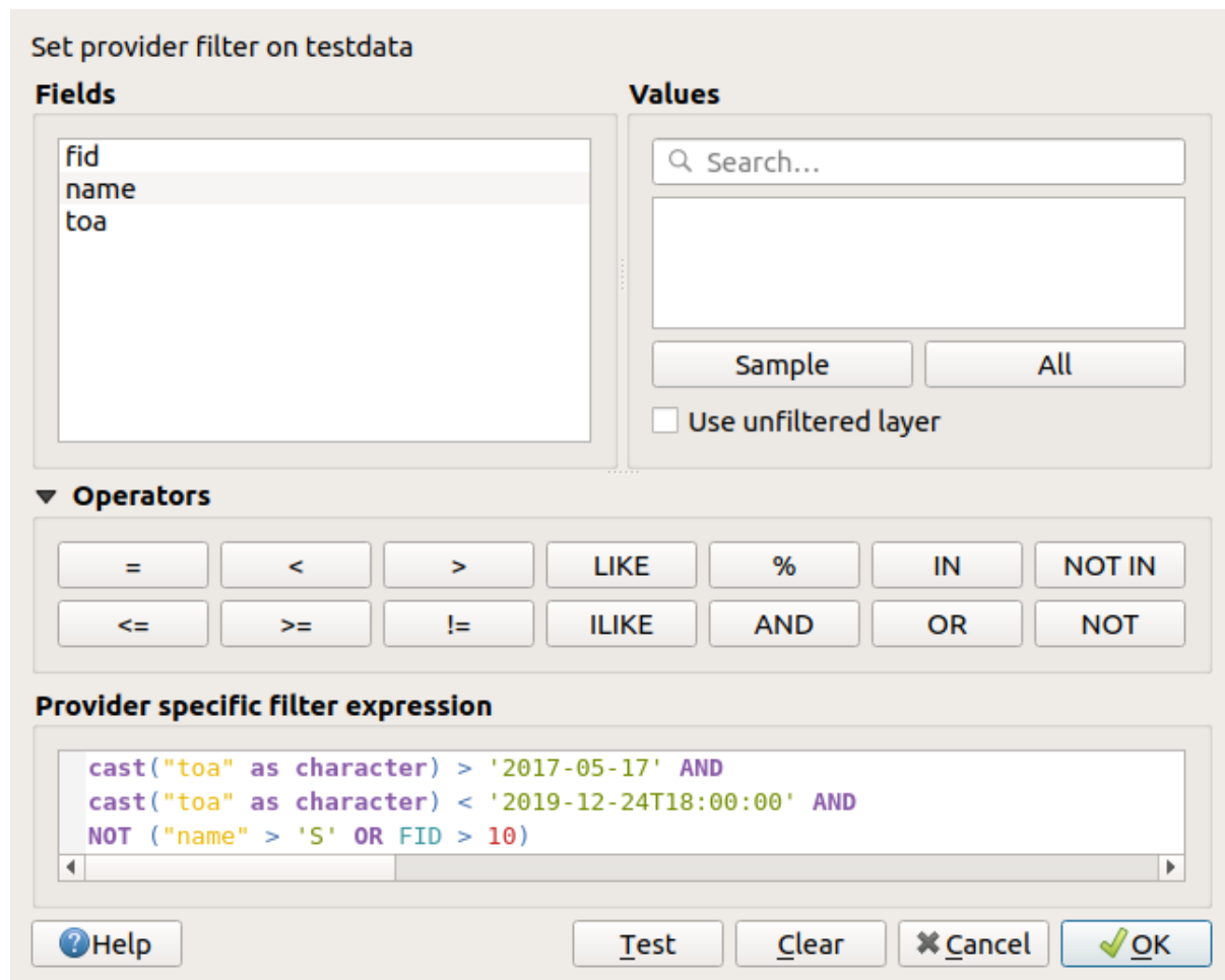
Gambar. 14.2: Query Builder
