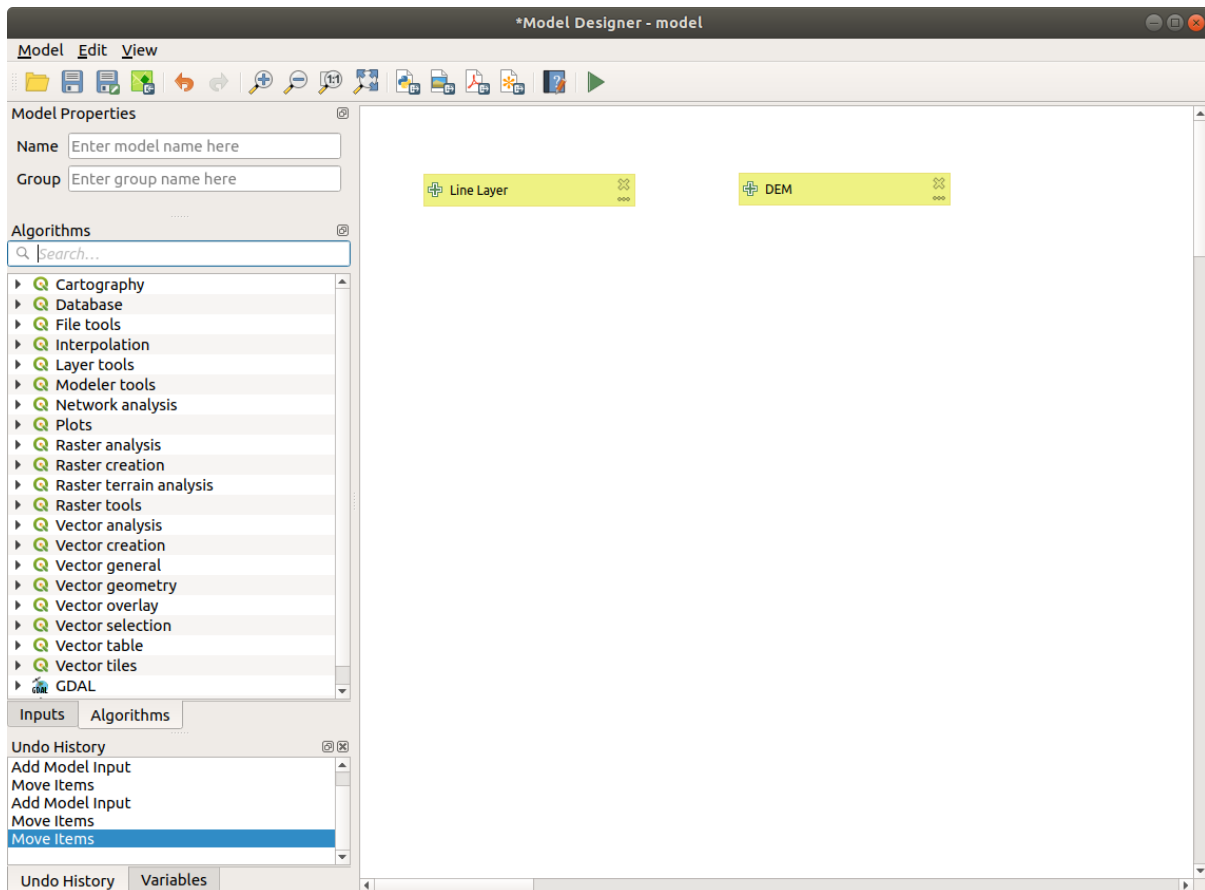
Gambar. 23.19: Model Inputs
