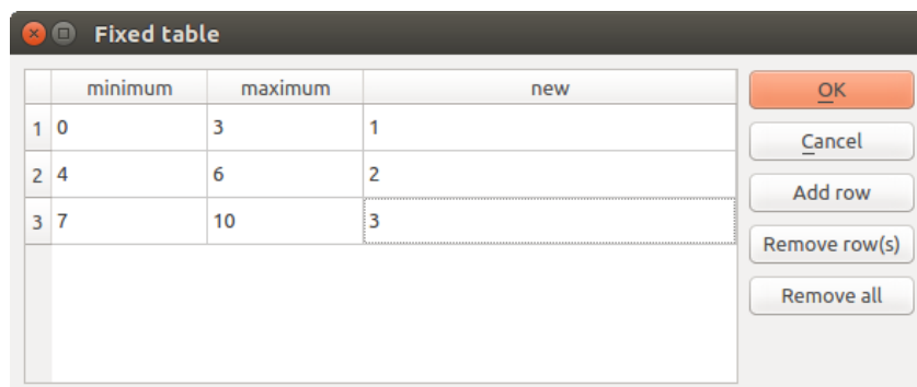
Gambar. 23.13: Fixed Table
