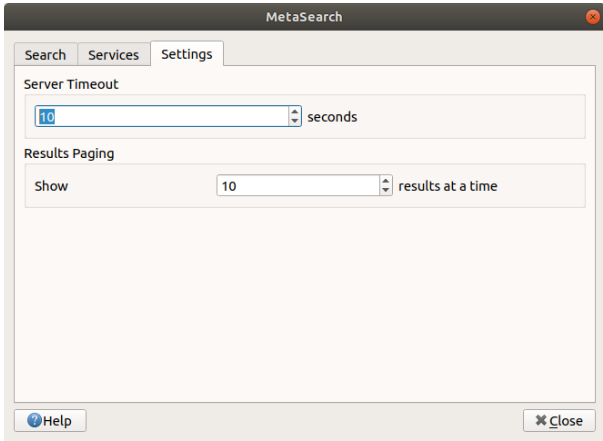
Gambar. 25.16: MetaSearch settings
