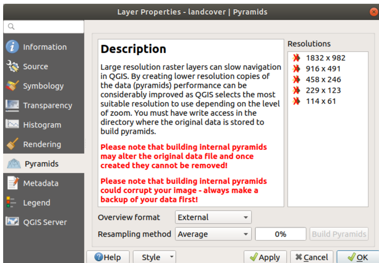
Gambar. 15.13: Raster Pyramids
