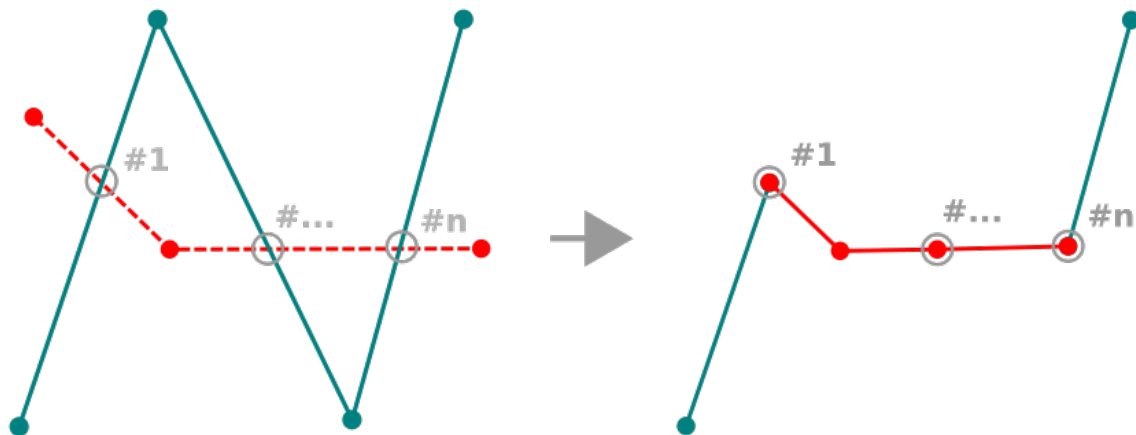
Gambar. 14.91: Reshape line
