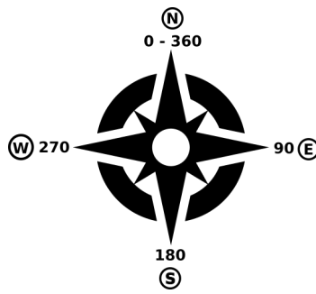
Gambar. 24.16: Aspect values
