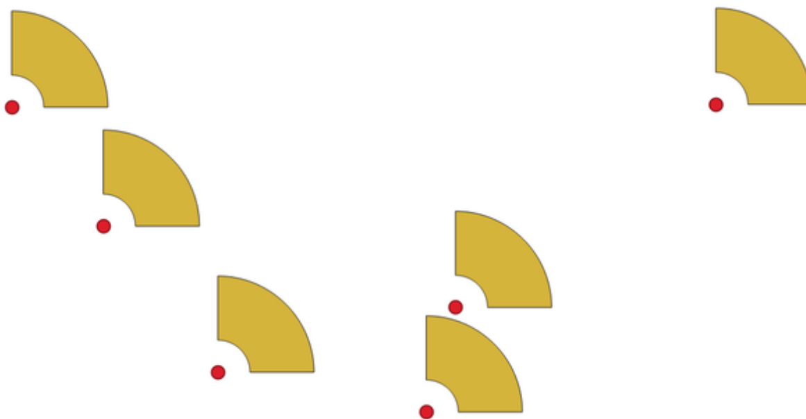
Fig. 24.51: Wedge buffers
