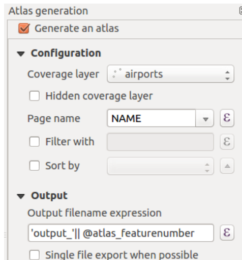
Obr. 18.62: Atlas Panel
