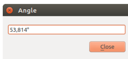
Obr. 11.19: Measure Angle
