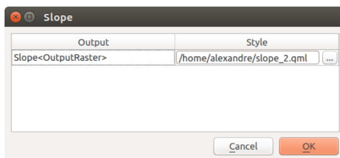
Obr. 23.5: Rendering Styles
