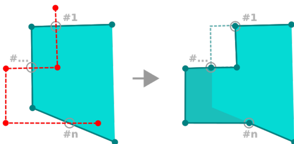
Obr. 14.92: Reshape polygon
