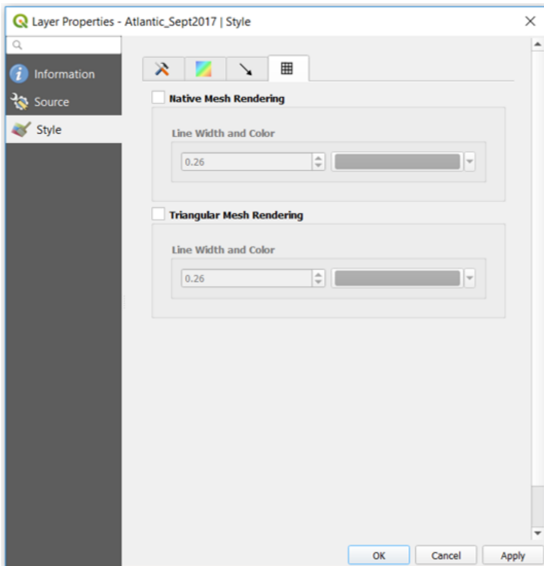
Obr. 16.9: Mesh Rendering
