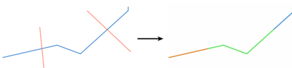
Obr. 24.96: Split lines
