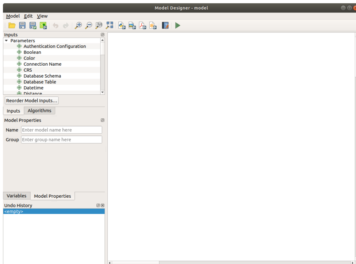
Obr. 23.16: Modelář
