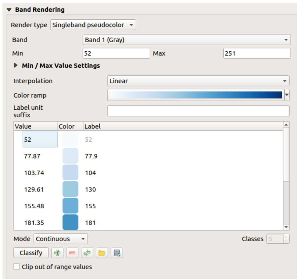
Obr. 15.5: Raster Symbology - Singleband pseudocolor rendering
