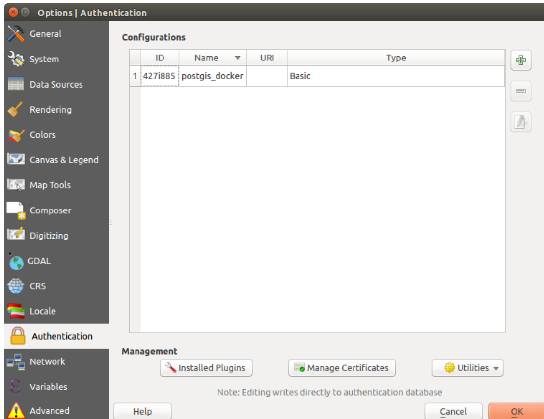
Obr. 21.5: Configurations editor
