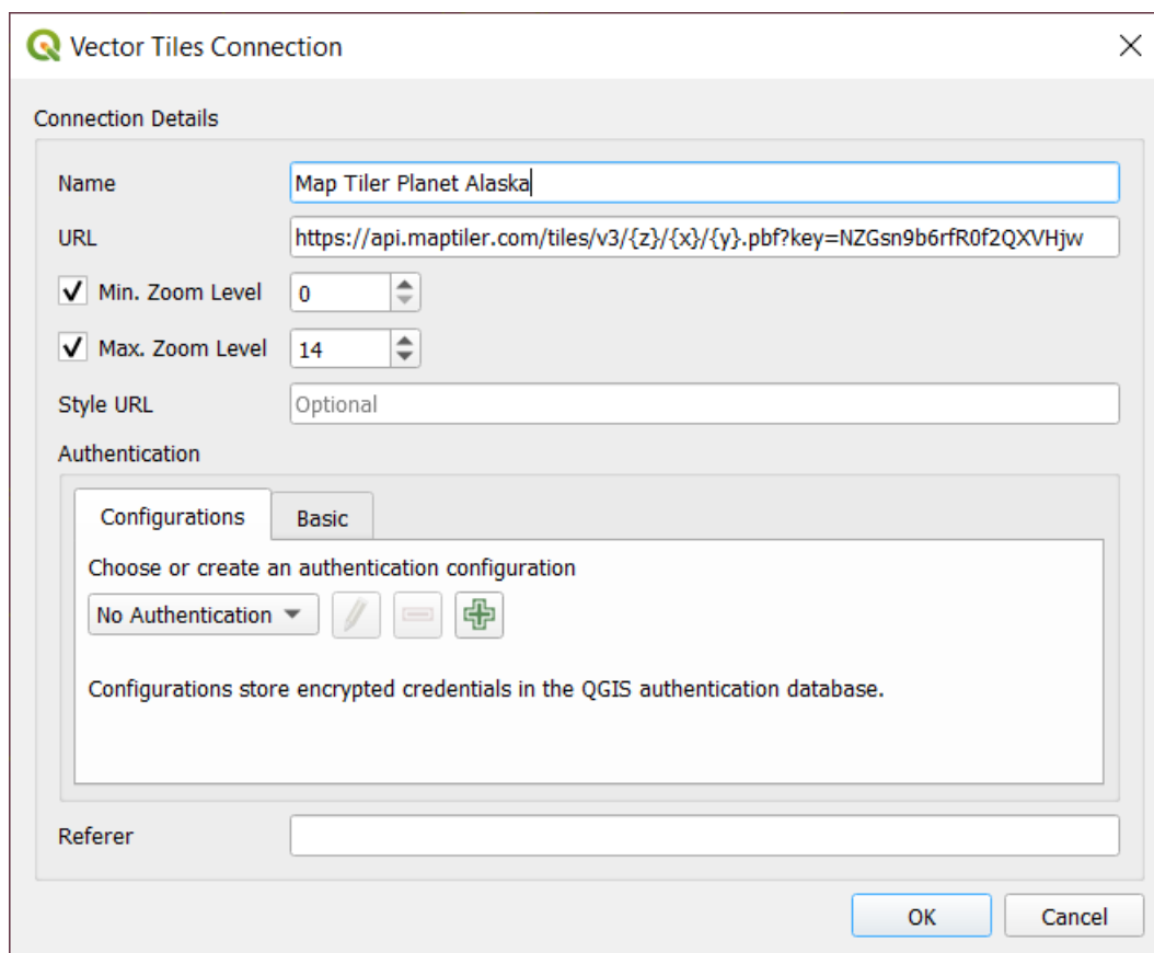
Obr. 13.13: Vector Tiles - Maptiler Planet configuration
