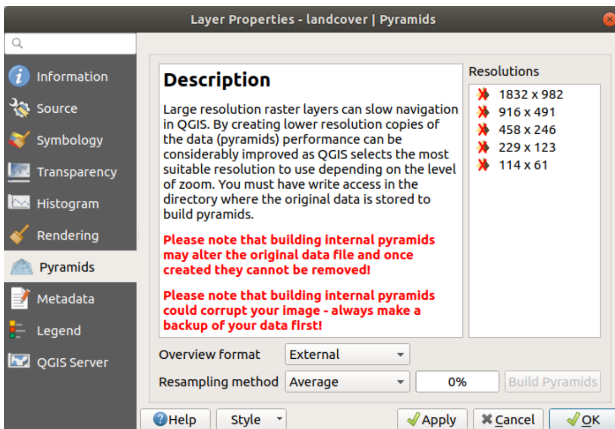
Obr. 15.13: Raster Pyramids
