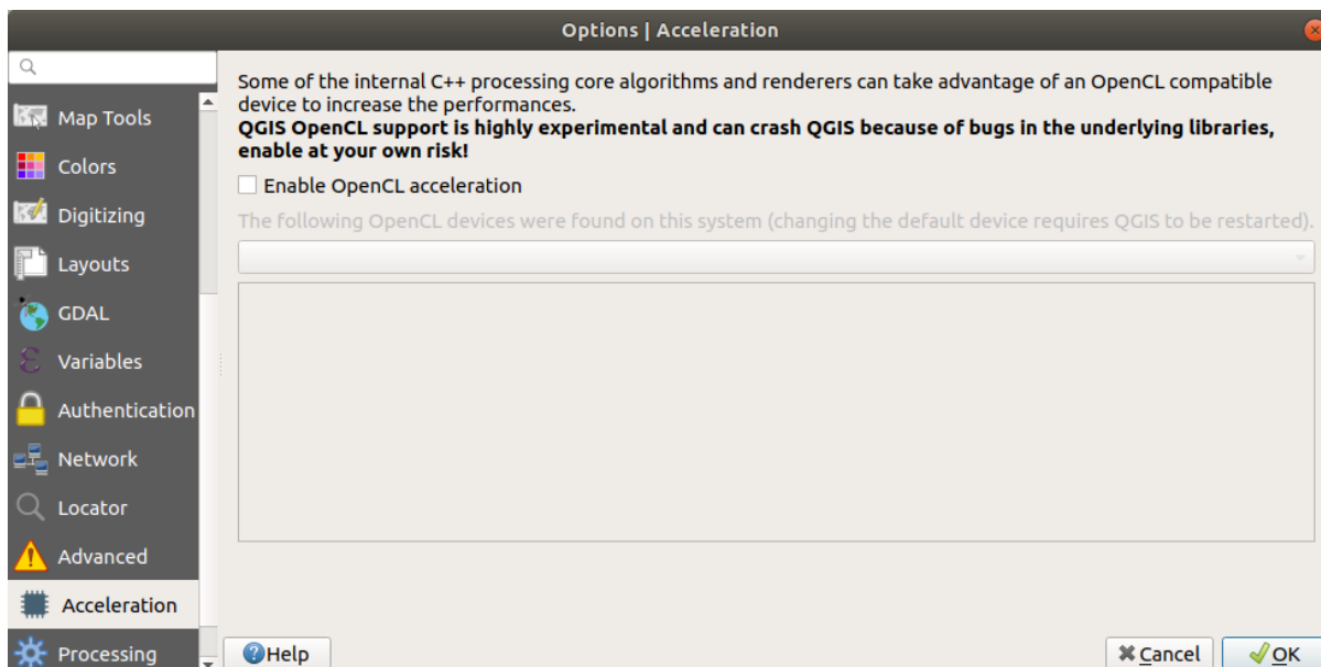
Obr. 9.19: Acceleration tab
