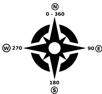
Obr. 24.16: Aspect values
