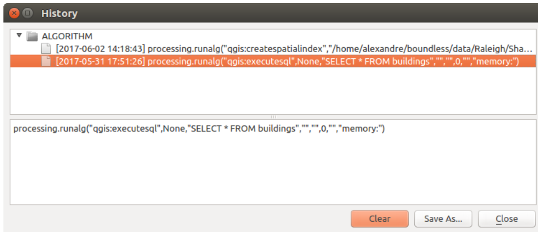
Obr. 23.3: Processing History
