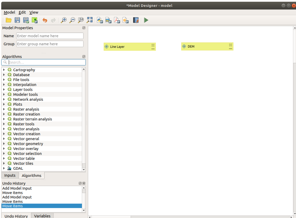
Obr. 23.19: Model Inputs
