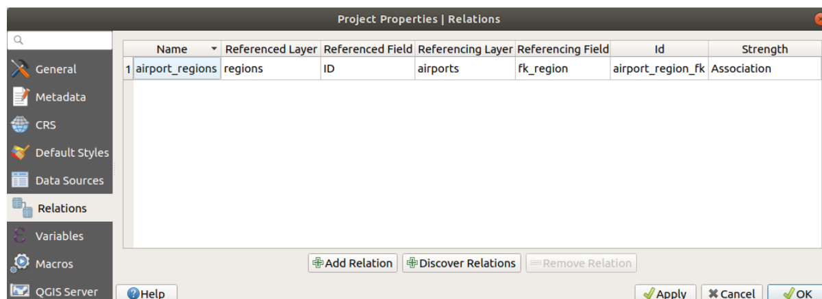
Obr. 9.26: Relations tab
