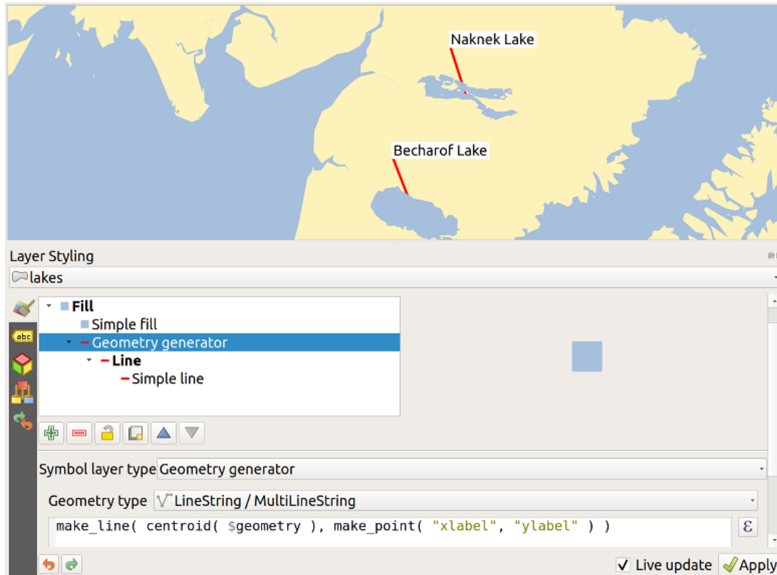
Obr. 14.34: Moved labels
