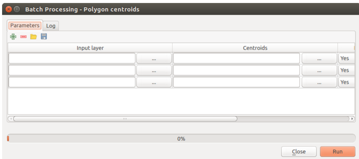
Obr. 23.31: Batch Processing
