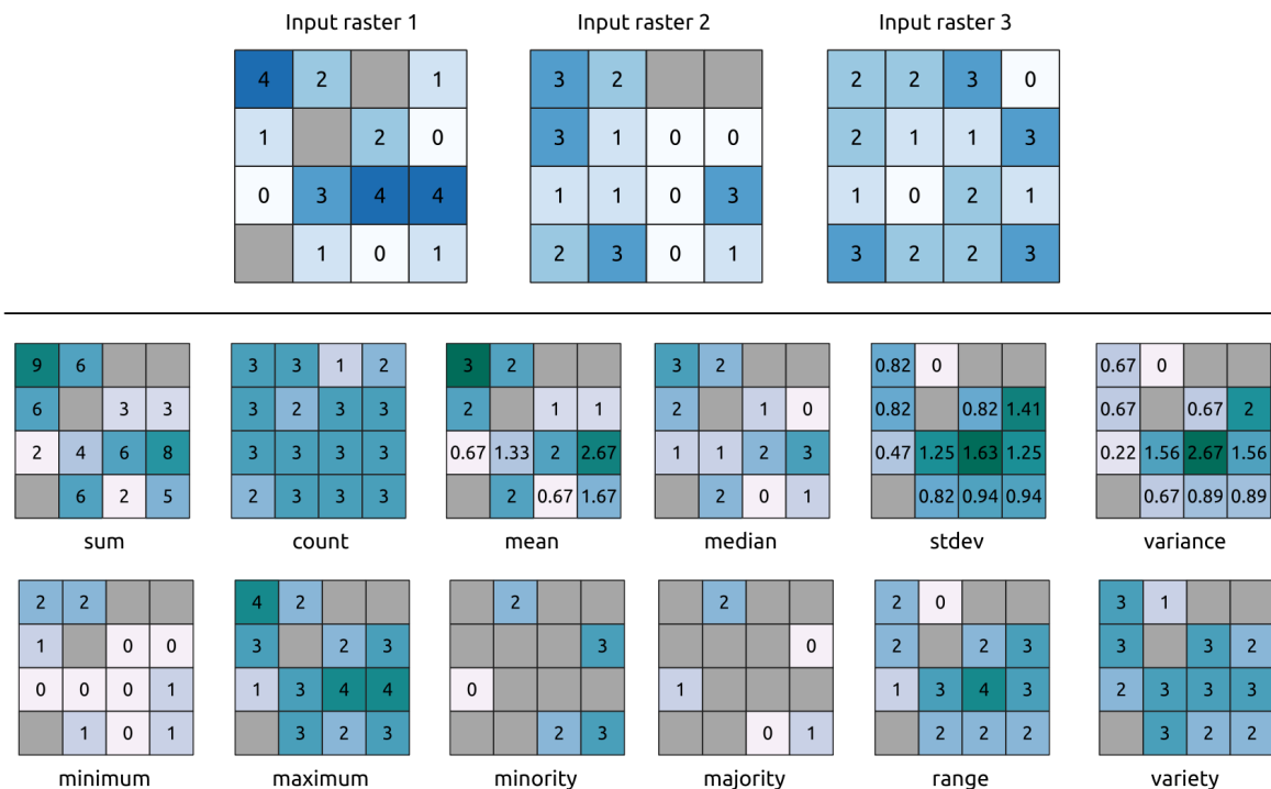
Fig. 24.8: Example with all the statistic functions. NoData cells (grey) are taken into account.
