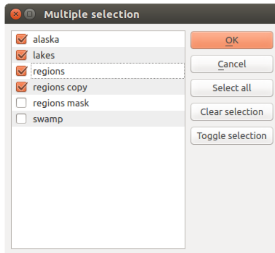
图 22.14: Multiple Selection
