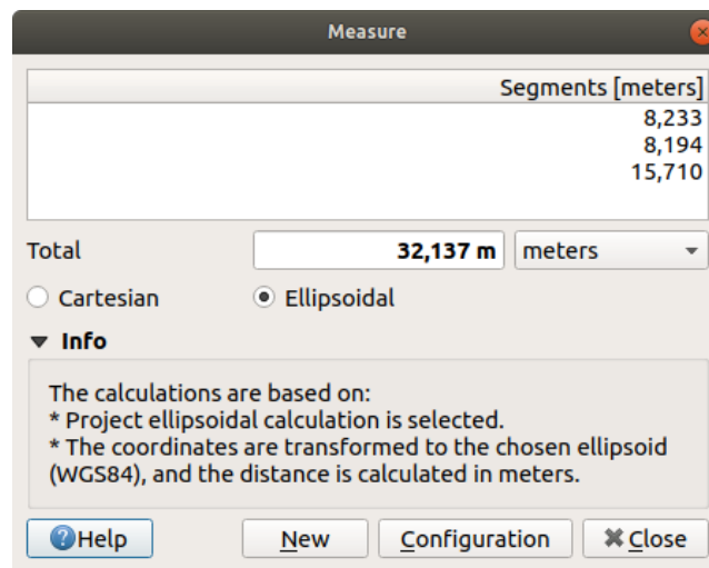
图 11.17: Measure Distance
