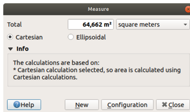
图 11.18: Measure Area
