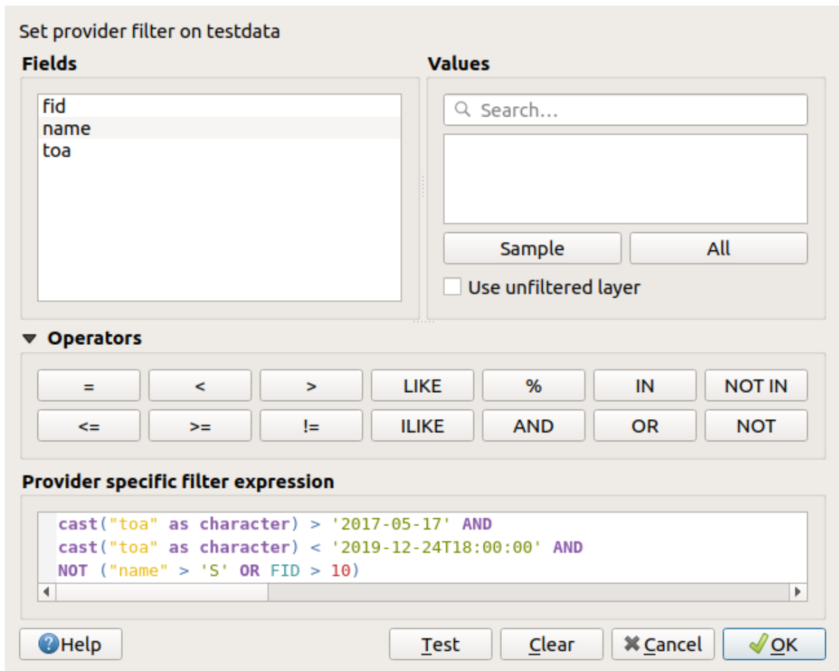
图 14.2: Query Builder
