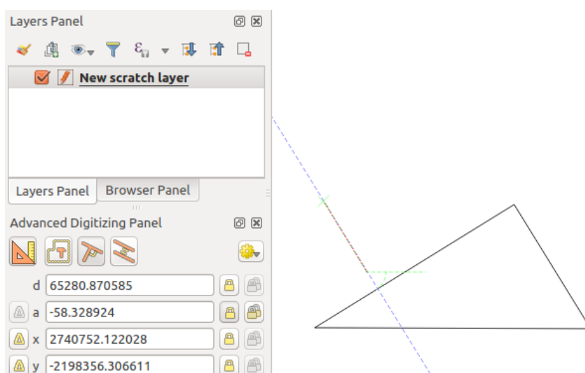
图 14.99: Perpendicular digitizing
