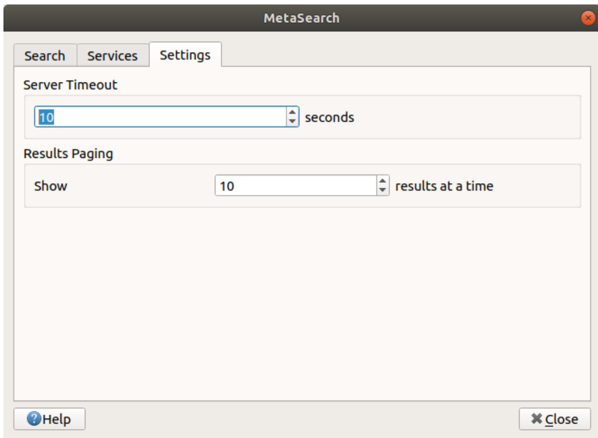
图 24.26: MetaSearch settings
