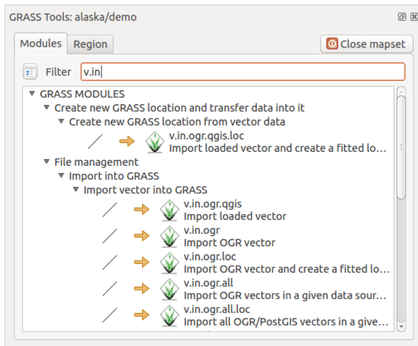
Şekil 21.3: GRASS Toolbox and Module Tree
