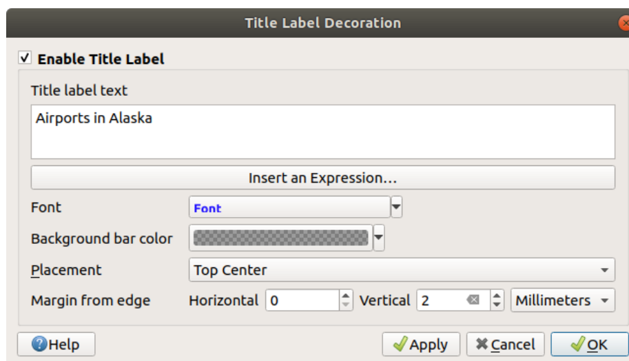
Şekil 11.8: The Title Decoration Dialog
