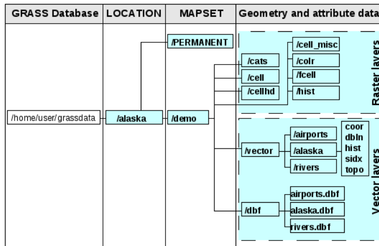
Şekil 21.1: GRASS data in the alaska LOCATION
