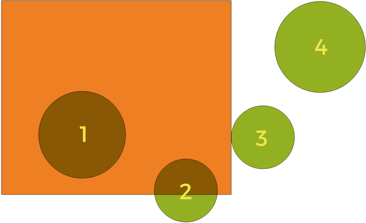
Şekil 23.87: In this example, the dataset from which we want to select (the source vector layer ) consists of the green circles, the orange rectangle is the dataset that it is being compared to (the intersection vector layer ).
