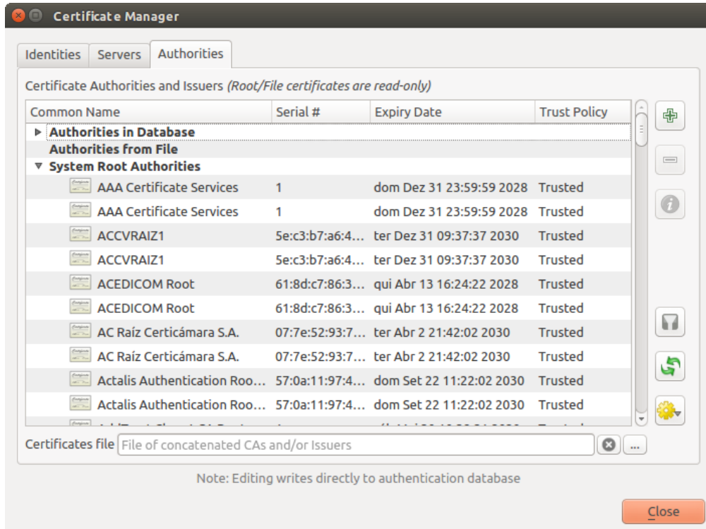
Şekil 20.24: Authorities editor
