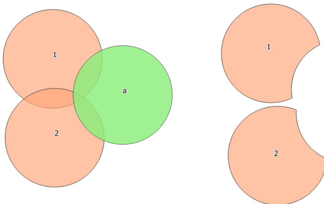
Şekil 23.79: Difference operation between a two-features input layer and a single feature overlay layer (left) - resulting features are moved for clarity (right)
