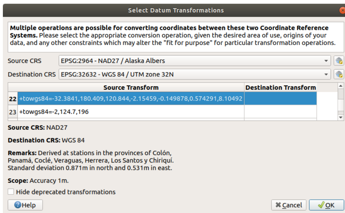
Şekil 10.5: Selecting a preferred default datum transformation
