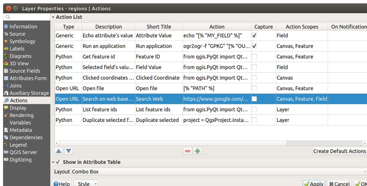
Şekil 14.56: Overview action dialog with some sample actions
