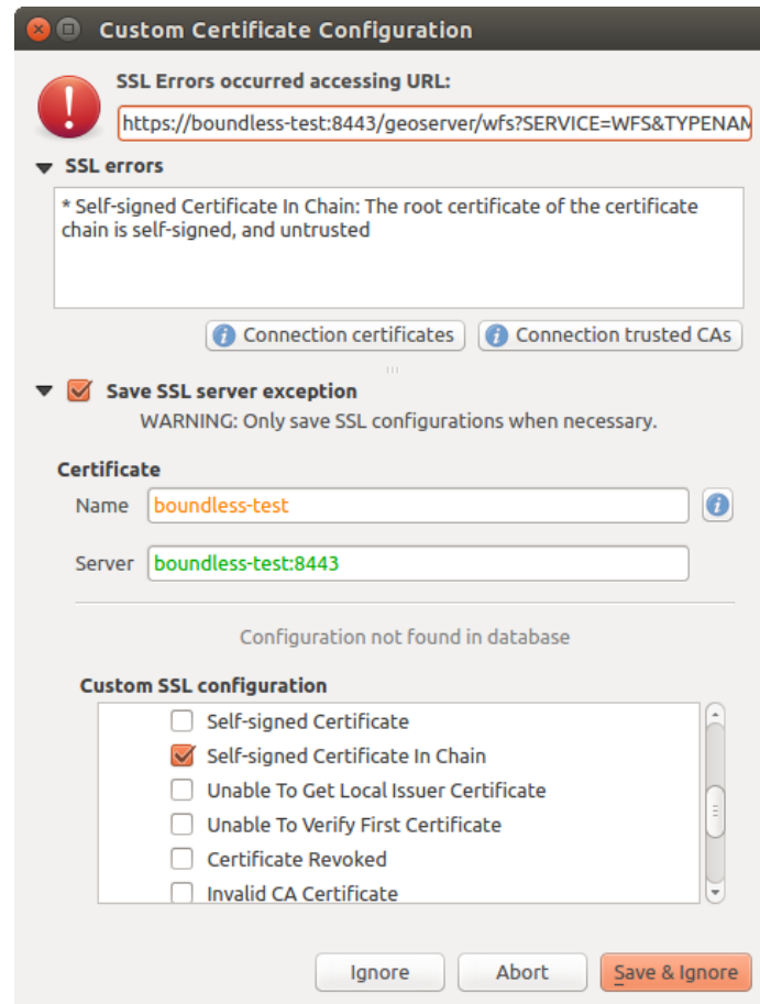
Şekil 20.37: Adding configuration during SSL error
