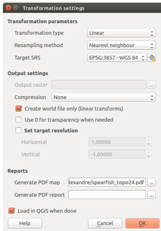
Şekil 24.21: Defining the georeferencer transformation settings
