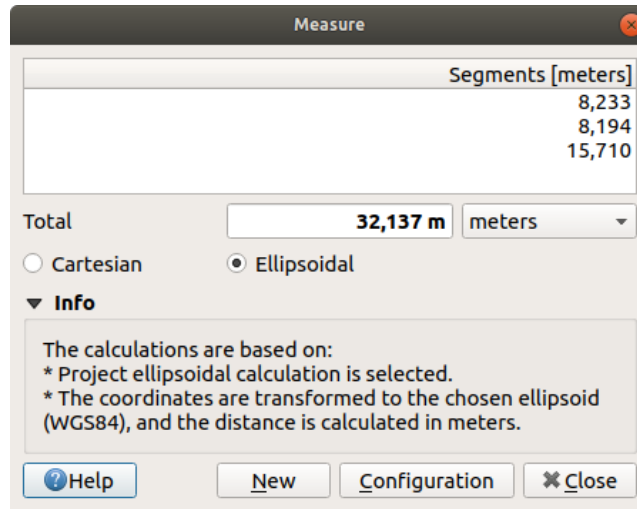
Şekil 11.17: Measure Distance
