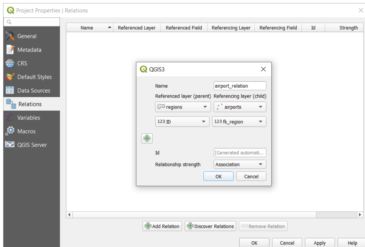
Şekil 14.77: Relation Manager
