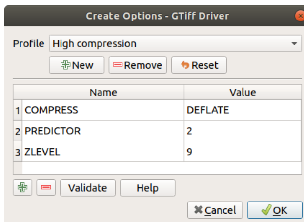
Şekil 9.10: Sample of create options profile (for GeoTiff)
