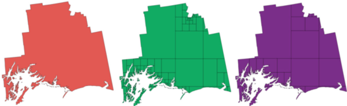
Gambar. 23.69: Left the input layer, middle maximum nodes value is 100 and right maximum value is 200
