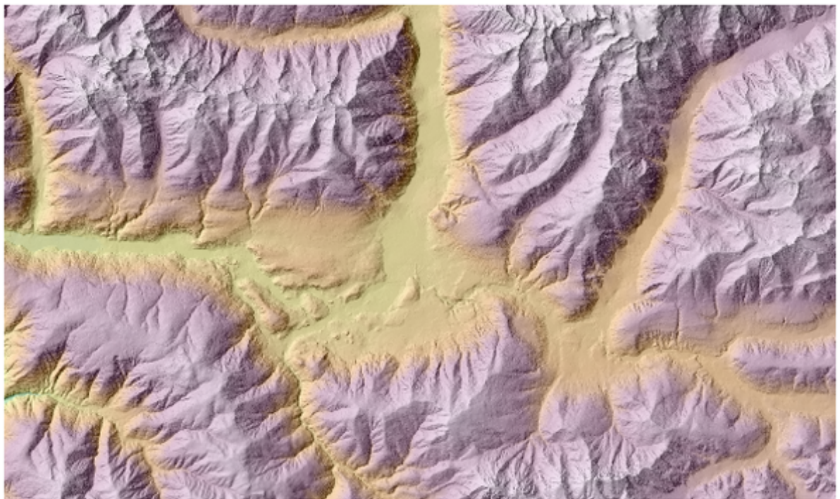
Gambar. 23.12: Overlapping the hillshade with the elevation layer
