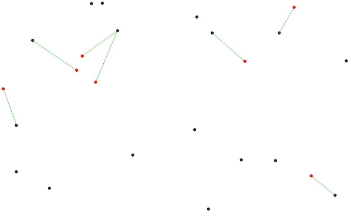
Gambar. 23.18: Display the nearest hub for the red input features
