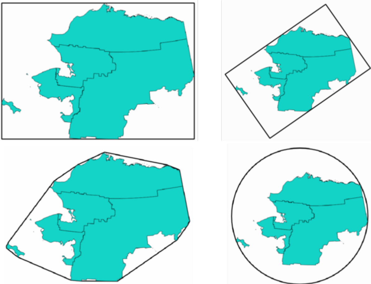
Gambar. 23.51: Clockwise from top left: envelope, oriented rectangle, circle, convex hull
