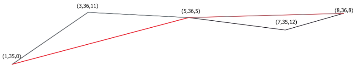
Gambar. 23.46: The red line represents the black line with only vertices whose M value is \leq 10 .
