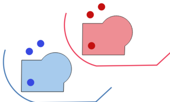
Gambar. 23.73: Dashed lines represent the translated geometry of the input layer
