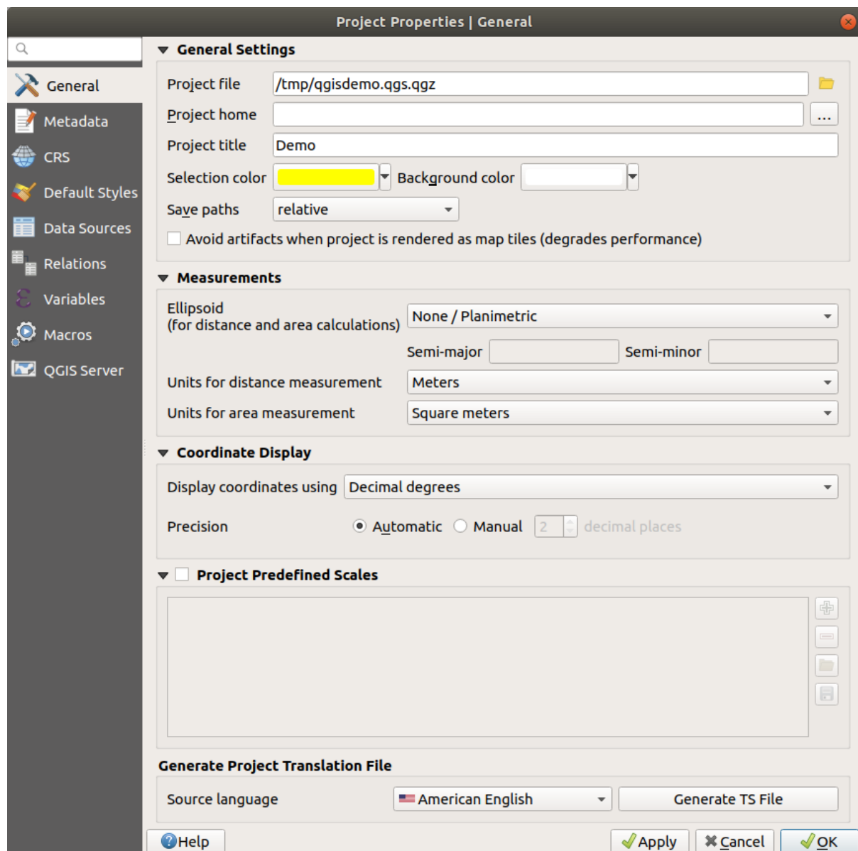
Gambar. 9.20: General tab of the Project Properties dialog
