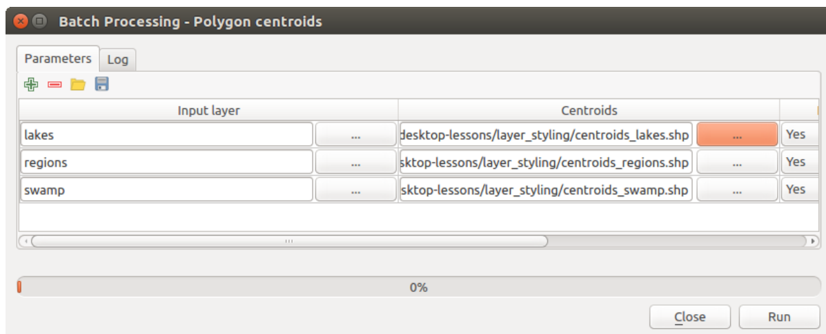
Gambar. 22.32: Batch Processing File Path
