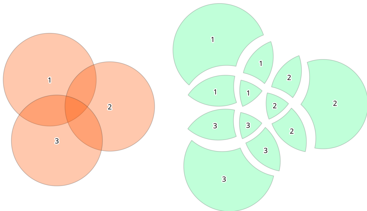
Gambar. 23.84: Union operation with a single input layer of three overlapping features (left) - resulting features are moved for clarity (right)
