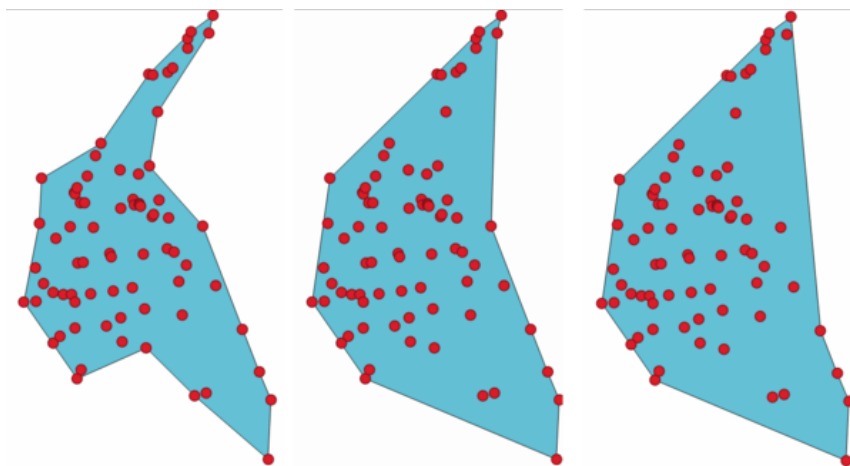
Gambar. 23.34: Concave hulls with different thresholds (0.3, 0.6, 0.9)
