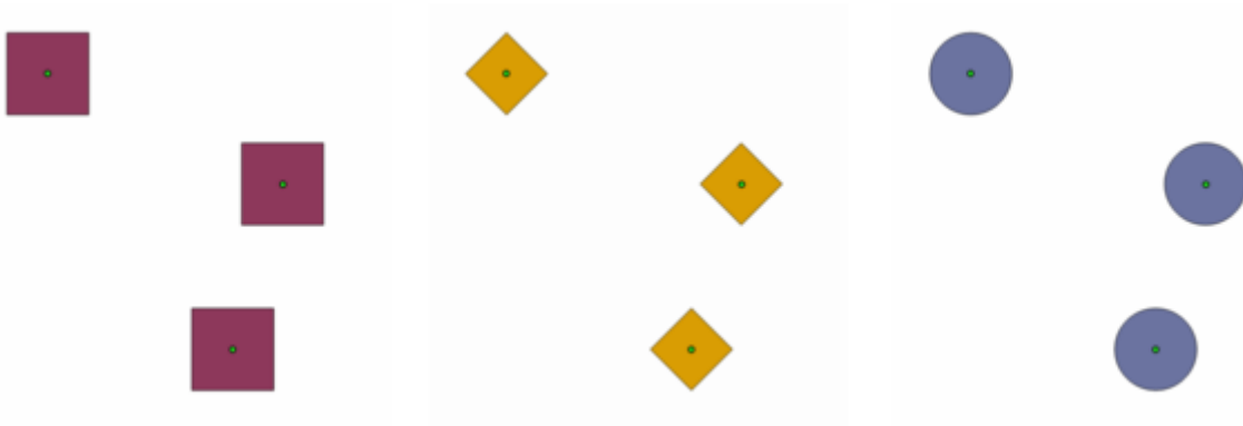
Gambar. 23.62: Different buffer shapes
