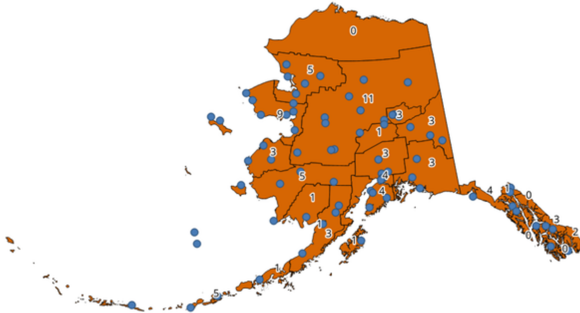
Gambar. 23.17: The labels in the polygons show the point count
