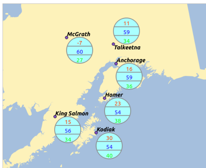
Gambar. 14.39: Diagram from temperature data overlaid on a map
