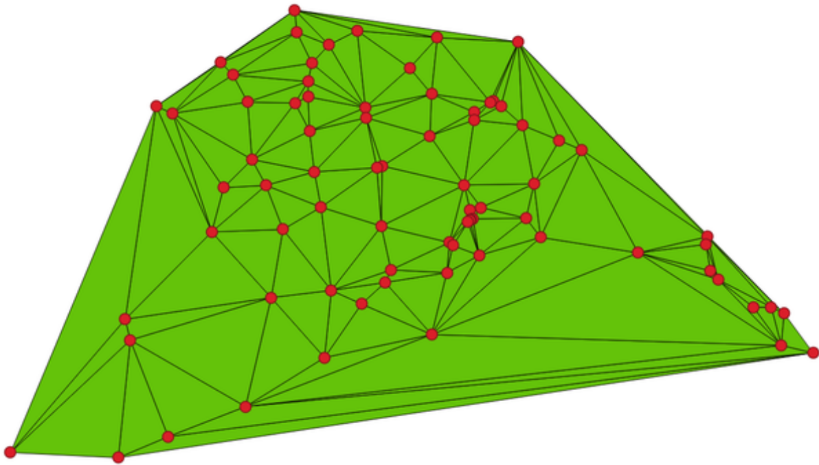
Gambar. 23.38: Delaunay triangulation on points
