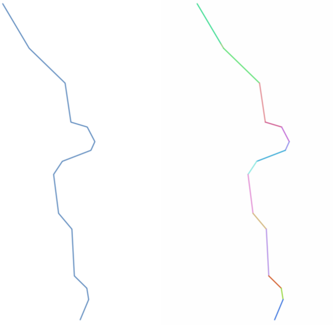
Gambar. 23.43: The original line layer and the exploded one
