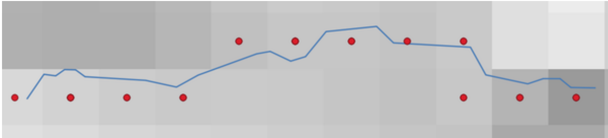
Gambar. 23.24: Points of the pixel centroids
