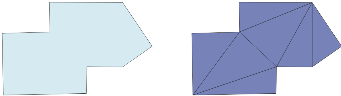
Gambar. 23.71: Tessellated polygon (right)
