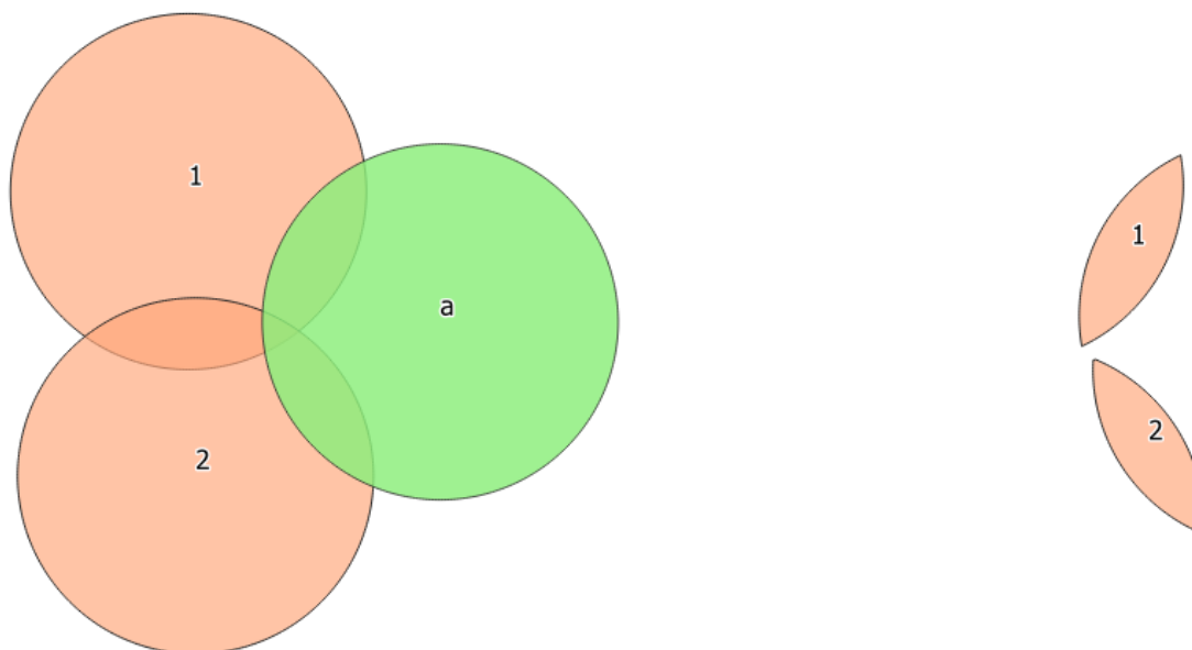
Gambar. 23.78: Clipping operation between a two-features input layer and a single feature overlay layer (left) - resulting features are moved for clarity (right)
