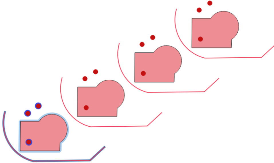
Gambar. 23.22: Input layers in blue tones, output layers with translated features in red tones
