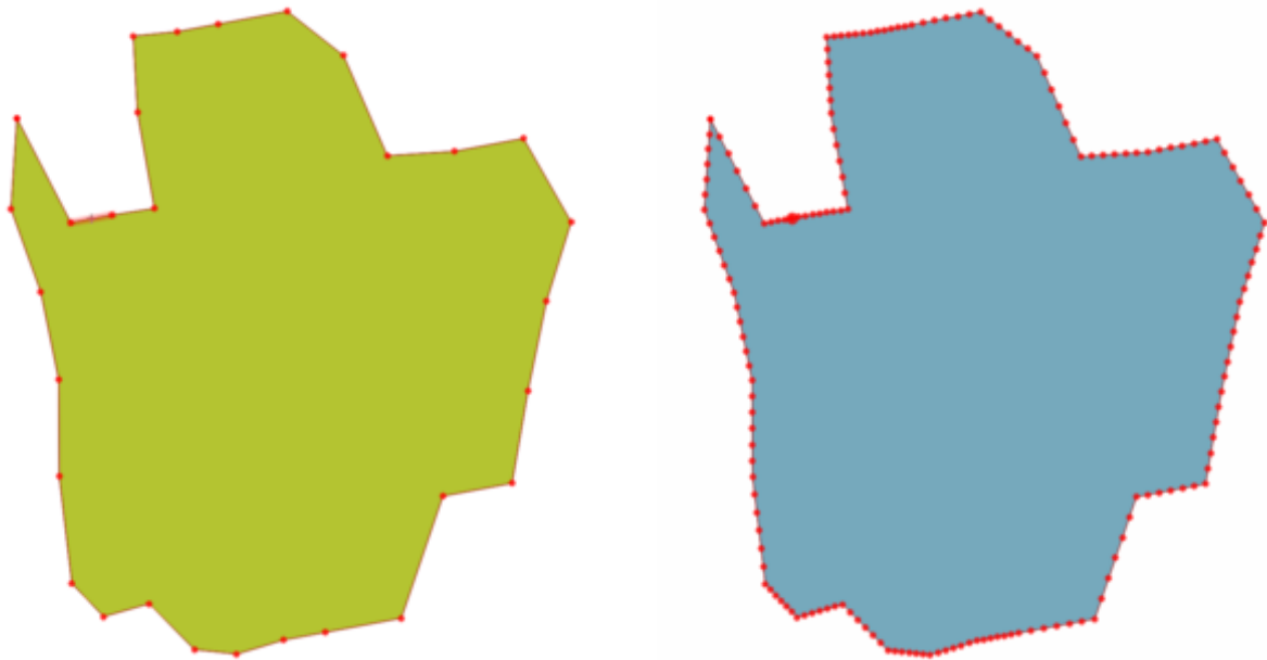
Gambar. 23.40: Red points show the vertices before and after the densify
