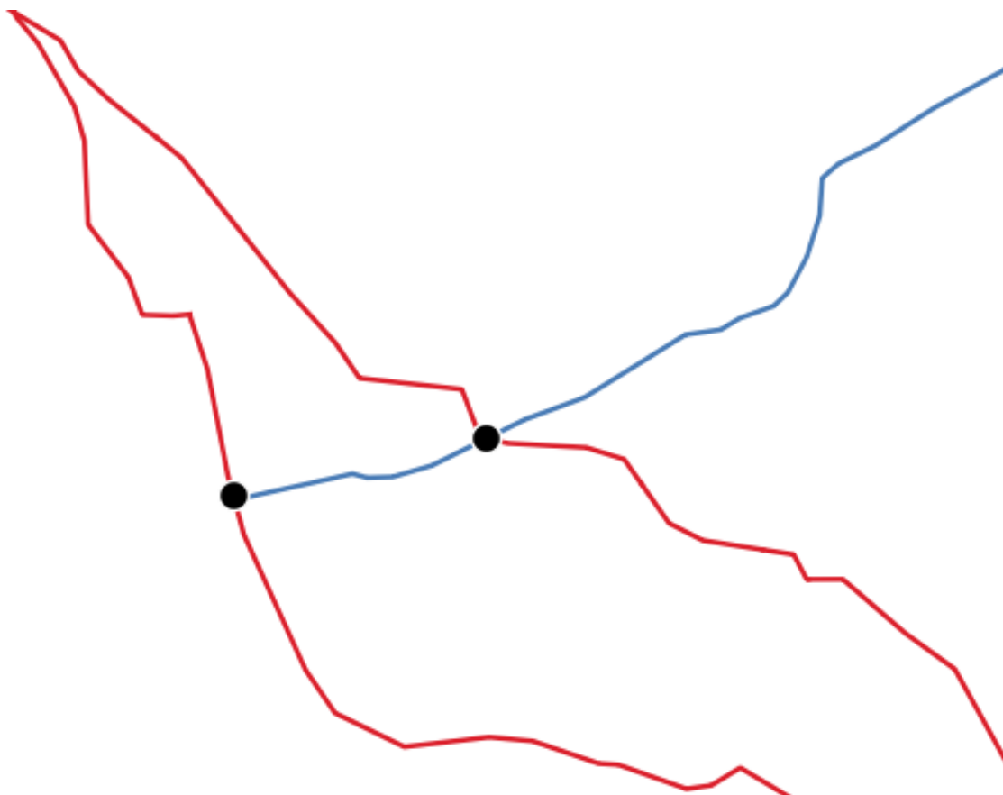
Gambar. 23.81: Points of intersection
