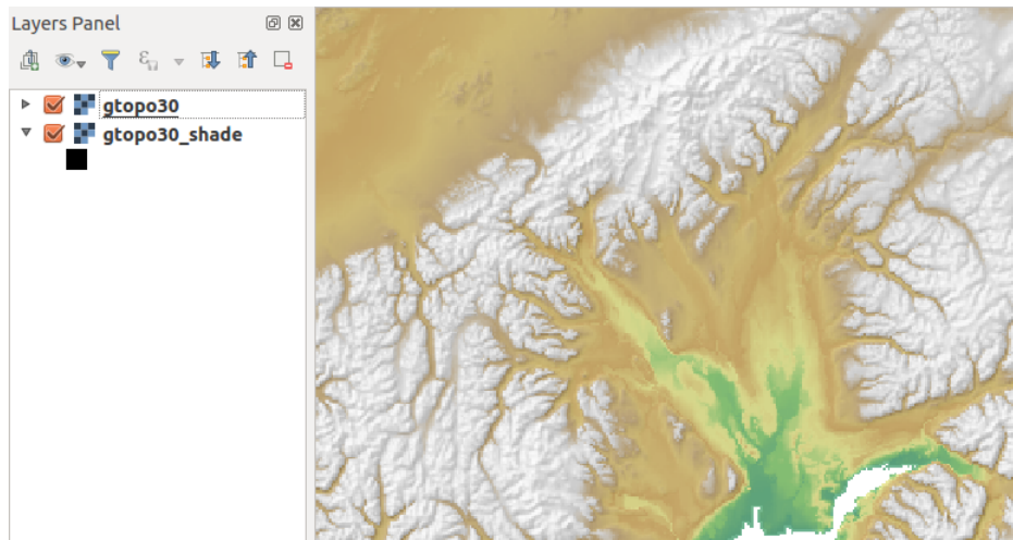
Gambar. 21.9: Displaying shaded relief created with the GRASS module r.shaded.relief
