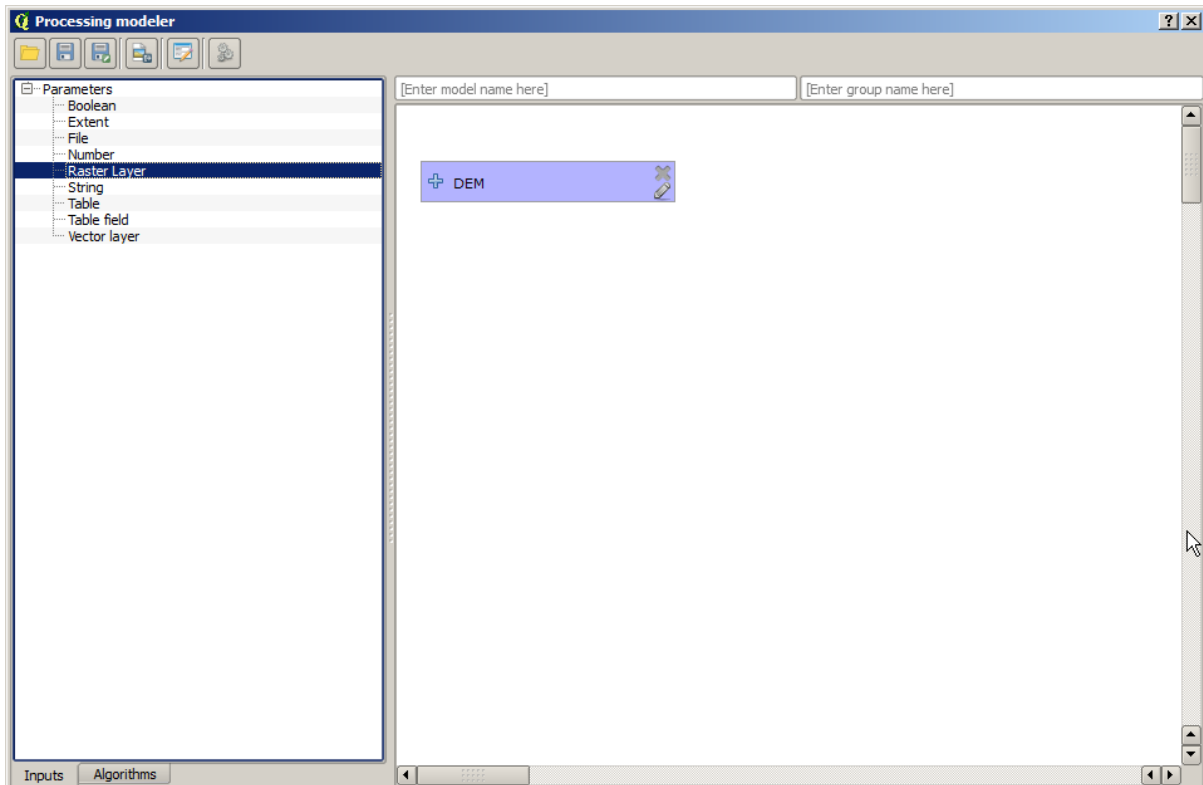
Figure 17.19: Model Parameters
