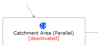
Figure 17.23: Deactivate
