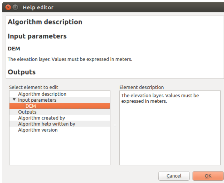
Figure 20.26: Help Edition
