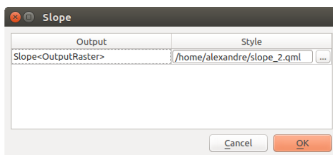
Figure 20.16: Rendering Styles
