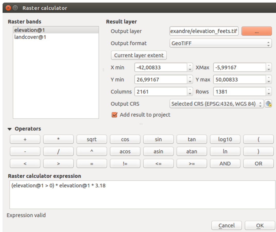
Figure 13.10: Calculadora Raster
