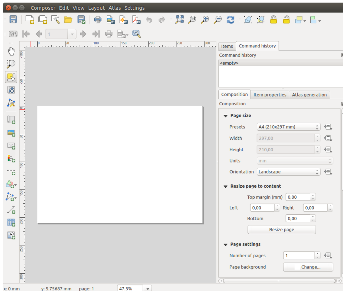
Figure 14.2: Print Composer
