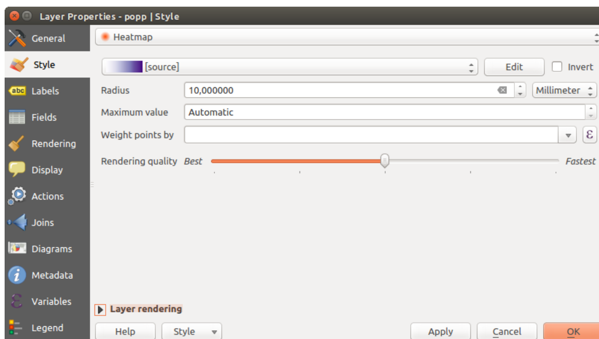
Figure 12.17: Heatmap dialog
