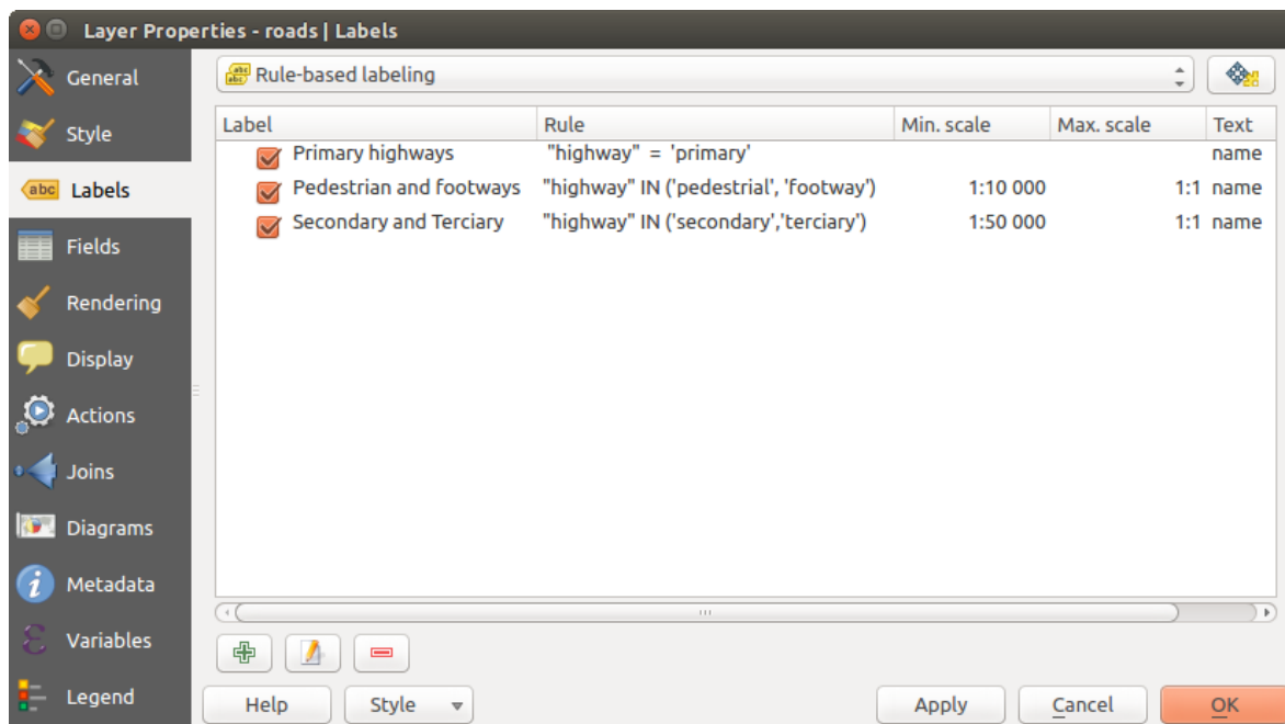
Gambar 12.34: Rule based labeling panel
