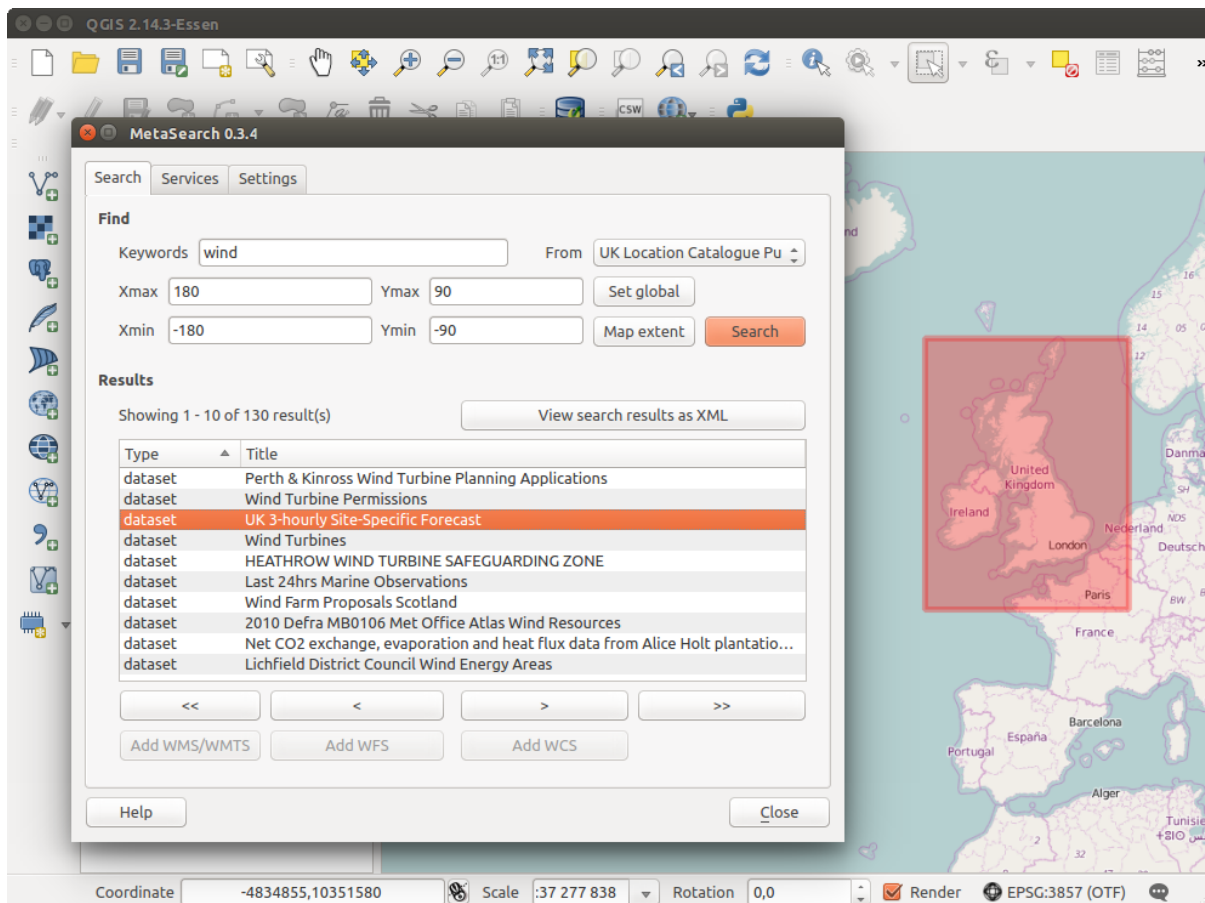
Gambar 21.31: Search and results of Services in Metasearch
