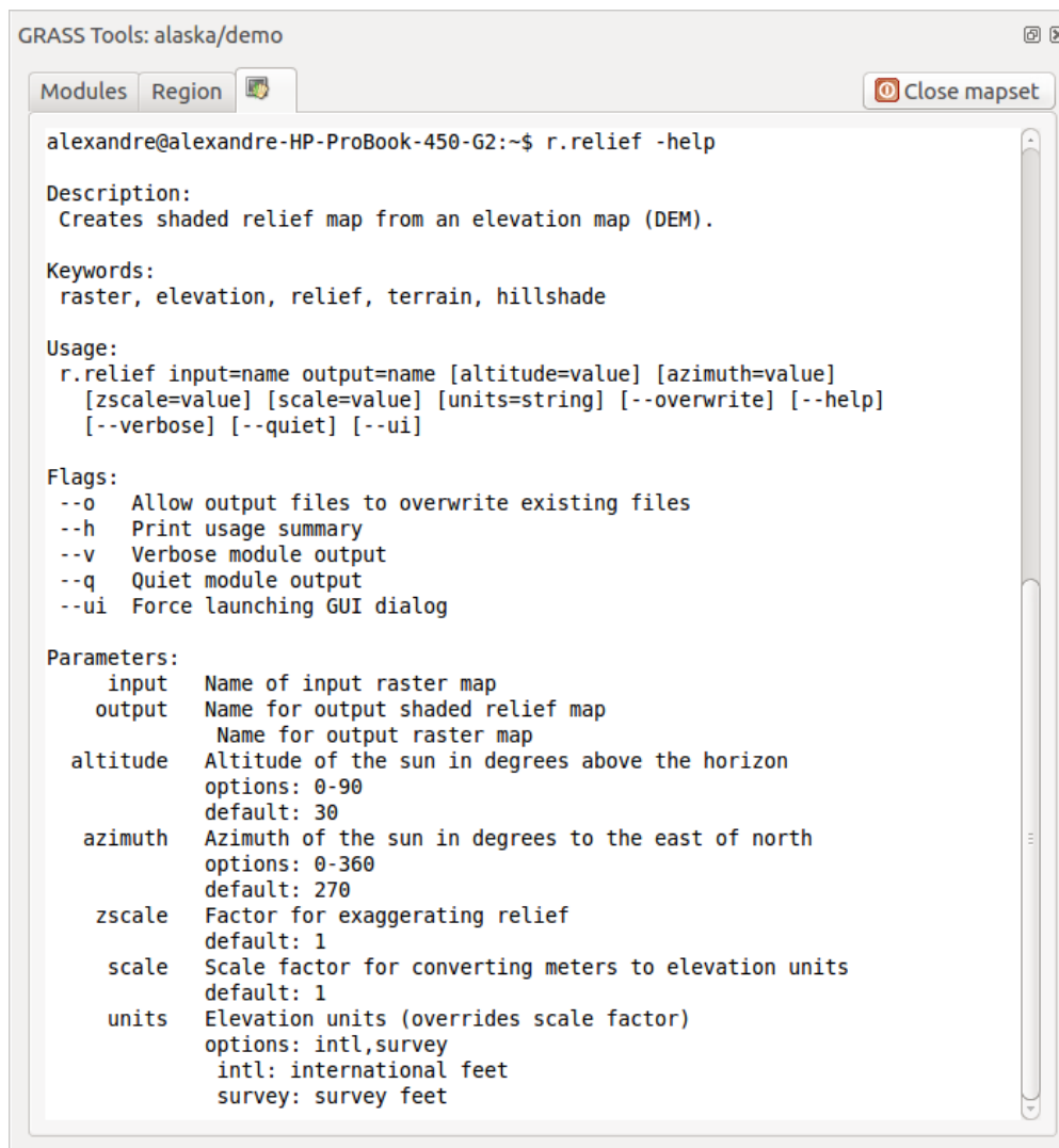
Gambar 18.8: The GRASS shell, r.shaded.relief module
