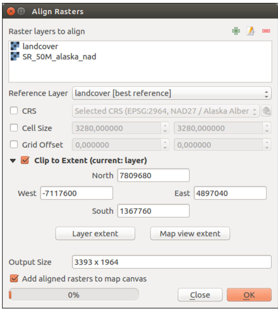
Figure 13.12: Raster Alignment
