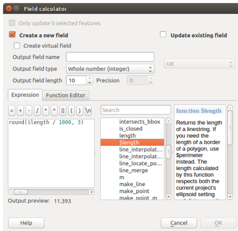
Figure 12.63: Field Calculator
