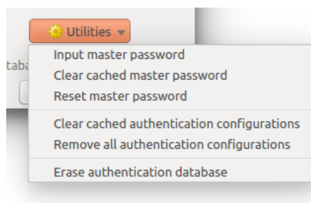
Figure 17.13: Utilities menu
