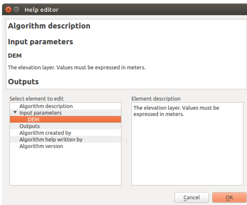
Figure 20.26: Help Edition
