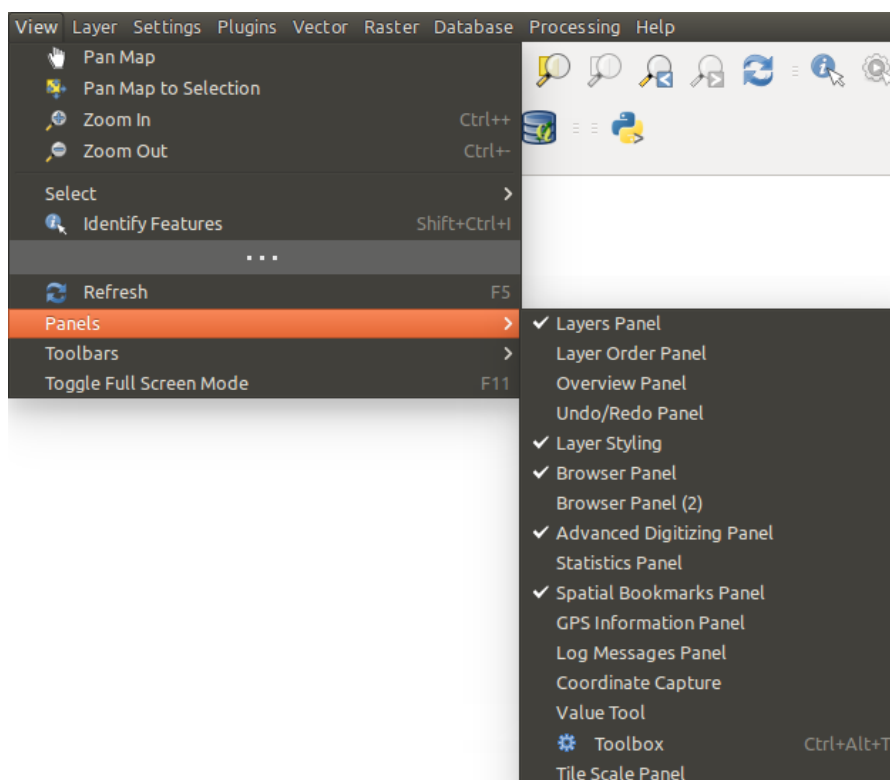
Figure 7.3: Panelové menu
