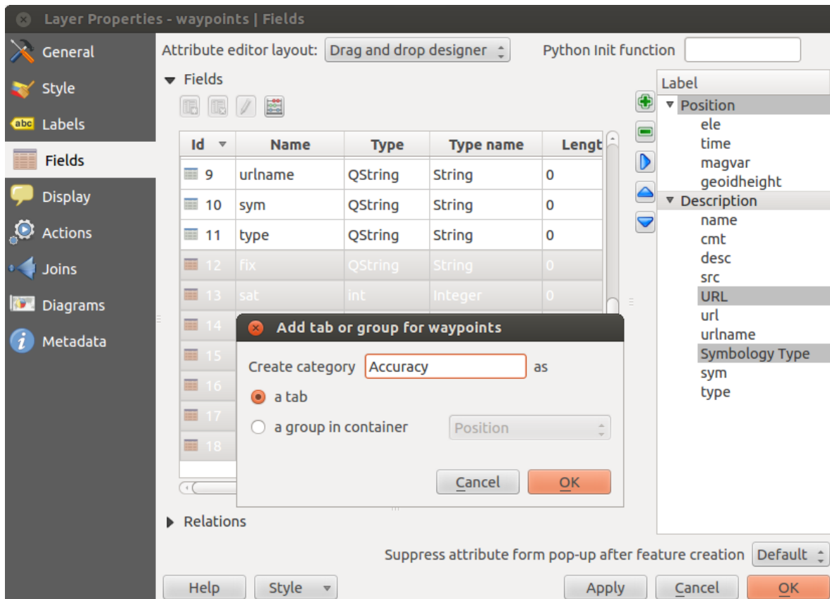
Figure 12.44: Dialog to create categories with the Attribute editor layout
