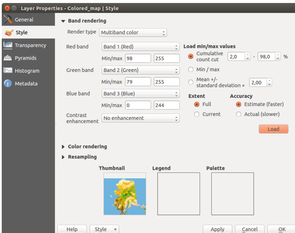
Figure 13.2: Raster Renderer - Multiband color
