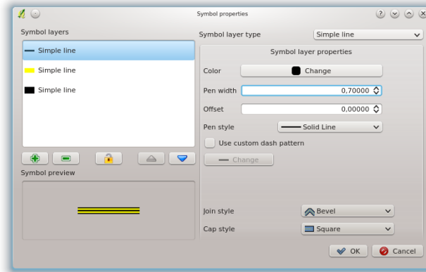
Kuva 11.13: Line composed from three simple lines 🐧
