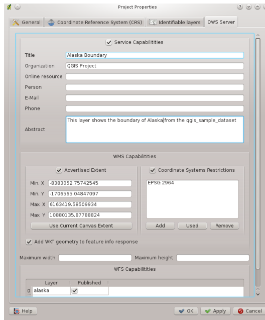
Figura 13.5: Definitions for a qgis project WMS/WFS server (KDE)
