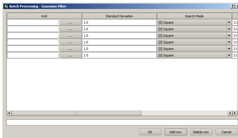
Figur 17.25: Batch Processing
