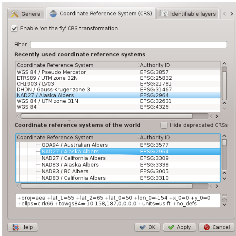
Figur 9.2: Projection Dialog
