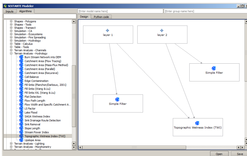
Figur 17.2: SEXTANTE Models
