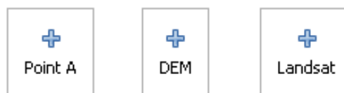
Figur 17.16: Model Parameters
