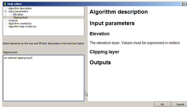
Figur 17.23: Help Edition
