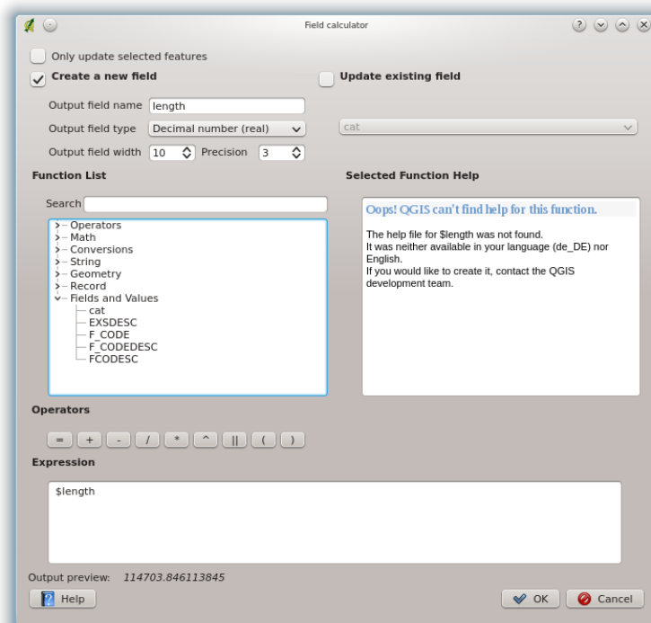
Figur 11.35: Field Calculator 🐧
